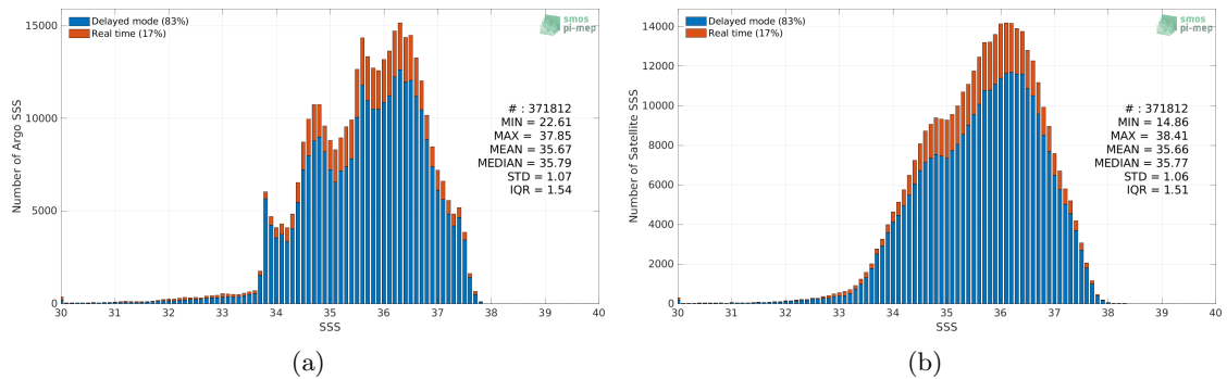
Figure 2: Histograms of SSS from Argo (a) and SMOS SSS L3 v8 - 9 Days (CATDS-CECOS-LOCEAN) (b) considering all match-up pairs per bins of 0.1 over the Atlantic Ocean Pi-MEP region and for the full satellite product period.
