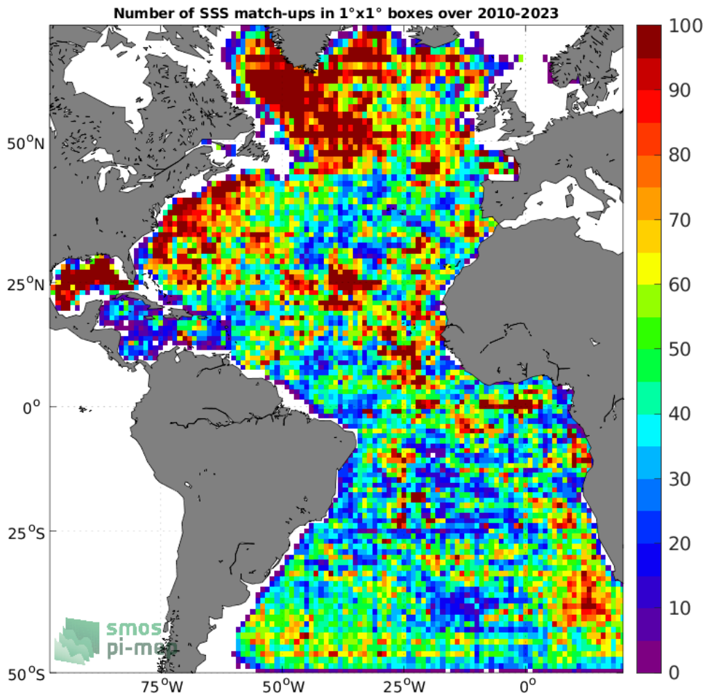
Figure 4: Number of SSS match-ups between Argo SSS and the SMOS SSS L3 v8 - 9 Days (CATDS-CECOS-LOCEAN) SSS product for the Atlantic Ocean Pi-MEP region over 1^{\circ} \times 1^{\circ} boxes and for the full satellite product period.
