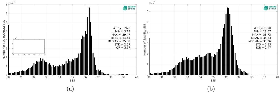
Figure 2: Histograms of SSS from TSG (SAMOS) (a) and SMOS SSS L3 v8 - 18 Days (CATDS-CEC-LOCEAN) (b) considering all match-up pairs per bins of 0.1 over the Atlantic Ocean Pi-MEP region and for the full satellite product period.
