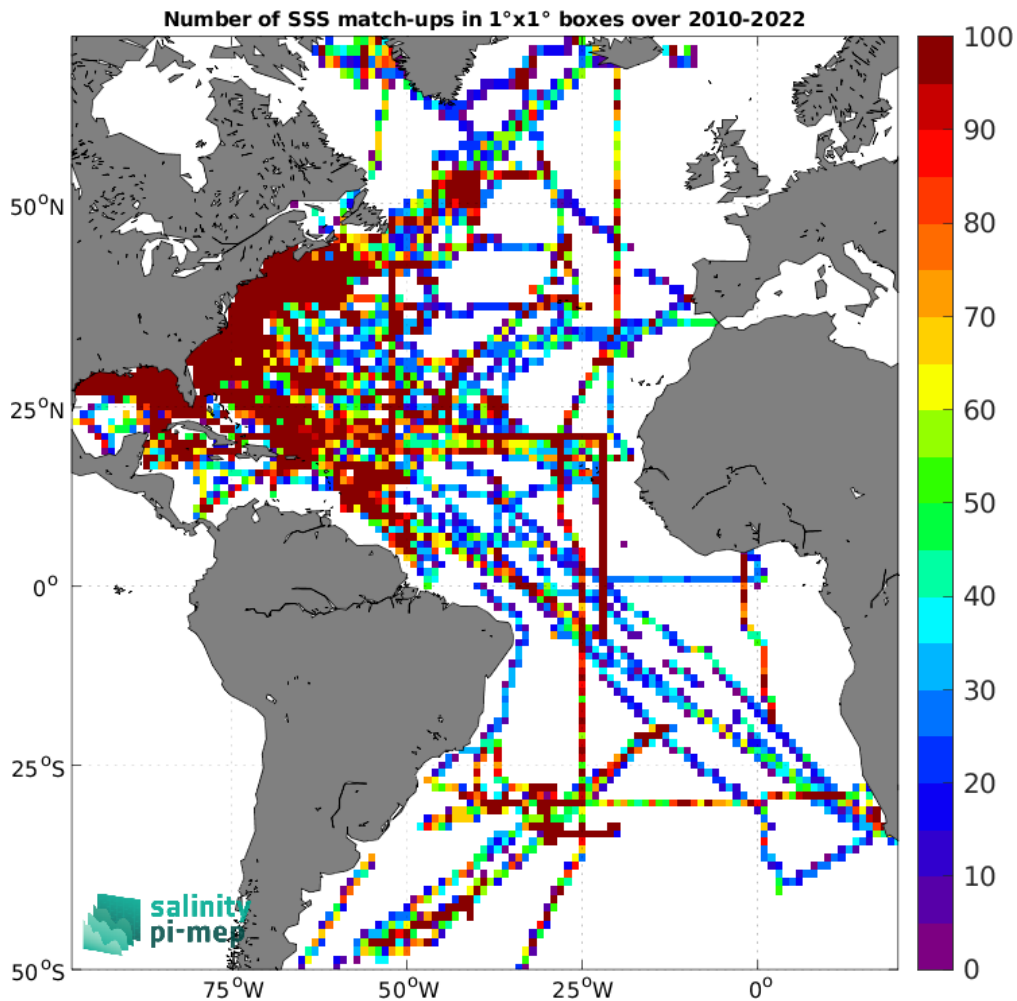
Figure 4: Number of SSS match-ups between TSG (SAMOS) SSS and the SMOS SSS L3 v8 - 18 Days (CATDS-CEC-LOCEAN) SSS product for the Atlantic Ocean Pi-MEP region over 1^\circ \times 1^\circ boxes and for the full satellite product period.
