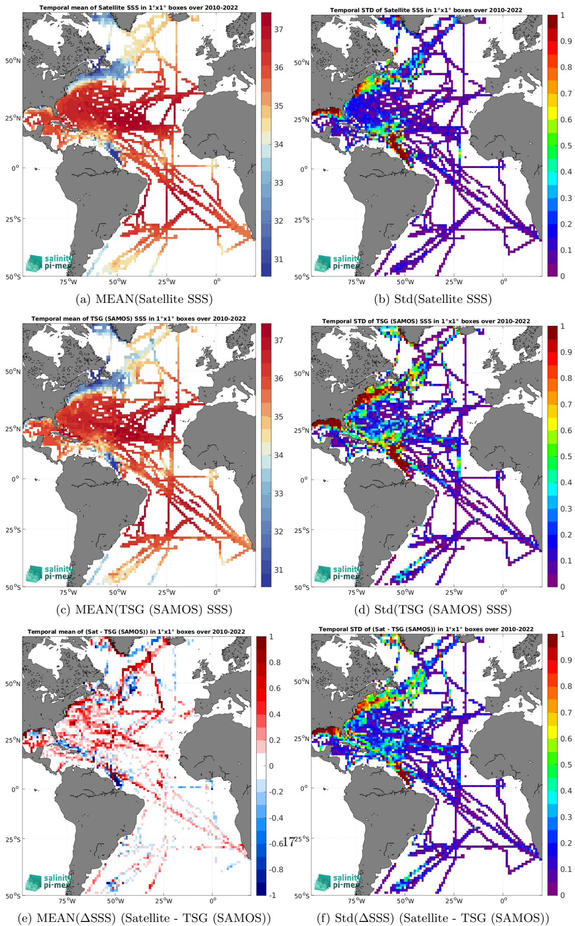
Figure 6: Temporal mean (left) and Std (right) of SSS from SMOS SSS L3 v8 - 18 Days (CATDS-CEC-LOCEAN) (top), TSG (SAMOS) (middle), and of \Delta SSS (Satellite - TSG (SAMOS)). Only match-up pairs are used to generate these maps.
