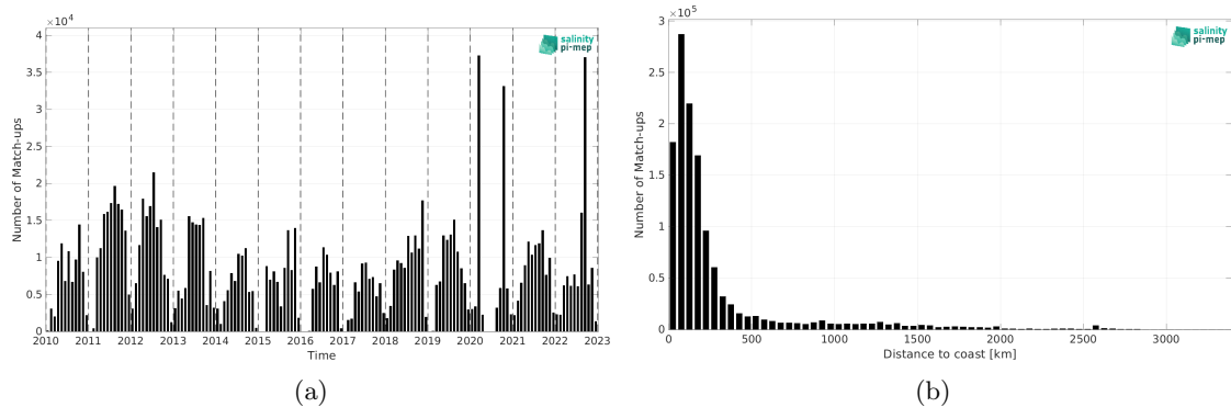
Figure 1: Number of match-ups between TSG (SAMOS) and SMOS SSS L3 v8 - 18 Days (CATDS-CEC-LOCEAN) SSS as a function of time (a) and as function of the distance to coast (b) over the Atlantic Ocean Pi-MEP region and for the full satellite product period.
