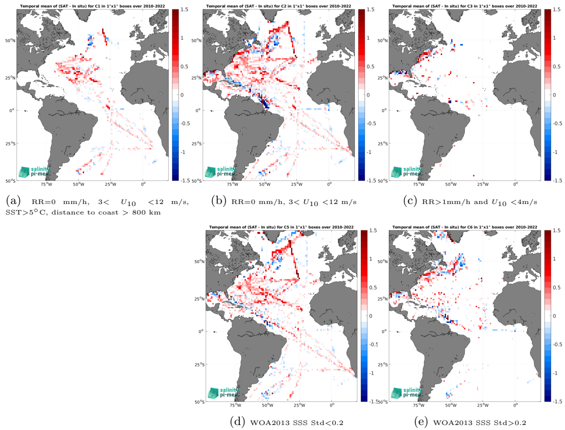
Figure 12: Temporal mean gridded over spatial boxes of size 1^\circ \times 1^\circ of \Delta SSS (SMOS SSS L3 v8 - 18 Days (CATDS-CEC-LOCEAN) - TSG (SAMOS)) for 5 different subdatasets corresponding to:RR=0 mm/h, 3 < U_{10} < 12 m/s, SST >5^\circ\text{C} , distance to coast > 800 km (a), RR=0 mm/h, 3 < U_{10} < 12 m/s (b), RR >1 mm/h and U_{10} < 4 m/s (c), WOA2013 SSS Std <0.2 (d), WOA2013 SSS Std >0.2 (e).
