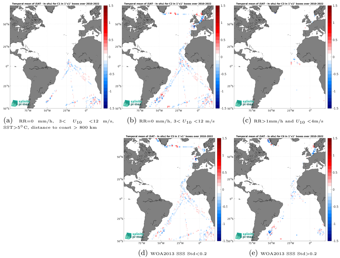
Figure 12: Temporal mean gridded over spatial boxes of size 1^\circ \times 1^\circ of \Delta SSS (SMOS SSS L3 v8 - 18 Days (CATDS-CEC-LOCEAN) - TSG (Polarstern)) for 5 different subdatasets corresponding to:RR=0 mm/h, 3 < U_{10} < 12 m/s, SST >5^\circ\text{C} , distance to coast > 800 km (a), RR=0 mm/h, 3 < U_{10} < 12 m/s (b), RR >1 mm/h and U_{10} < 4 m/s (c), WOA2013 SSS Std <0.2 (d), WOA2013 SSS Std >0.2 (e).
