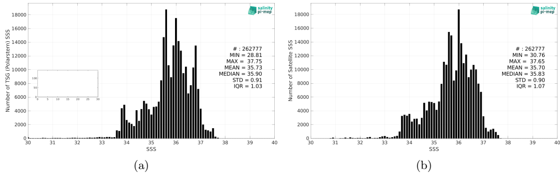
Figure 2: Histograms of SSS from TSG (Polarstern) (a) and SMOS SSS L3 v8 - 18 Days (CATDS-CEC-LOCEAN) (b) considering all match-up pairs per bins of 0.1 over the Atlantic Ocean Pi-MEP region and for the full satellite product period.
