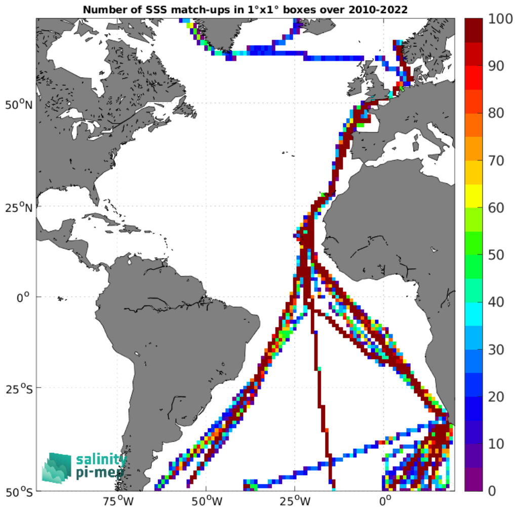
Figure 4: Number of SSS match-ups between TSG (Polarstern) SSS and the SMOS SSS L3 v8 - 18 Days (CATDS-CEC-LOCEAN) SSS product for the Atlantic Ocean Pi-MEP region over 1^\circ \times 1^\circ boxes and for the full satellite product period.
