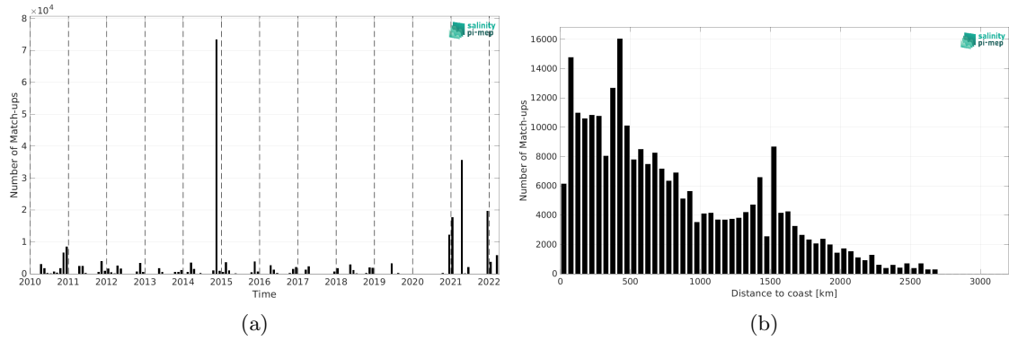
Figure 1: Number of match-ups between TSG (Polarstern) and SMOS SSS L3 v8 - 18 Days (CATDS-CEC-LOCEAN) SSS as a function of time (a) and as function of the distance to coast (b) over the Atlantic Ocean Pi-MEP region and for the full satellite product period.
