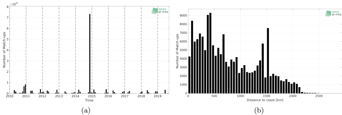
Figure 1: Number of match-ups between TSG (Polarstern) and SMOS SSS L3 v8 - 18 Days (CATDS-CECOS-LOCEAN) SSS as a function of time (a) and as function of the distance to coast (b) over the Atlantic Ocean Pi-MEP region and for the full satellite product period.
