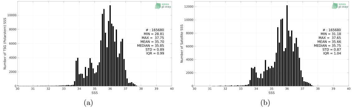
Figure 2: Histograms of SSS from TSG (Polarstern) (a) and SMOS SSS L3 v8 - 18 Days (CATDS-CECOS-LOCEAN) (b) considering all match-up pairs per bins of 0.1 over the Atlantic Ocean Pi-MEP region and for the full satellite product period.
