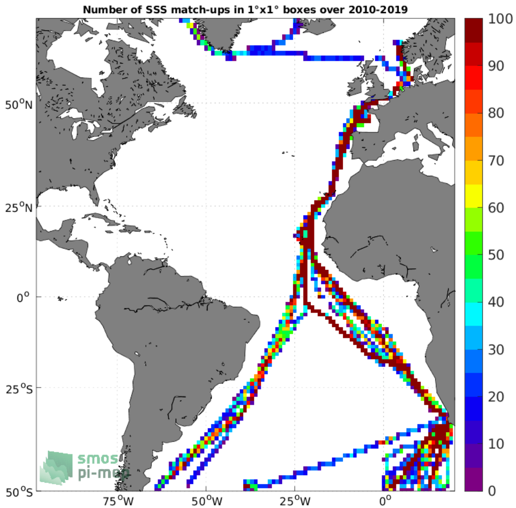
Figure 4: Number of SSS match-ups between TSG (Polarstern) SSS and the SMOS SSS L3 v8 - 18 Days (CATDS-CECOS-LOCEAN) SSS product for the Atlantic Ocean Pi-MEP region over 1°x1° boxes and for the full satellite product period.
