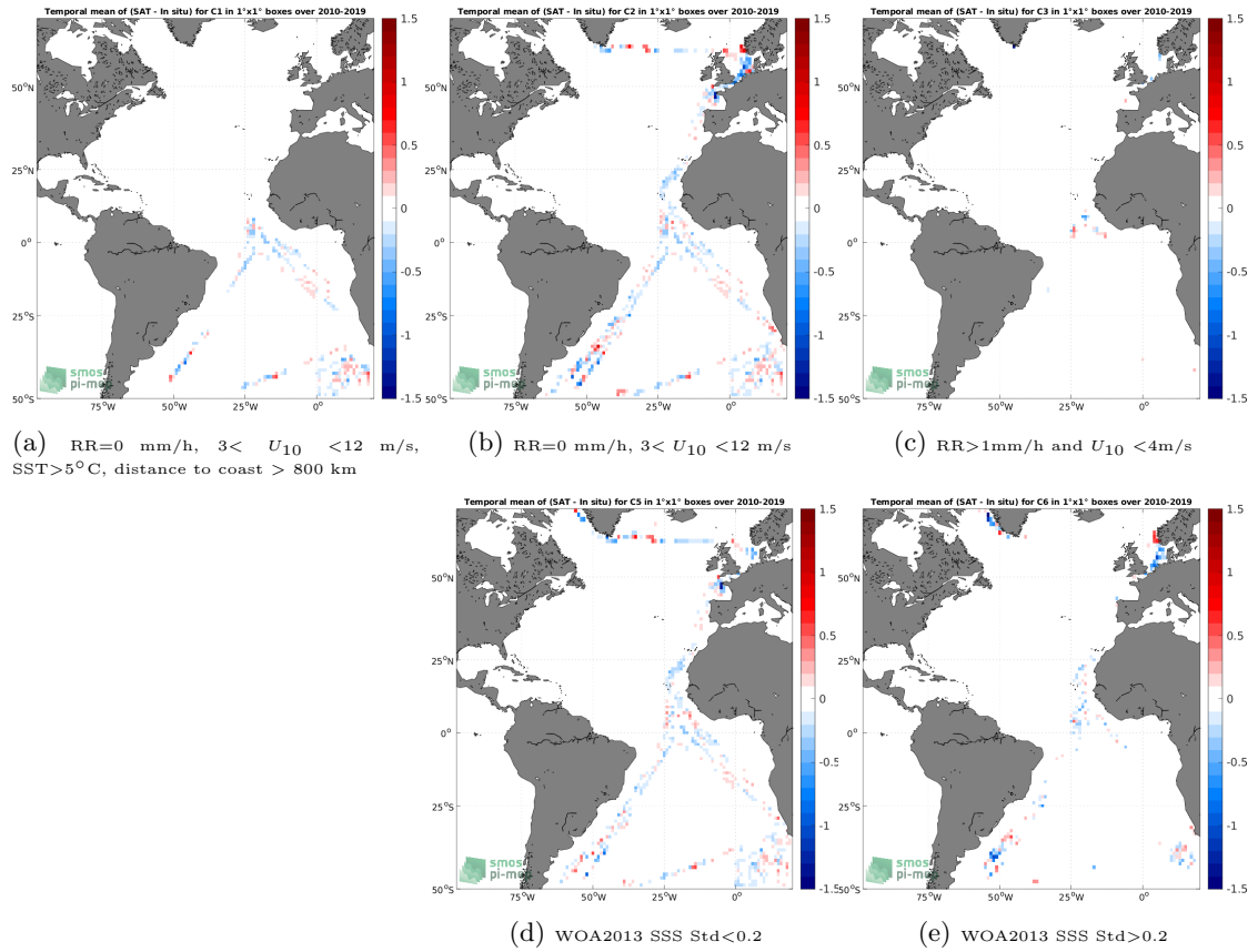
Figure 12: Temporal mean gridded over spatial boxes of size 1^\circ \times 1^\circ of \Delta SSS (SMOS SSS L3 v8 - 18 Days (CATDS-CECOS-LOCEAN) - TSG (Polarstern)) for 5 different subdatasets corresponding to:RR=0 mm/h, 3 < U_{10} < 12 m/s, SST >5^\circ\text{C} , distance to coast > 800 km (a), RR=0 mm/h, 3 < U_{10} < 12 m/s (b), RR >1 mm/h and U_{10} < 4 m/s (c), WOA2013 SSS Std <0.2 (d), WOA2013 SSS Std >0.2 (e).
