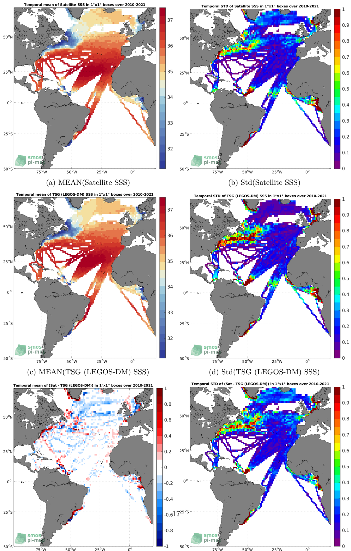
(e) MEAN( \Delta SSS) (Satellite - TSG (LEGOS-DM)) (f) Std( \Delta SSS) (Satellite - TSG (LEGOS-DM)) Figure 6: Temporal mean (left) and Std (right) of SSS from SMOS SSS L3 v8 - 18 Days (CATDS-CECOS-LOCEAN) (top), TSG (LEGOS-DM) (middle), and of \Delta SSS (Satellite - TSG (LEGOS-DM)). Only match-up pairs are used to generate these maps.
