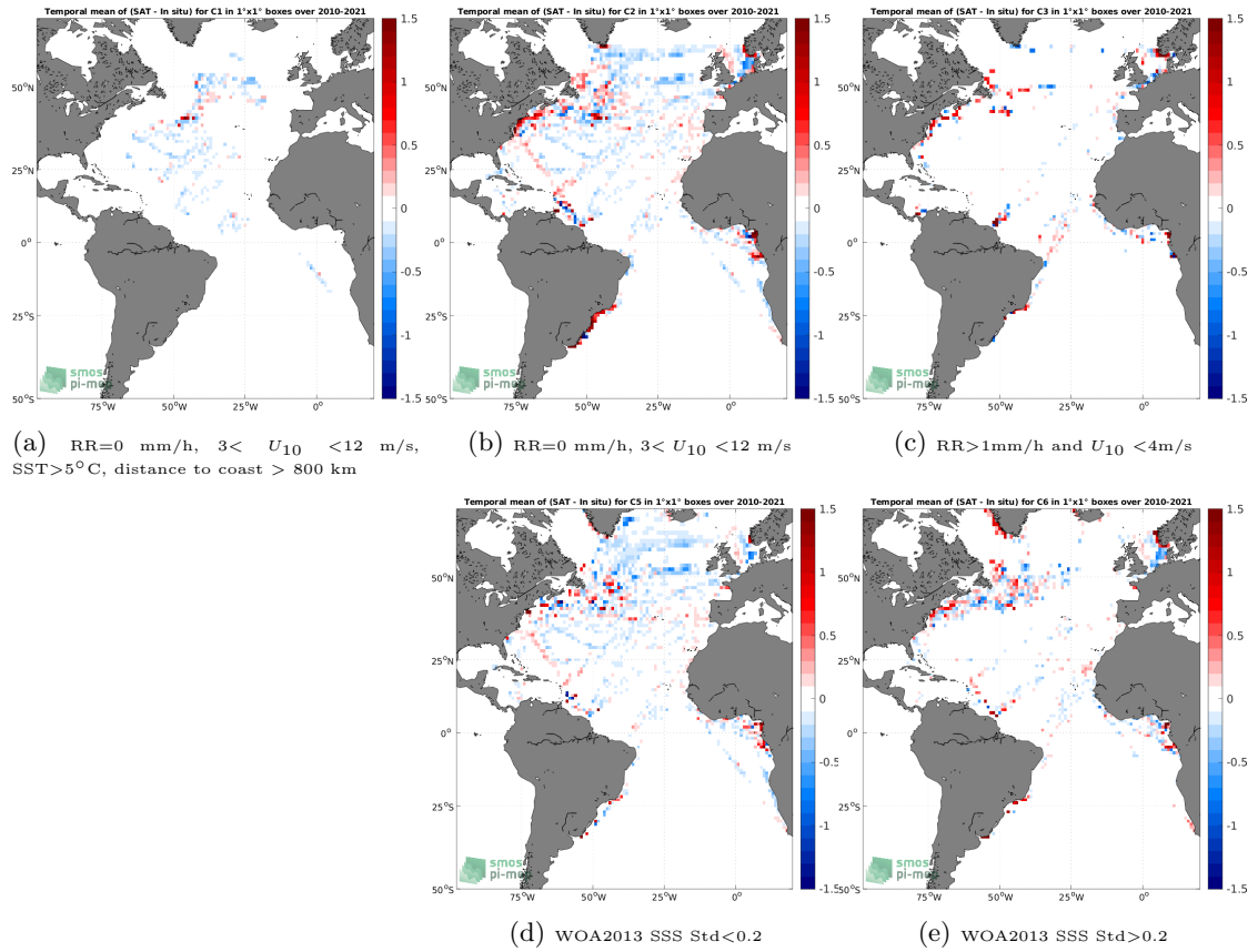
Figure 12: Temporal mean gridded over spatial boxes of size 1^\circ \times 1^\circ of \Delta\text{SSS} (SMOS SSS L3 v8 - 18 Days (CATDS-CECOS-LOCEAN) - TSG (LEGOS-DM)) for 5 different subdatasets corresponding to:RR=0 mm/h, 3 < U_{10} < 12 m/s, SST >5^\circ\text{C} , distance to coast > 800 km (a), RR=0 mm/h, 3 < U_{10} < 12 m/s (b), RR >1 mm/h and U_{10} < 4 m/s (c), WOA2013 SSS Std <0.2 (d), WOA2013 SSS Std >0.2 (e).
