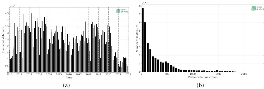
Figure 1: Number of match-ups between TSG (LEGOS-DM) and SMOS SSS L3 v8 - 18 Days (CATDS-CECOS-LOCEAN) SSS as a function of time (a) and as function of the distance to coast (b) over the Atlantic Ocean Pi-MEP region and for the full satellite product period.
