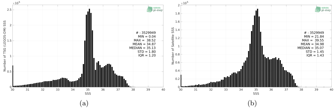
Figure 2: Histograms of SSS from TSG (LEGOS-DM) (a) and SMOS SSS L3 v8 - 18 Days (CATDS-CECOS-LOCEAN) (b) considering all match-up pairs per bins of 0.1 over the Atlantic Ocean Pi-MEP region and for the full satellite product period.
