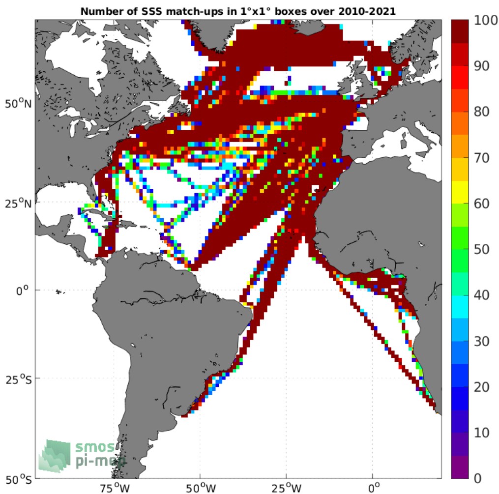
Figure 4: Number of SSS match-ups between TSG (LEGOS-DM) SSS and the SMOS SSS L3 v8 - 18 Days (CATDS-CECOS-LOCEAN) SSS product for the Atlantic Ocean Pi-MEP region over 1^\circ \times 1^\circ boxes and for the full satellite product period.
