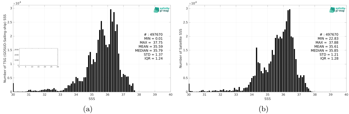
Figure 2: Histograms of SSS from TSG (GOSUD-Sailing-ship) (a) and SMOS SSS L3 v8 - 18 Days (CATDS-CEC-LOCEAN) (b) considering all match-up pairs per bins of 0.1 over the Atlantic Ocean Pi-MEP region and for the full satellite product period.
