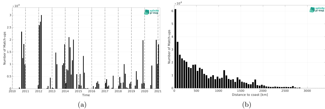
Figure 1: Number of match-ups between TSG (GOSUD-Sailing-ship) and SMOS SSS L3 v8 - 18 Days (CATDS-CEC-LOCEAN) SSS as a function of time (a) and as function of the distance to coast (b) over the Atlantic Ocean Pi-MEP region and for the full satellite product period.
