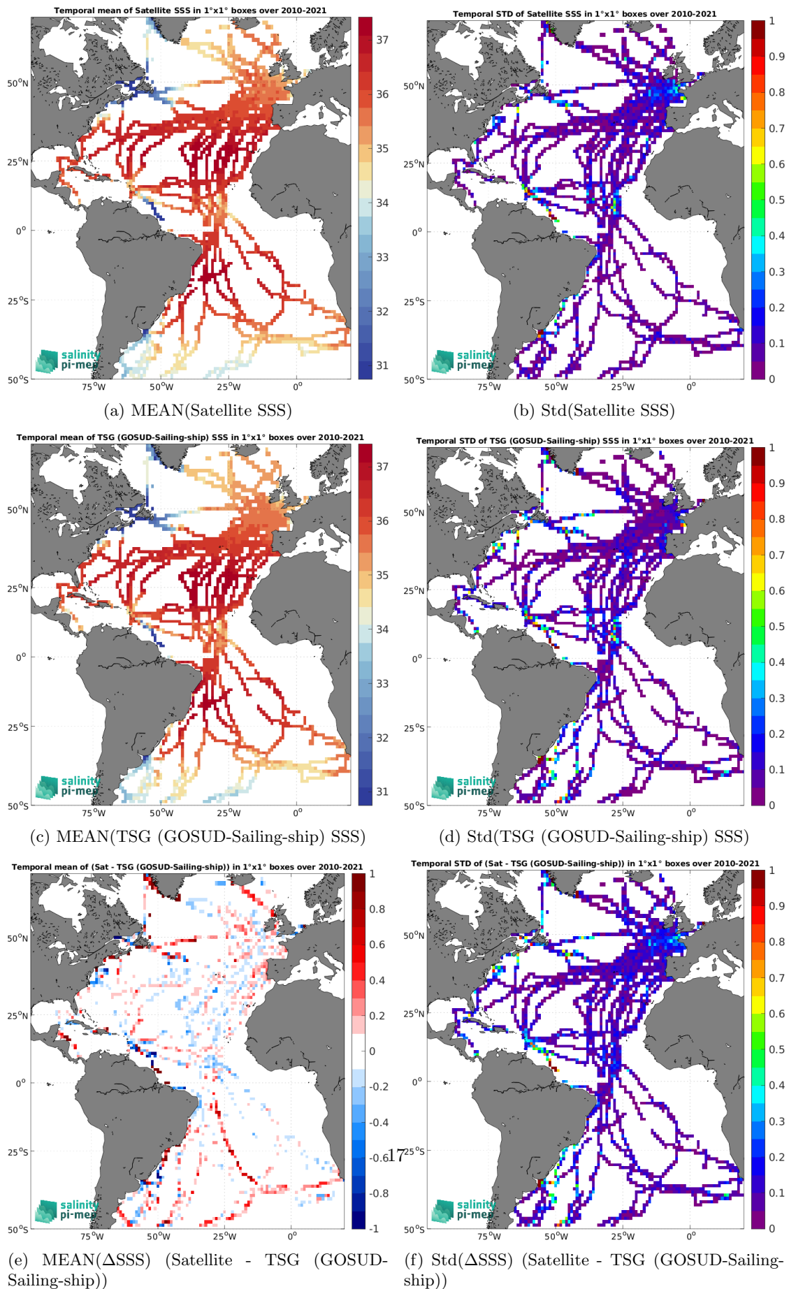
Figure 6: Temporal mean (left) and Std (right) of SSS from SMOS SSS L3 v8 - 18 Days (CATDS-CEC-LOCEAN) (top), TSG (GOSUD-Sailing-ship) (middle), and of \Delta SSS (Satellite - TSG (GOSUD-Sailing-ship)). Only match-up pairs are used to generate these maps.
