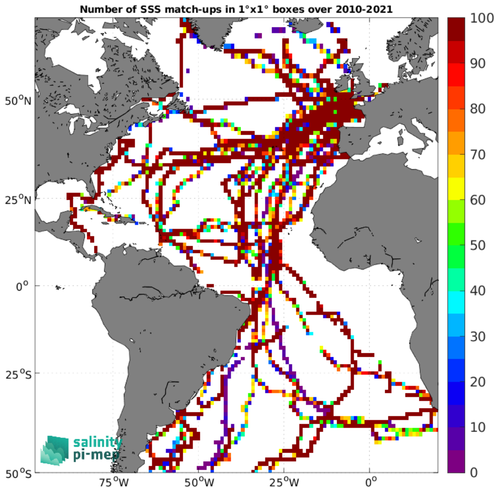
Figure 4: Number of SSS match-ups between TSG (GOSUD-Sailing-ship) SSS and the SMOS SSS L3 v8 - 18 Days (CATDS-CEC-LOCEAN) SSS product for the Atlantic Ocean Pi-MEP region over 1^{\circ} \times 1^{\circ} boxes and for the full satellite product period.
