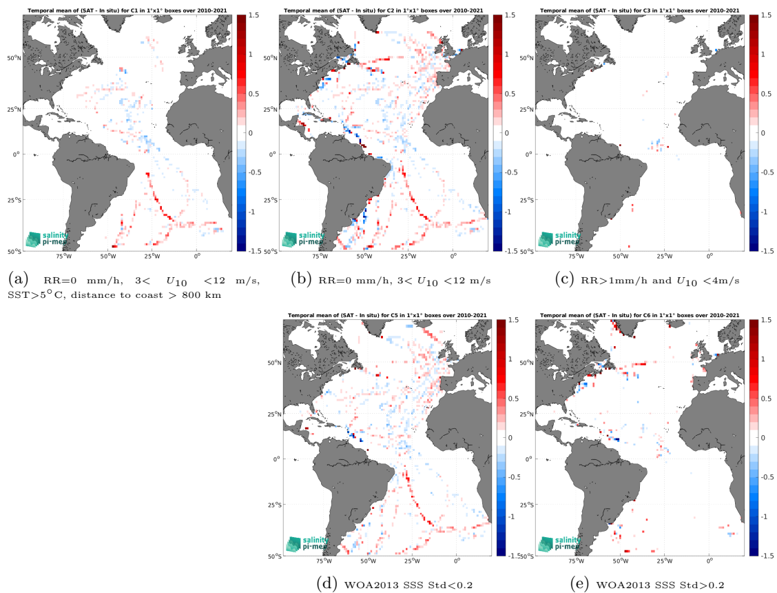
Figure 12: Temporal mean gridded over spatial boxes of size 1^\circ \times 1^\circ of \Delta\text{SSS} (SMOS SSS L3 v8 - 18 Days (CATDS-CEC-LOCEAN) - TSG (GOSUD-Sailing-ship)) for 5 different subdatasets corresponding to:RR=0 mm/h, 3 < U_{10} < 12 m/s, SST>5°C, distance to coast > 800 km (a), RR=0 mm/h, 3 < U_{10} < 12 m/s (b), RR>1mm/h and U_{10} < 4 m/s (c), WOA2013 SSS Std<0.2 (d), WOA2013 SSS Std>0.2 (e).
