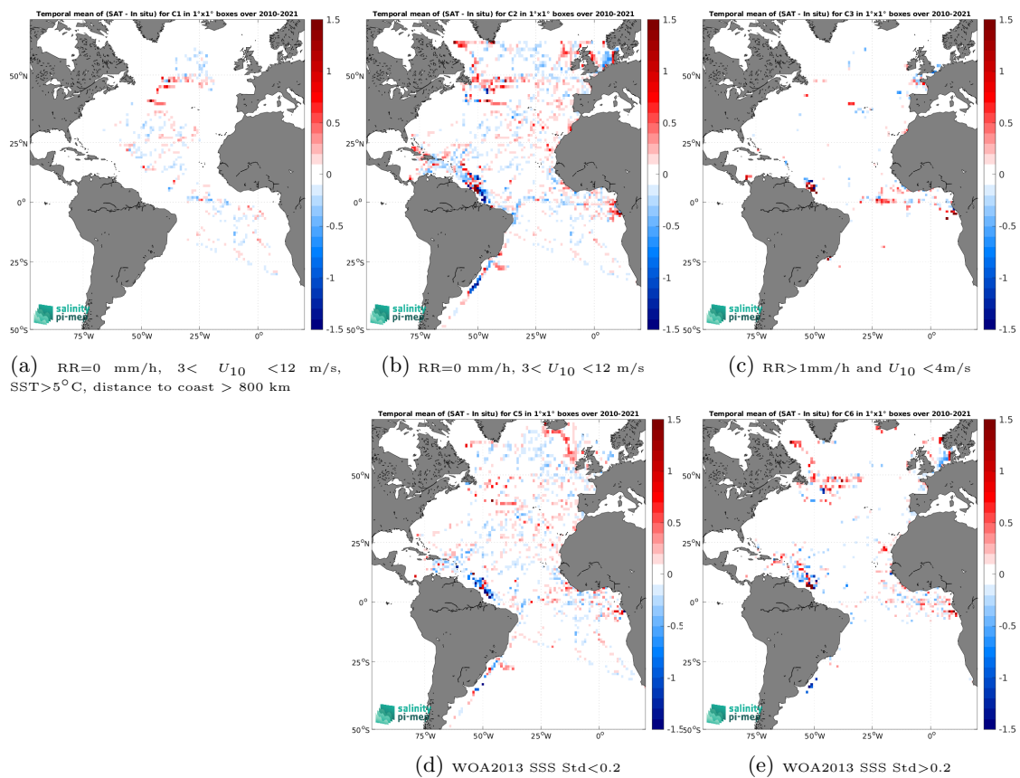
Figure 12: Temporal mean gridded over spatial boxes of size 1^\circ \times 1^\circ of \Delta SSS (SMOS SSS L3 v8 - 18 Days (CATDS-CEC-LOCEAN) - TSG (GOSUD-Research-vessel)) for 5 different subdatasets corresponding to:RR=0 mm/h, 3 < U_{10} < 12 m/s, SST >5^\circ\text{C} , distance to coast > 800 km (a), RR=0 mm/h, 3 < U_{10} < 12 m/s (b), RR >1 mm/h and U_{10} < 4 m/s (c), WOA2013 SSS Std <0.2 (d), WOA2013 SSS Std >0.2 (e).
