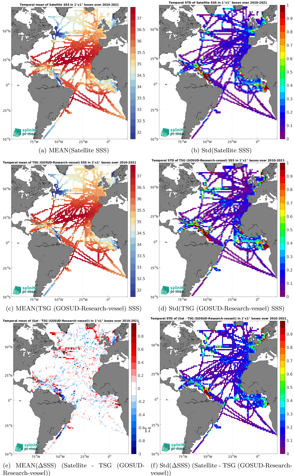
Figure 6: Temporal mean (left) and Std (right) of SSS from SMOS SSS L3 v8 - 18 Days (CATDS-CEC-LOCEAN) (top), TSG (GOSUD-Research-vessel) (middle), and of \Delta SSS (Satellite - TSG (GOSUD-Research-vessel)). Only match-up pairs are used to generate these maps.
