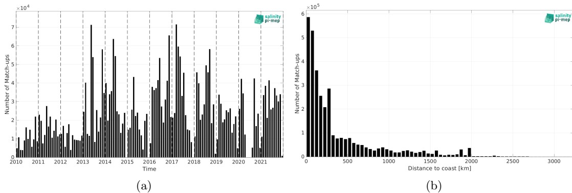
Figure 1: Number of match-ups between TSG (GOSUD-Research-vessel) and SMOS SSS L3 v8 - 18 Days (CATDS-CEC-LOCEAN) SSS as a function of time (a) and as function of the distance to coast (b) over the Atlantic Ocean Pi-MEP region and for the full satellite product period.
