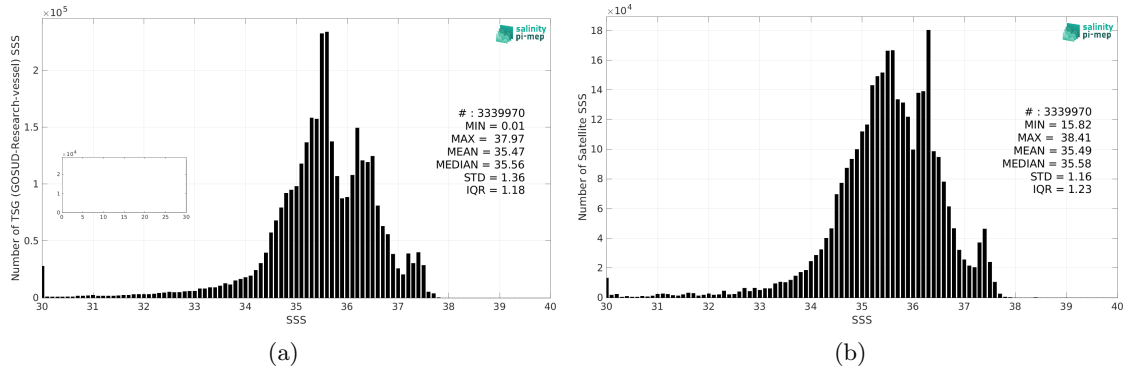
Figure 2: Histograms of SSS from TSG (GOSUD-Research-vessel) (a) and SMOS SSS L3 v8 - 18 Days (CATDS-CEC-LOCEAN) (b) considering all match-up pairs per bins of 0.1 over the Atlantic Ocean Pi-MEP region and for the full satellite product period.
