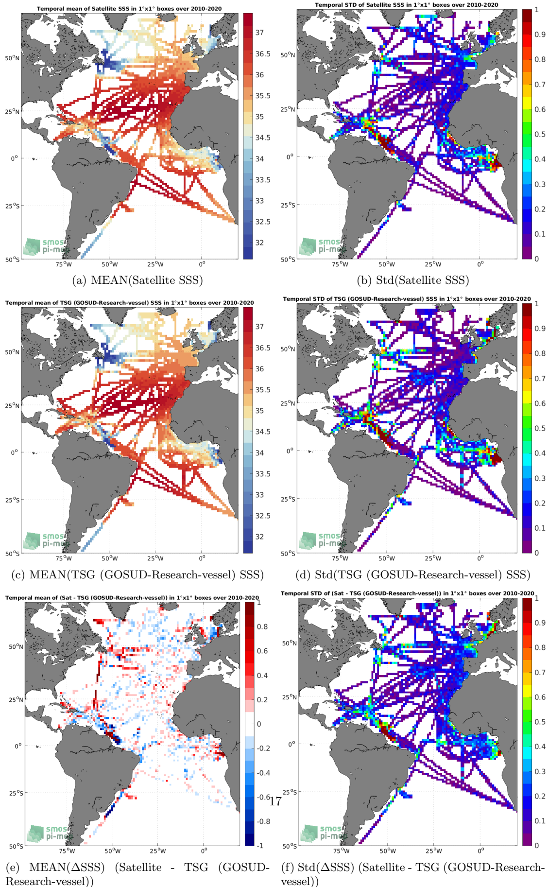
Figure 6: Temporal mean (left) and Std (right) of SSS from SMOS SSS L3 v8 - 18 Days (CATDS-CECOS-LOCEAN) (top), TSG (GOSUD-Research-vessel) (middle), and of \Delta SSS (Satellite - TSG (GOSUD-Research-vessel)). Only match-up pairs are used to generate these maps.
