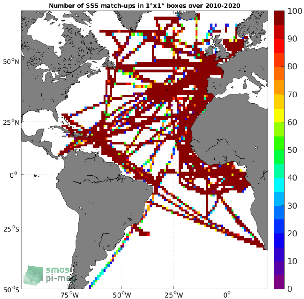
Figure 4: Number of SSS match-ups between TSG (GOSUD-Research-vessel) SSS and the SMOS SSS L3 v8 - 18 Days (CATDS-CECOS-LOCEAN) SSS product for the Atlantic Ocean Pi-MEP region over 1°x1° boxes and for the full satellite product period.
