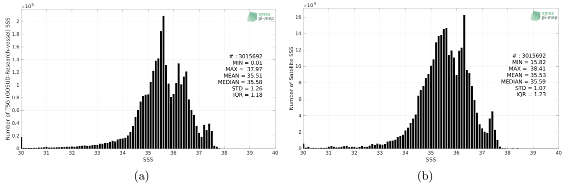
Figure 2: Histograms of SSS from TSG (GOSUD-Research-vessel) (a) and SMOS SSS L3 v8 - 18 Days (CATDS-CECOS-LOCEAN) (b) considering all match-up pairs per bins of 0.1 over the Atlantic Ocean Pi-MEP region and for the full satellite product period.
