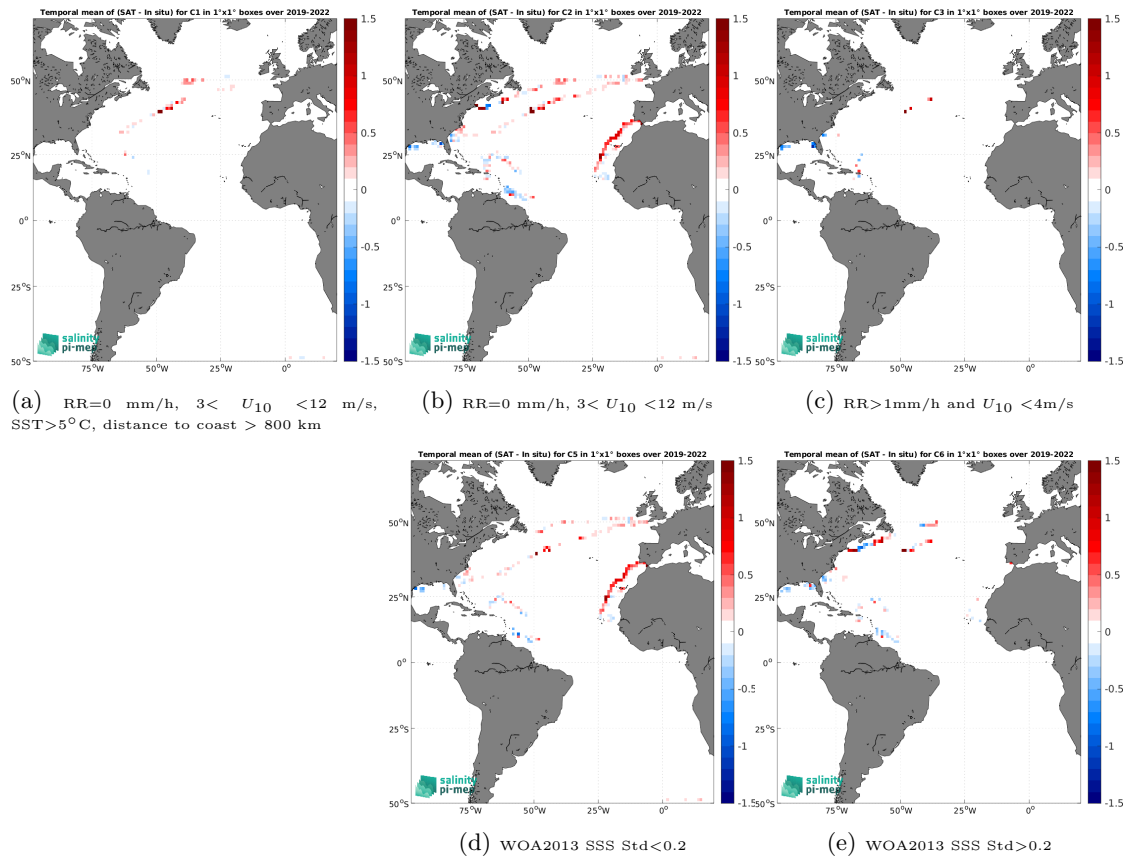
Figure 12: Temporal mean gridded over spatial boxes of size 1^\circ \times 1^\circ of \Delta\text{SSS} (SMOS SSS L3 v8 - 18 Days (CATDS-CEC-LOCEAN) - Sailydrone) for 5 different subdatasets corresponding to:RR=0 mm/h, 3 < U_{10} < 12 m/s, SST >5^\circ\text{C} , distance to coast > 800 km (a), RR=0 mm/h, 3 < U_{10} < 12 m/s (b), RR >1 mm/h and U_{10} < 4 m/s (c), WOA2013 SSS Std <0.2 (d), WOA2013 SSS Std >0.2 (e).
