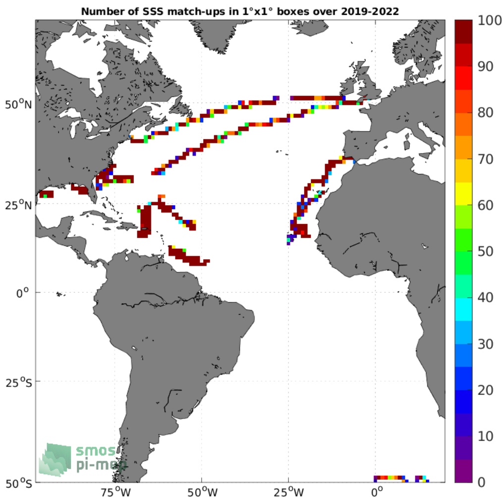
Figure 4: Number of SSS match-ups between Saildrone SSS and the SMOS SSS L3 v8 - 18 Days (CATDS-CECOS-LOCEAN) SSS product for the Atlantic Ocean Pi-MEP region over 1^\circ \times 1^\circ boxes and for the full satellite product period.
