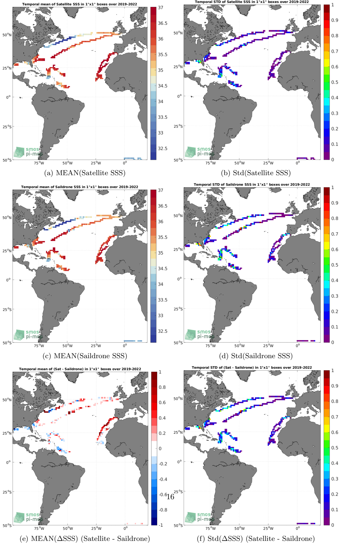
Figure 6: Temporal mean (left) and Std (right) of SSS from SMOS SSS L3 v8 - 18 Days (CATDS-CECOS-LOCEAN) (top), Saildrone (middle), and of \Delta SSS (Satellite - Saildrone). Only match-up pairs are used to generate these maps.
