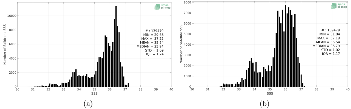
Figure 2: Histograms of SSS from Saildrone (a) and SMOS SSS L3 v8 - 18 Days (CATDS-CECOS-LOCEAN) (b) considering all match-up pairs per bins of 0.1 over the Atlantic Ocean Pi-MEP region and for the full satellite product period.
