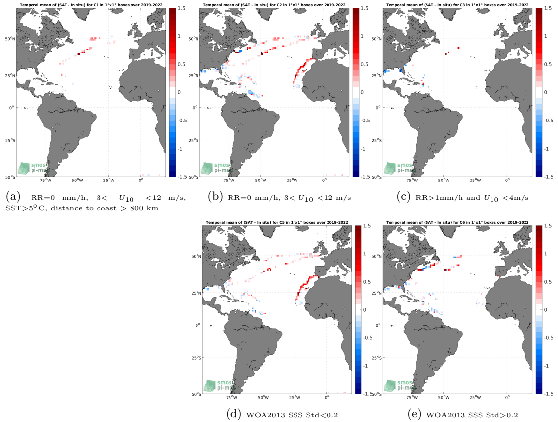
Figure 12: Temporal mean gridded over spatial boxes of size 1^\circ \times 1^\circ of \Delta SSS (SMOS SSS L3 v8 - 18 Days (CATDS-CECOS-LOCEAN) - Saildrone) for 5 different subdatasets corresponding to:RR=0 mm/h, 3 < U_{10} < 12 m/s, SST >5^\circ\text{C} , distance to coast > 800 km (a), RR=0 mm/h, 3 < U_{10} < 12 m/s (b), RR >1 mm/h and U_{10} < 4 m/s (c), WOA2013 SSS Std <0.2 (d), WOA2013 SSS Std >0.2 (e).
