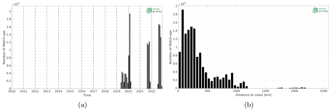
Figure 1: Number of match-ups between Saildrone and SMOS SSS L3 v8 - 18 Days (CATDS-CECOS-LOCEAN) SSS as a function of time (a) and as function of the distance to coast (b) over the Atlantic Ocean Pi-MEP region and for the full satellite product period.
