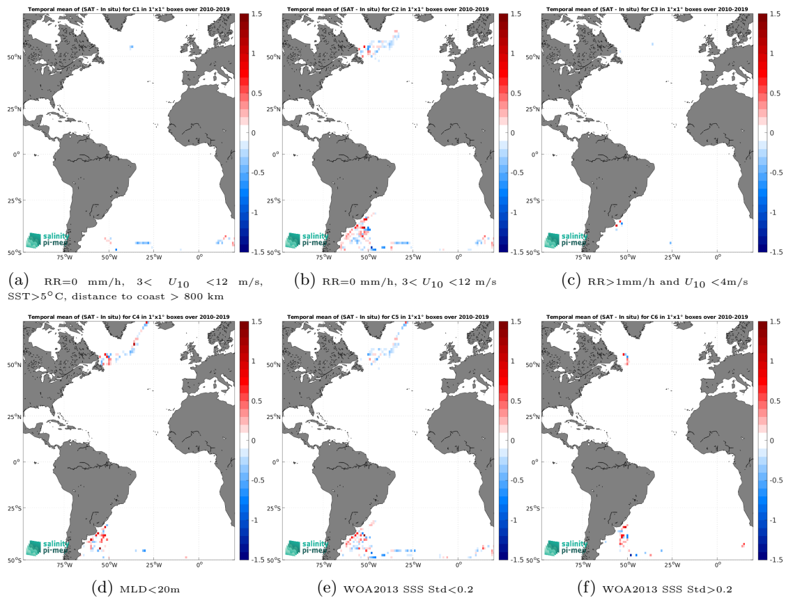
Figure 12: Temporal mean gridded over spatial boxes of size 1^\circ \times 1^\circ of \Delta SSS (SMOS SSS L3 v8 - 18 Days (CATDS-CEC-LOCEAN) - Marine mammals) for 6 different subdatasets corresponding to: RR=0 mm/h, 3 < U_{10} < 12 m/s, SST > 5°C, distance to coast > 800 km (a), RR=0 mm/h, 3 < U_{10} < 12 m/s (b), RR > 1mm/h and U_{10} < 4 m/s (c), MLD < 20m (d), WOA2013 SSS Std < 0.2 (e), WOA2013 SSS Std > 0.2 (f).
