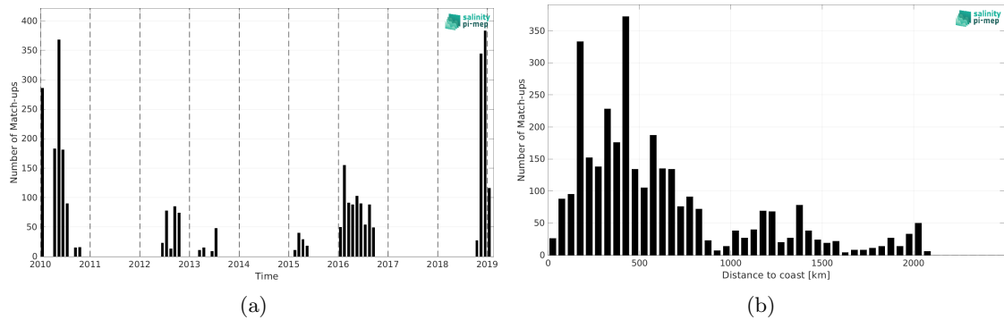
Figure 1: Number of match-ups between Marine mammals and SMOS SSS L3 v8 - 18 Days (CATDS-CEC-LOCEAN) SSS as a function of time (a) and as function of the distance to coast (b) over the Atlantic Ocean Pi-MEP region and for the full satellite product period.
