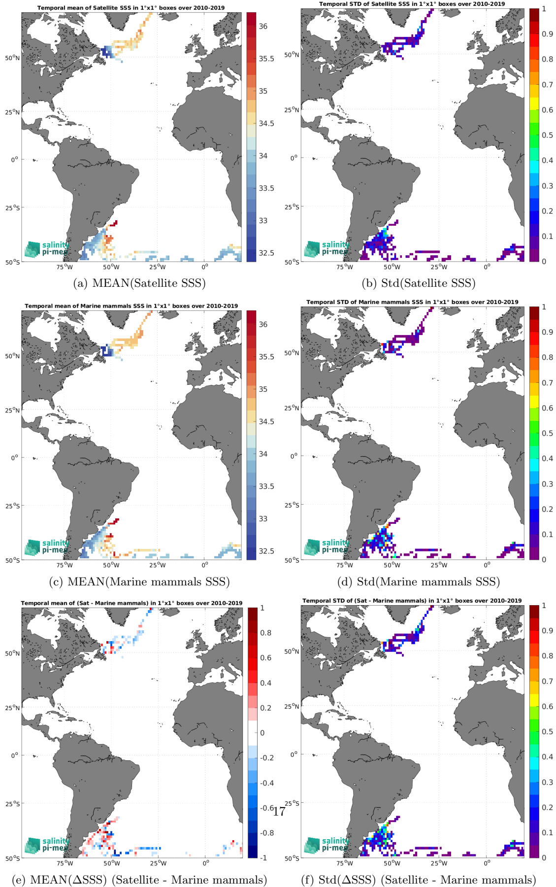
Figure 6: Temporal mean (left) and Std (right) of SSS from SMOS SSS L3 v8 - 18 Days (CATDS-CEC-LOCEAN) (top), Marine mammals (middle), and of \Delta SSS (Satellite - Marine mammals). Only match-up pairs are used to generate these maps.
