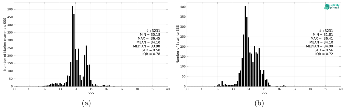
Figure 2: Histograms of SSS from Marine mammals (a) and SMOS SSS L3 v8 - 18 Days (CATDS-CEC-LOCEAN) (b) considering all match-up pairs per bins of 0.1 over the Atlantic Ocean Pi-MEP region and for the full satellite product period.
