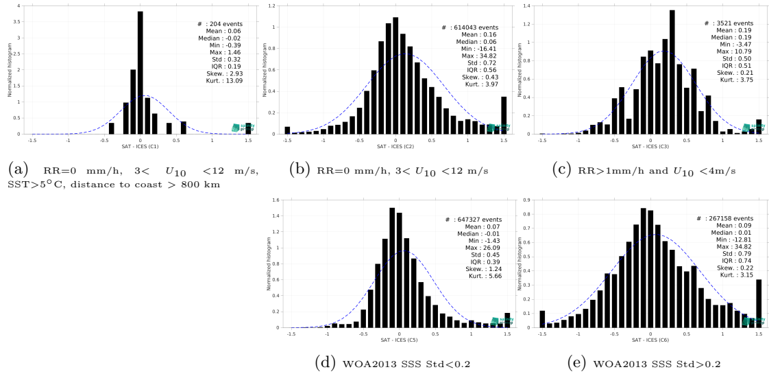
Figure 13: Normalized histogram of \Delta SSS (SMOS SSS L3 v8 - 18 Days (CATDS-CEC-LOCEAN) - ICES) for 5 different subdatasets corresponding to: RR=0 mm/h, 3 < U_{10} < 12 m/s, SST > 5°C, distance to coast > 800 km (a), RR=0 mm/h, 3 < U_{10} < 12 m/s (b), RR > 1mm/h and U_{10} < 4 m/s (c), WOA2013 SSS Std < 0.2 (d), WOA2013 SSS Std > 0.2 (e).
