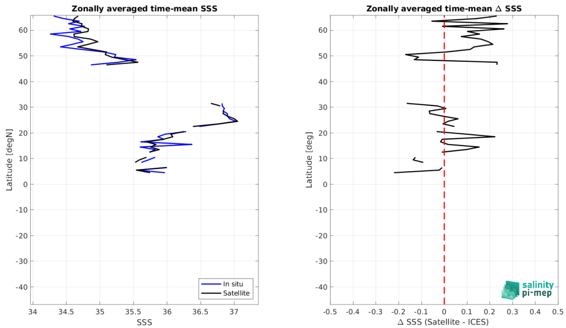
Figure 8: Left panel: Zonal mean SSS from SMOS SSS L3 v8 - 18 Days (CATDS-CEC-LOCEAN) satellite product (black) and from ICES (blue). Right panel: Zonal mean of \Delta SSS (Satellite - ICES) for all the collected Pi-MEP match-up pairs estimated over the full satellite product period.
