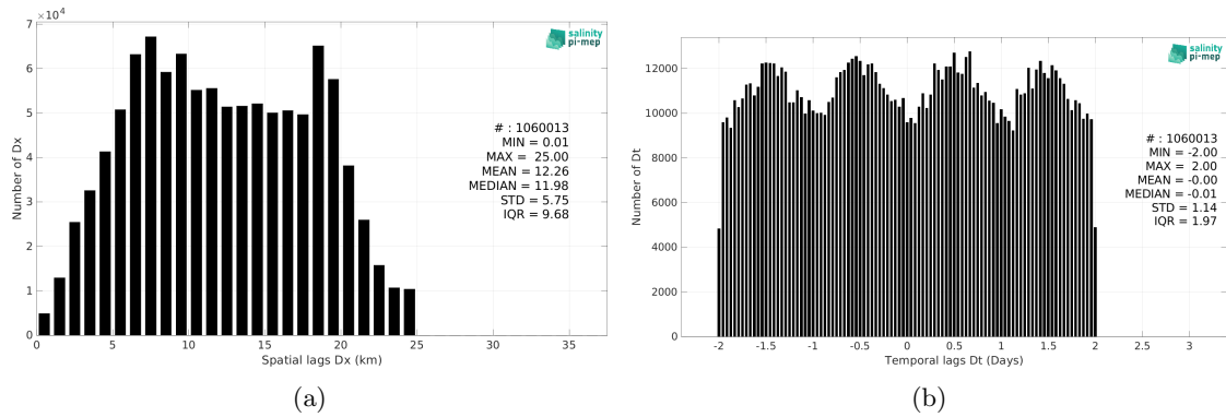
Figure 5: Histograms of the spatial (a) and temporal (b) lags between the location/time of the ICES measurement and the date of the corresponding SMOS SSS L3 v8 - 18 Days (CATDS-CEC-LOCEAN) SSS pixel.
