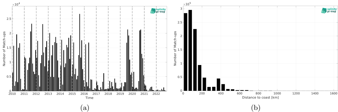
Figure 1: Number of match-ups between ICES and SMOS SSS L3 v8 - 18 Days (CATDS-CEC-LOCEAN) SSS as a function of time (a) and as function of the distance to coast (b) over the Atlantic Ocean Pi-MEP region and for the full satellite product period.
