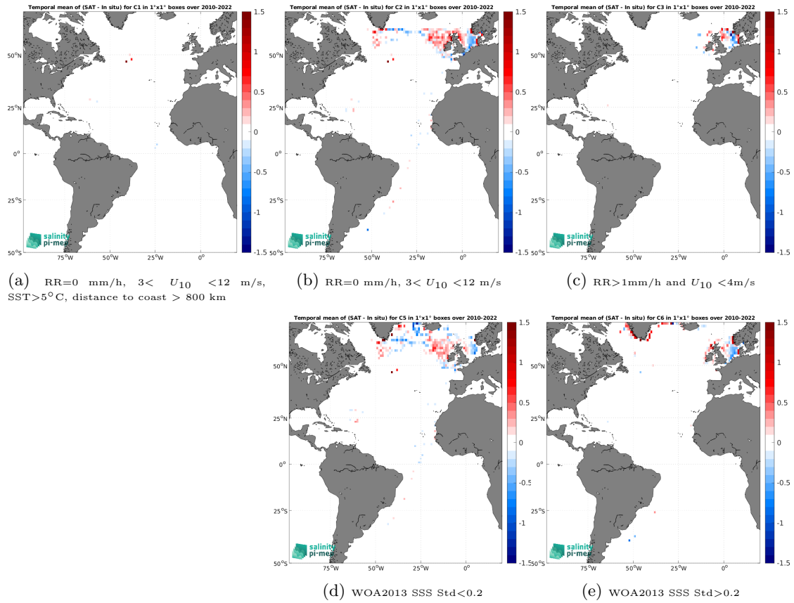
Figure 12: Temporal mean gridded over spatial boxes of size 1^\circ \times 1^\circ of \Delta SSS (SMOS SSS L3 v8 - 18 Days (CATDS-CEC-LOCEAN) - ICES) for 5 different subdatasets corresponding to:RR=0 mm/h, 3 < U_{10} < 12 m/s, SST >5^\circ\text{C} , distance to coast > 800 km (a), RR=0 mm/h, 3 < U_{10} < 12 m/s (b), RR >1 mm/h and U_{10} < 4 m/s (c), WOA2013 SSS Std <0.2 (d), WOA2013 SSS Std >0.2 (e).
