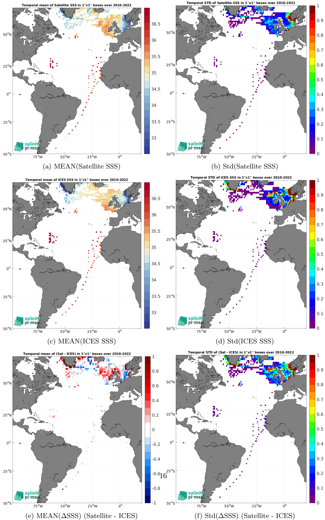
Figure 6: Temporal mean (left) and Std (right) of SSS from SMOS SSS L3 v8 - 18 Days (CATDS-CEC-LOCEAN) (top), ICES (middle), and of \Delta SSS (Satellite - ICES). Only match-up pairs are used to generate these maps.
