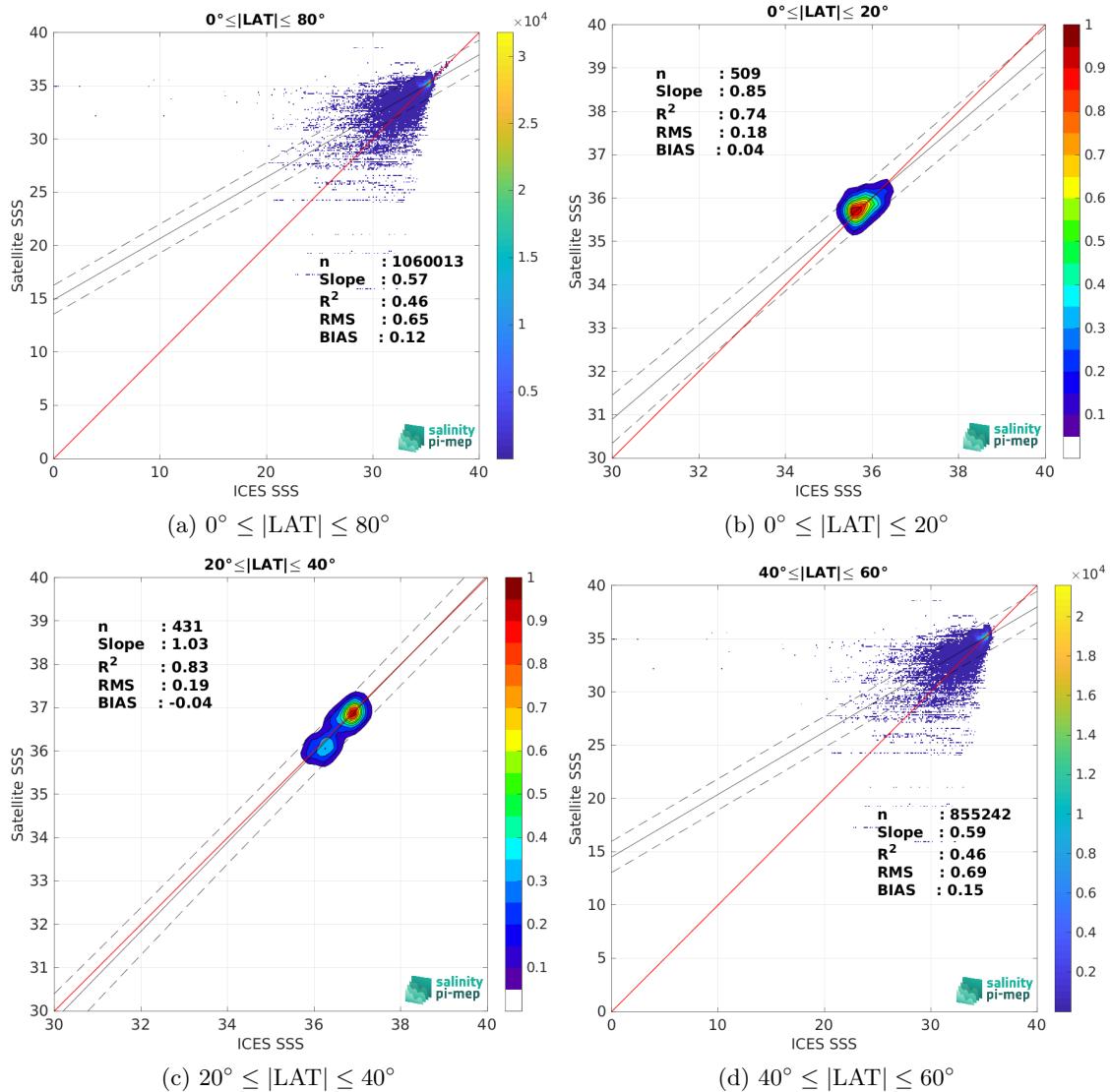
Figure 9: Contour maps of the concentration of SMOS SSS L3 v8 - 18 Days (CATDS-CEC-LOCEAN) SSS (y-axis) versus ICES SSS (x-axis) at match-up pairs for different latitude bands. For each plot, the red line shows x=y . The black thin and dashed lines indicate a linear fit through the data cloud and the \pm 95\% confidence levels, respectively. The number match-up pairs n , the slope and R^2 coefficient of the linear fit, the root mean square (RMS) and the mean bias between satellite and in situ data are indicated for each latitude band in each plots.
