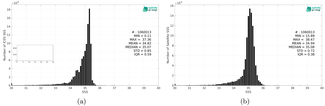
Figure 2: Histograms of SSS from ICES (a) and SMOS SSS L3 v8 - 18 Days (CATDS-CEC-LOCEAN) (b) considering all match-up pairs per bins of 0.1 over the Atlantic Ocean Pi-MEP region and for the full satellite product period.
