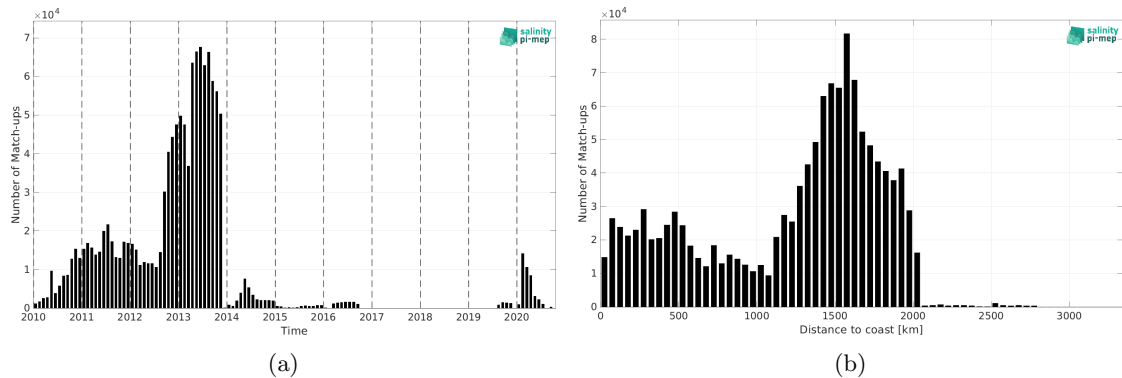
Figure 1: Number of match-ups between Surface drifters and SMOS SSS L3 v8 - 18 Days (CATDS-CEC-LOCEAN) SSS as a function of time (a) and as function of the distance to coast (b) over the Atlantic Ocean Pi-MEP region and for the full satellite product period.
