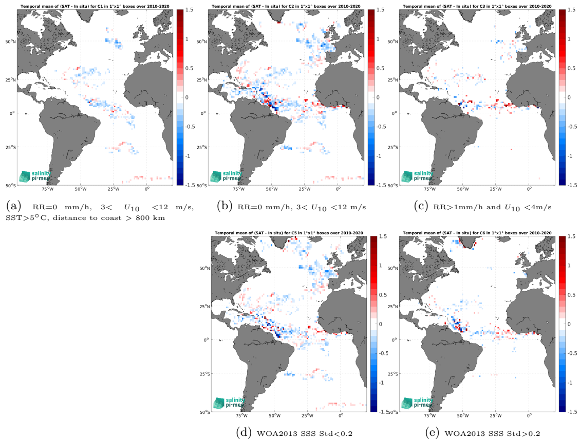
Figure 11: Temporal mean gridded over spatial boxes of size 1^\circ \times 1^\circ of \Delta SSS (SMOS SSS L3 v8 - 18 Days (CATDS-CEC-LOCEAN) - Surface drifters) for 5 different subdatasets corresponding to:RR=0 mm/h, 3 < U_{10} < 12 m/s, SST >5^\circ\text{C} , distance to coast > 800 km (a), RR=0 mm/h, 3 < U_{10} < 12 m/s (b), RR >1 mm/h and U_{10} < 4 m/s (c), WOA2013 SSS Std <0.2 (d), WOA2013 SSS Std >0.2 (e).
