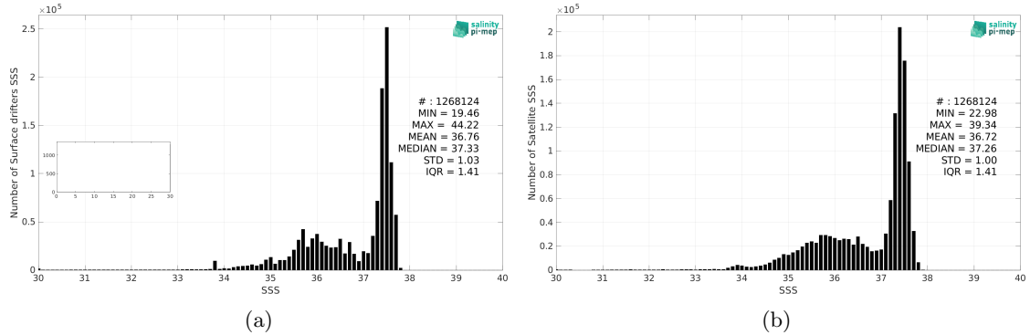
Figure 2: Histograms of SSS from Surface drifters (a) and SMOS SSS L3 v8 - 18 Days (CATDS-CEC-LOCEAN) (b) considering all match-up pairs per bins of 0.1 over the Atlantic Ocean Pi-MEP region and for the full satellite product period.
