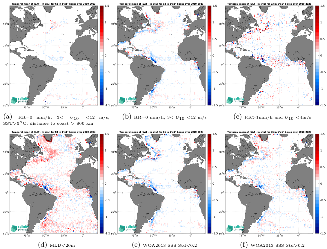
Figure 12: Temporal mean gridded over spatial boxes of size 1^\circ \times 1^\circ of \Delta SSS (SMOS SSS L3 v8 - 18 Days (CATDS-CEC-LOCEAN) - Argo) for 6 different subdatasets corresponding to:RR=0 mm/h, 3 < U_{10} < 12 m/s, SST > 5^\circ C, distance to coast > 800 km (a), RR=0 mm/h, 3 < U_{10} < 12 m/s (b), RR > 1 mm/h and U_{10} < 4 m/s (c),MLD < 20 m (d),WOA2013 SSS Std < 0.2 (e),WOA2013 SSS Std > 0.2 (f).
