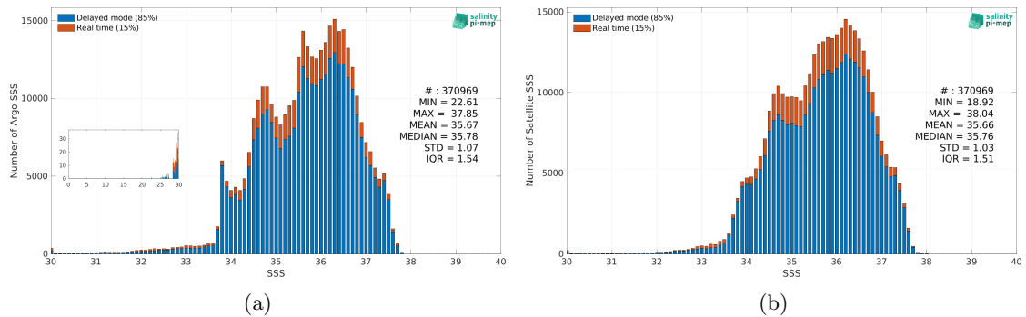
Figure 2: Histograms of SSS from Argo (a) and SMOS SSS L3 v8 - 18 Days (CATDS-CEC-LOCEAN) (b) considering all match-up pairs per bins of 0.1 over the Atlantic Ocean Pi-MEP region and for the full satellite product period.
