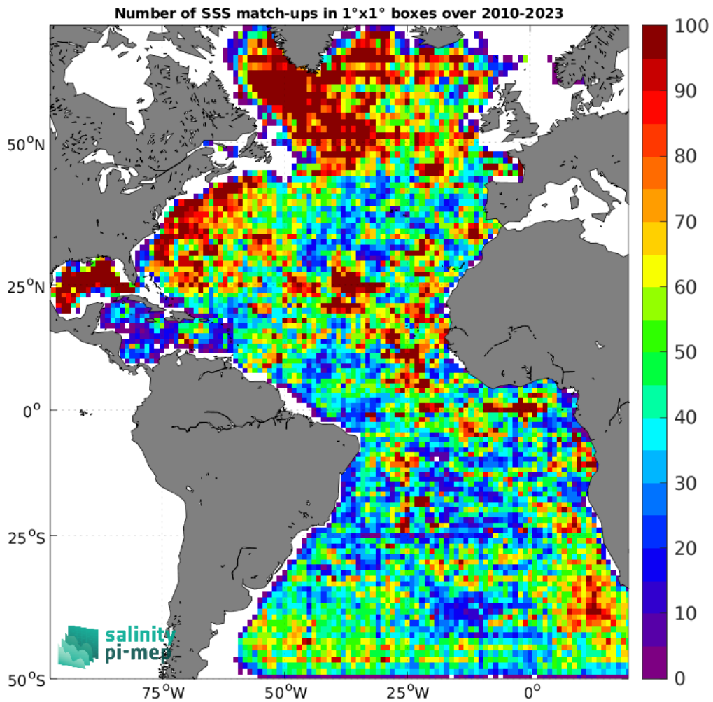
Figure 4: Number of SSS match-ups between Argo SSS and the SMOS SSS L3 v8 - 18 Days (CATDS-CEC-LOCEAN) SSS product for the Atlantic Ocean Pi-MEP region over 1^\circ \times 1^\circ boxes and for the full satellite product period.
