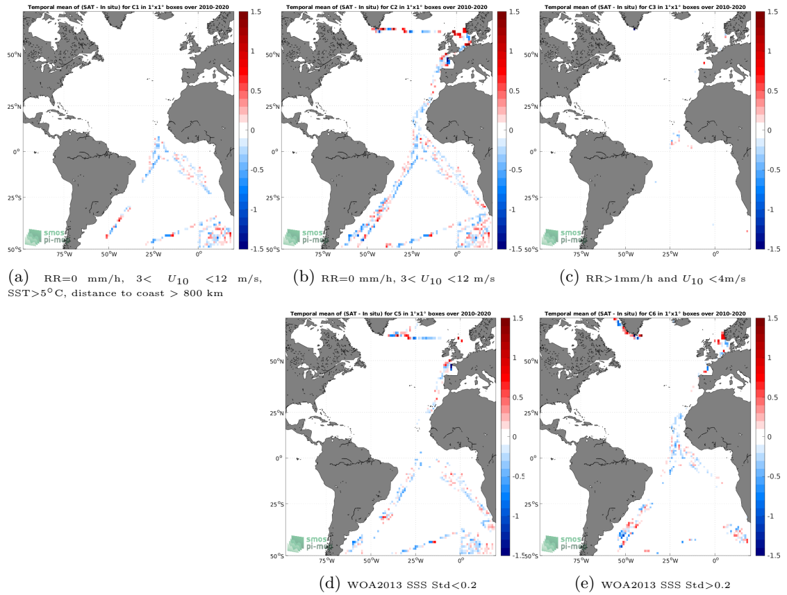
Figure 12: Temporal mean gridded over spatial boxes of size 1^\circ \times 1^\circ of \Delta SSS (SMOS SSS L3 v7 - 9 Days (CATDS-CECOS-LOCEAN) - TSG (Polarstern)) for 5 different subdatasets corresponding to:RR=0 mm/h, 3 < U_{10} < 12 m/s, SST >5^\circ\text{C} , distance to coast > 800 km (a), RR=0 mm/h, 3 < U_{10} < 12 m/s (b), RR >1 mm/h and U_{10} < 4 m/s (c), WOA2013 SSS Std <0.2 (d), WOA2013 SSS Std >0.2 (e).
