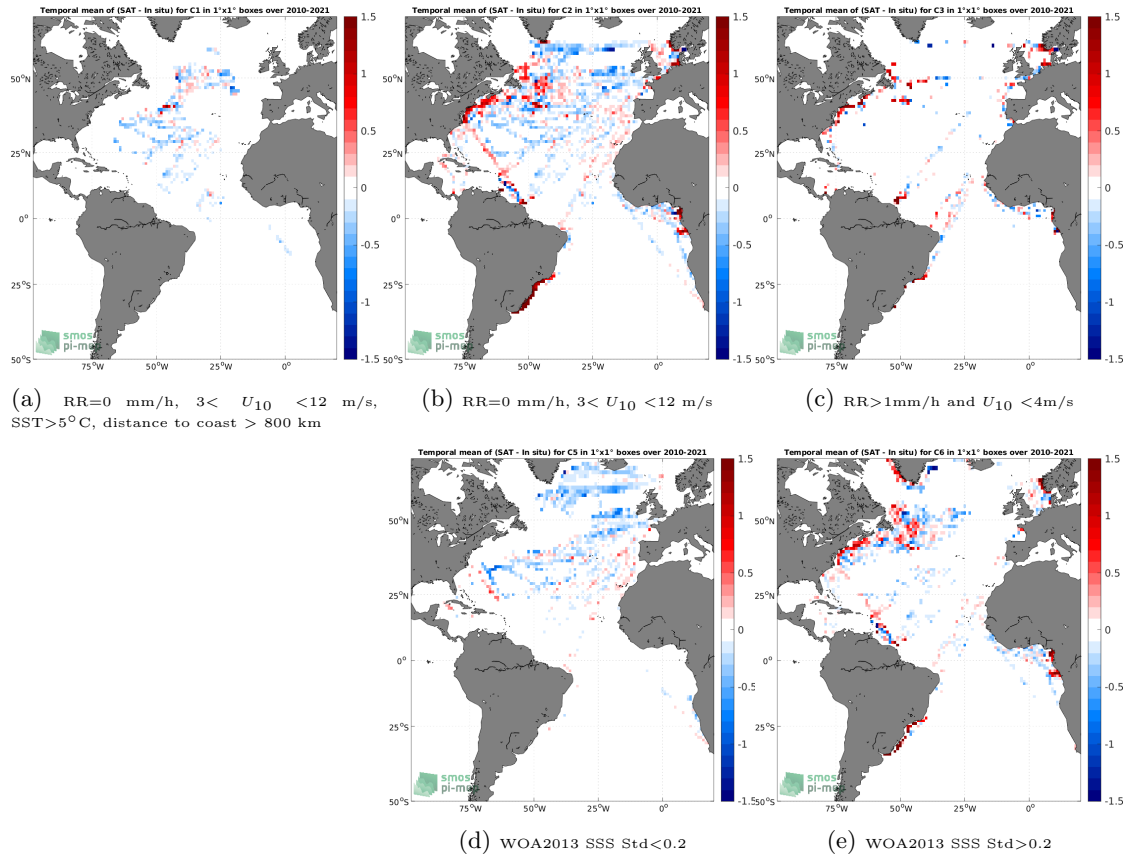
Figure 12: Temporal mean gridded over spatial boxes of size 1^\circ \times 1^\circ of \Delta\text{SSS} (SMOS SSS L3 v7 - 9 Days (CATDS-CECOS-LOCEAN) - TSG (LEGOS-DM)) for 5 different subdatasets corresponding to:RR=0 mm/h, 3 < U_{10} < 12 m/s, SST >5^\circ\text{C} , distance to coast > 800 km (a), RR=0 mm/h, 3 < U_{10} < 12 m/s (b), RR >1 mm/h and U_{10} < 4 m/s (c), WOA2013 SSS Std <0.2 (d), WOA2013 SSS Std >0.2 (e).
