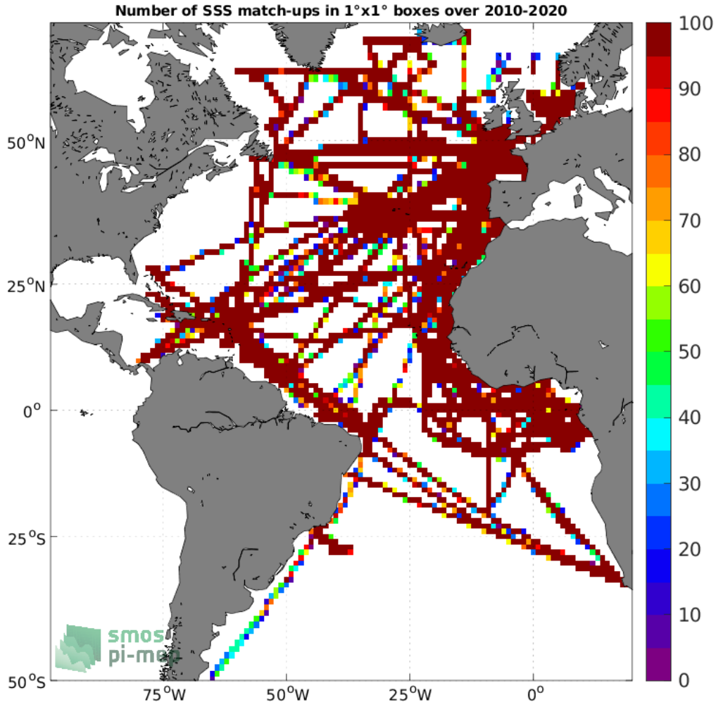
Figure 4: Number of SSS match-ups between TSG (GOSUD-Research-vessel) SSS and the SMOS SSS L3 v7 - 9 Days (CATDS-CECOS-LOCEAN) SSS product for the Atlantic Ocean Pi-MEP region over 1^\circ \times 1^\circ boxes and for the full satellite product period.
