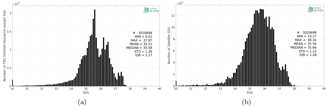
Figure 2: Histograms of SSS from TSG (GOSUD-Research-vessel) (a) and SMOS SSS L3 v7 - 9 Days (CATDS-CECOS-LOCEAN) (b) considering all match-up pairs per bins of 0.1 over the Atlantic Ocean Pi-MEP region and for the full satellite product period.
