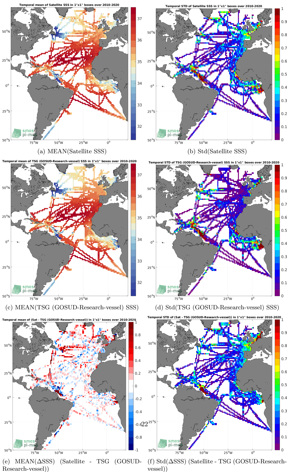
Figure 6: Temporal mean (left) and Std (right) of SSS from SMOS SSS L3 v7 - 9 Days (CATDS-CECOS-LOCEAN) (top), TSG (GOSUD-Research-vessel) (middle), and of \Delta SSS (Satellite - TSG (GOSUD-Research-vessel)). Only match-up pairs are used to generate these maps.
