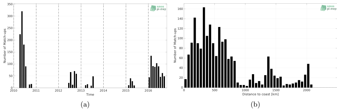
Figure 1: Number of match-ups between Marine mammals and SMOS SSS L3 v7 - 9 Days (CATDS-CECOS-LOCEAN) SSS as a function of time (a) and as function of the distance to coast (b) over the Atlantic Ocean Pi-MEP region and for the full satellite product period.
