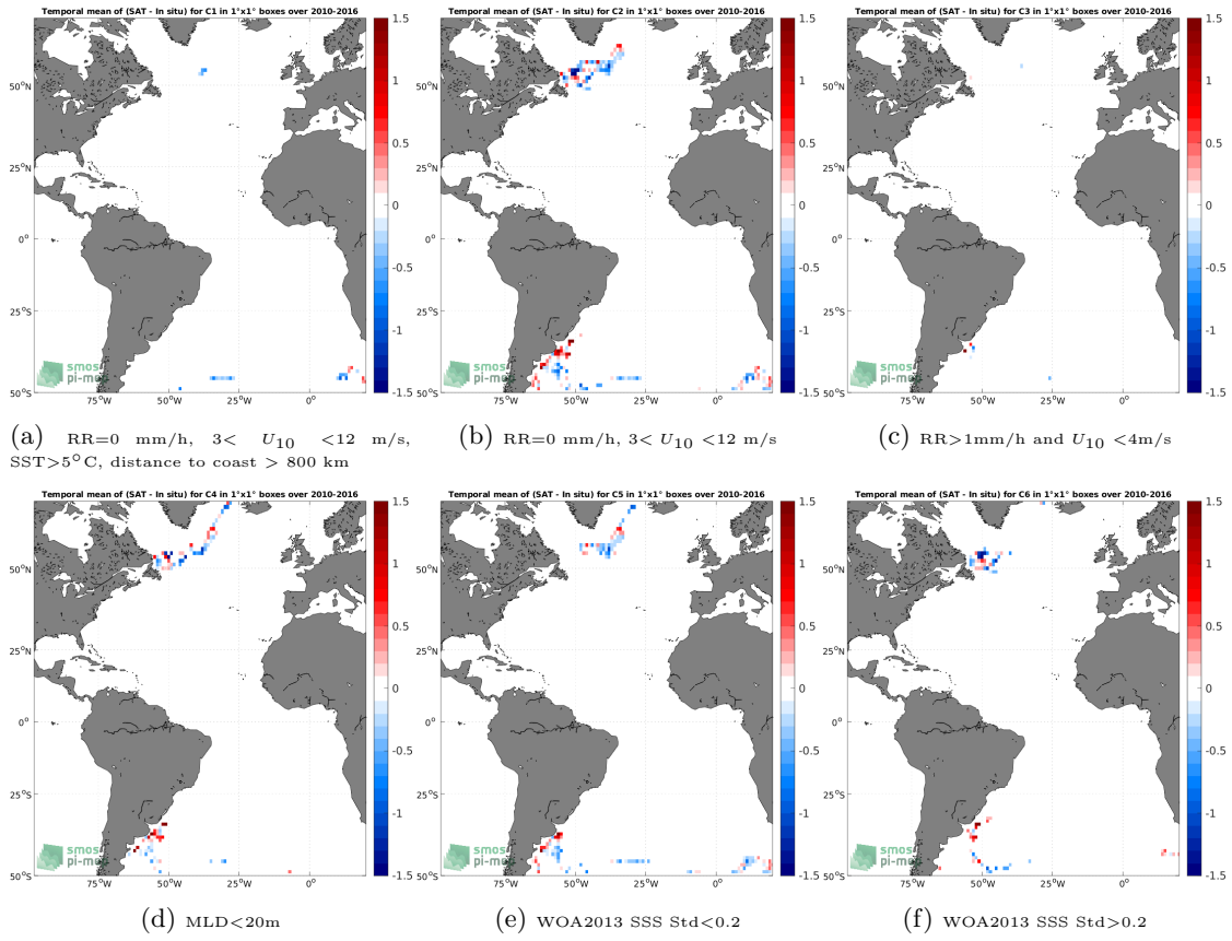
Figure 12: Temporal mean gridded over spatial boxes of size 1^\circ \times 1^\circ of \Delta SSS (SMOS SSS L3 v7 - 9 Days (CATDS-CECOS-LOCEAN) - Marine mammals) for 6 different subdatasets corresponding to:RR=0 mm/h, 3 < U_{10} < 12 m/s, SST>5°C, distance to coast > 800 km (a), RR=0 mm/h, 3 < U_{10} < 12 m/s (b), RR>1mm/h and U_{10} < 4 m/s (c),MLD<20m (d),WOA2013 SSS Std<0.2 (e),WOA2013 SSS Std>0.2 (f).
