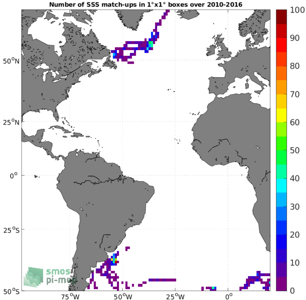
Figure 4: Number of SSS match-ups between Marine mammals SSS and the SMOS SSS L3 v7 - 9 Days (CATDS-CECOS-LOCEAN) SSS product for the Atlantic Ocean Pi-MEP region over 1^\circ \times 1^\circ boxes and for the full satellite product period.
