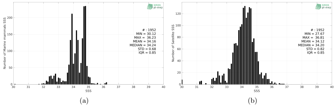
Figure 2: Histograms of SSS from Marine mammals (a) and SMOS SSS L3 v7 - 9 Days (CATDS-CECOS-LOCEAN) (b) considering all match-up pairs per bins of 0.1 over the Atlantic Ocean Pi-MEP region and for the full satellite product period.
