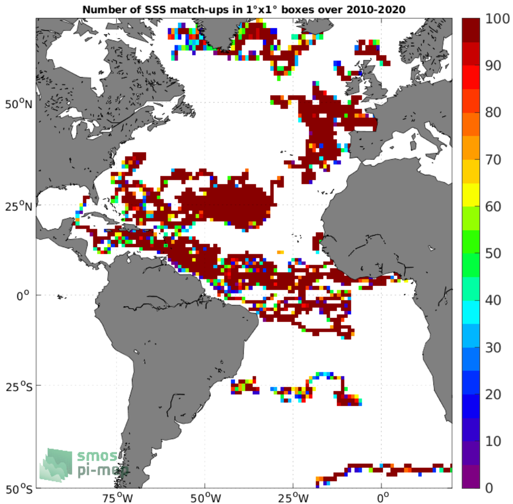
Figure 3: Number of SSS match-ups between Surface drifters SSS and the SMOS SSS L3 v7 - 9 Days (CATDS-CECOS-LOCEAN) SSS product for the Atlantic Ocean Pi-MEP region over 1^\circ \times 1^\circ boxes and for the full satellite product period.
