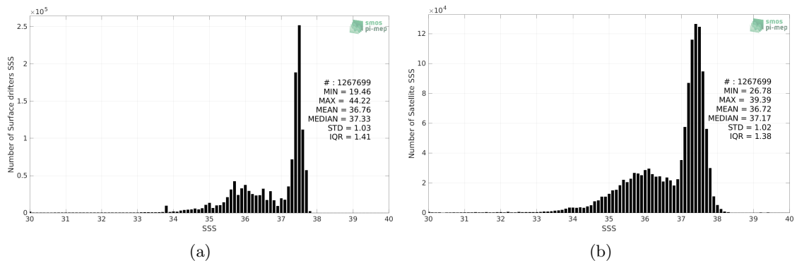
Figure 2: Histograms of SSS from Surface drifters (a) and SMOS SSS L3 v7 - 9 Days (CATDS-CECOS-LOCEAN) (b) considering all match-up pairs per bins of 0.1 over the Atlantic Ocean Pi-MEP region and for the full satellite product period.
