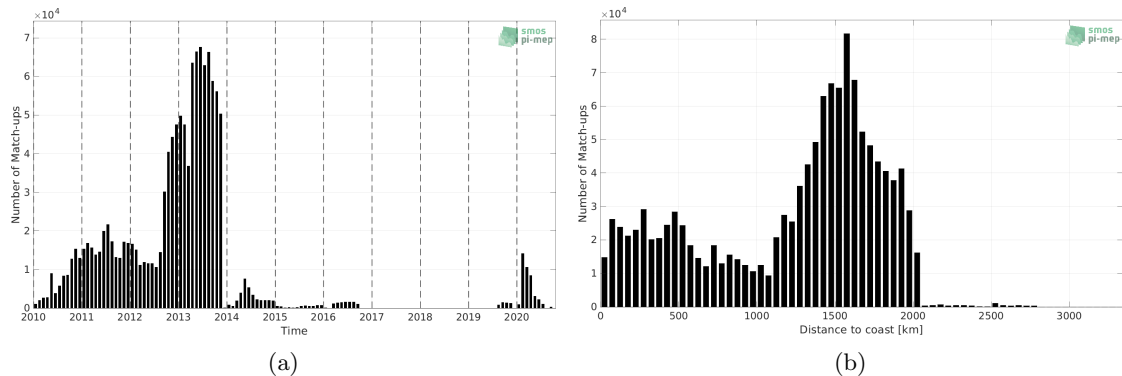
Figure 1: Number of match-ups between Surface drifters and SMOS SSS L3 v7 - 9 Days (CATDS-CECOS-LOCEAN) SSS as a function of time (a) and as function of the distance to coast (b) over the Atlantic Ocean Pi-MEP region and for the full satellite product period.
