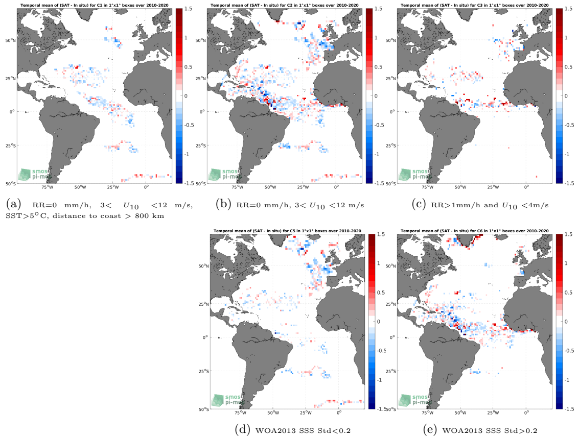
Figure 11: Temporal mean gridded over spatial boxes of size 1^\circ \times 1^\circ of \Delta SSS (SMOS SSS L3 v7 - 9 Days (CATDS-CECOS-LOCEAN) - Surface drifters) for 5 different subdatasets corresponding to:RR=0 mm/h, 3 < U_{10} < 12 m/s, SST >5^\circ\text{C} , distance to coast > 800 km (a), RR=0 mm/h, 3 < U_{10} < 12 m/s (b), RR >1 mm/h and U_{10} < 4 m/s (c), WOA2013 SSS Std <0.2 (d), WOA2013 SSS Std >0.2 (e).
