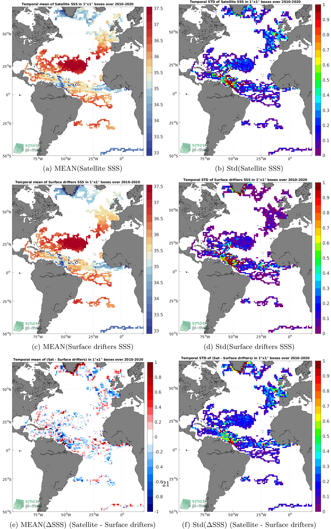
(e) MEAN( \Delta SSS) (Satellite - Surface drifters) (f) Std( \Delta SSS) (Satellite - Surface drifters) Figure 5: Temporal mean (left) and Std (right) of SSS from SMOS SSS L3 v7 - 9 Days (CATDS-CECOS-LOCEAN) (top), Surface drifters (middle), and of \Delta SSS (Satellite - Surface drifters). Only match-up pairs are used to generate these maps.
