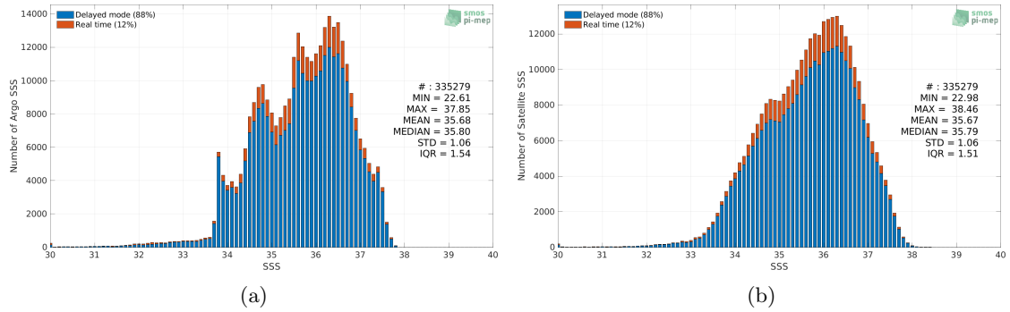
Figure 2: Histograms of SSS from Argo (a) and SMOS SSS L3 v7 - 9 Days (CATDS-CECOS-LOCEAN) (b) considering all match-up pairs per bins of 0.1 over the Atlantic Ocean Pi-MEP region and for the full satellite product period.
