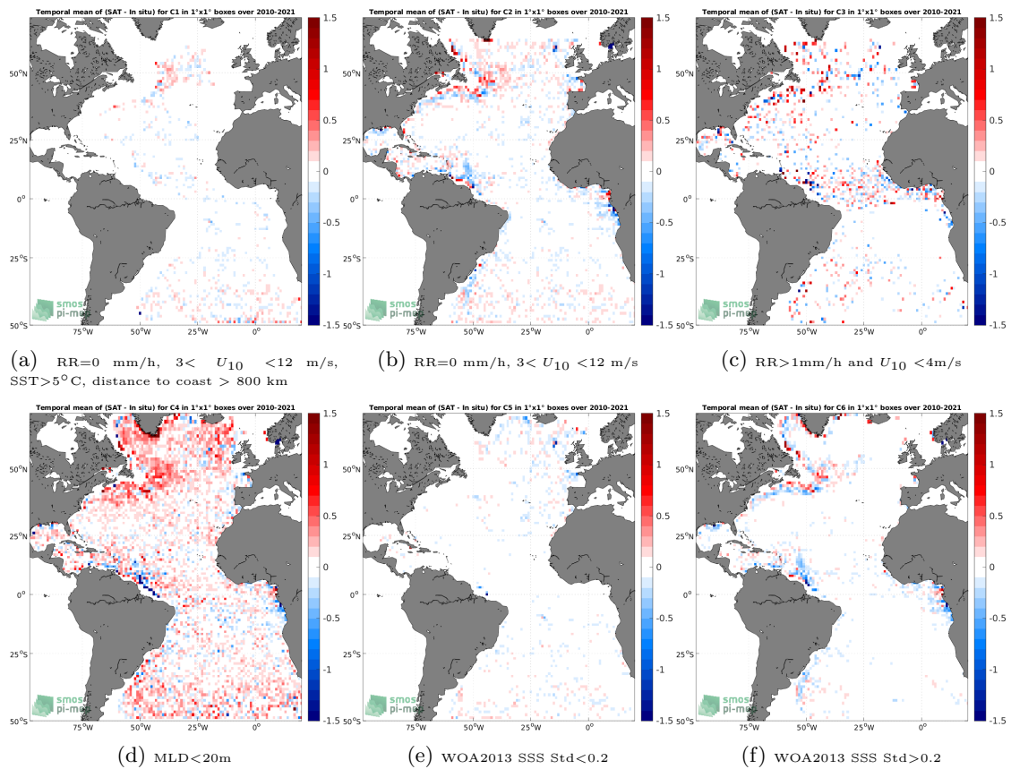
Figure 12: Temporal mean gridded over spatial boxes of size 1^\circ \times 1^\circ of \Delta SSS (SMOS SSS L3 v7 - 9 Days (CATDS-CECOS-LOCEAN) - Argo) for 6 different subdatasets corresponding to:RR=0 mm/h, 3 < U_{10} < 12 m/s, SST > 5^\circ\text{C} , distance to coast > 800 km (a), RR=0 mm/h, 3 < U_{10} < 12 m/s (b), RR > 1 mm/h and U_{10} < 4 m/s (c),MLD < 20 m (d),WOA2013 SSS Std < 0.2 (e),WOA2013 SSS Std > 0.2 (f).
