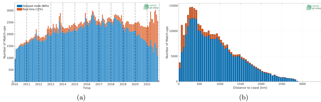
Figure 1: Number of match-ups between Argo and SMOS SSS L3 v7 - 9 Days (CATDS-CECOS-LOCEAN) SSS as a function of time (a) and as function of the distance to coast (b) over the Atlantic Ocean Pi-MEP region and for the full satellite product period.
