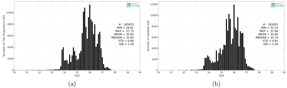
Figure 2: Histograms of SSS from TSG (Polarstern) (a) and SMOS SSS L3 v7 - 18 Days (CATDS-CECOS-LOCEAN) (b) considering all match-up pairs per bins of 0.1 over the Atlantic Ocean Pi-MEP region and for the full satellite product period.
