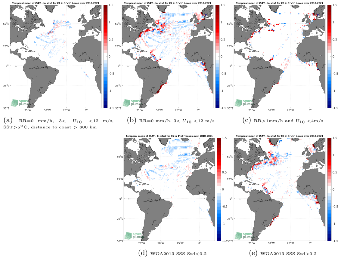
Figure 12: Temporal mean gridded over spatial boxes of size 1^\circ \times 1^\circ of \Delta\text{SSS} (SMOS SSS L3 v7 - 18 Days (CATDS-CECOS-LOCEAN) - TSG (LEGOS-DM)) for 5 different subdatasets corresponding to:RR=0 mm/h, 3 < U_{10} < 12 m/s, SST >5^\circ\text{C} , distance to coast > 800 km (a), RR=0 mm/h, 3 < U_{10} < 12 m/s (b), RR >1 mm/h and U_{10} < 4 m/s (c), WOA2013 SSS Std <0.2 (d), WOA2013 SSS Std >0.2 (e).
