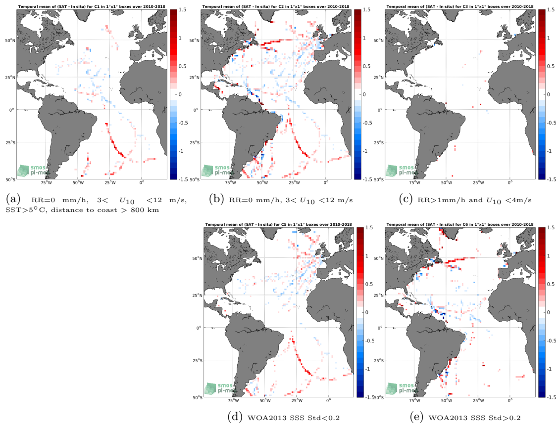
Figure 12: Temporal mean gridded over spatial boxes of size 1^\circ \times 1^\circ of \Delta SSS (SMOS SSS L3 v7 - 18 Days (CATDS-CECOS-LOCEAN) - TSG (GOSUD-Sailing-ship)) for 5 different subdatasets corresponding to:RR=0 mm/h, 3 < U_{10} < 12 m/s, SST>5°C, distance to coast > 800 km (a), RR=0 mm/h, 3 < U_{10} < 12 m/s (b), RR>1mm/h and U_{10} < 4 m/s (c), WOA2013 SSS Std<0.2 (d), WOA2013 SSS Std>0.2 (e).
