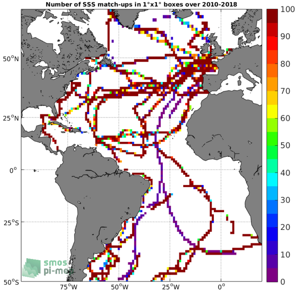
Figure 4: Number of SSS match-ups between TSG (GOSUD-Sailing-ship) SSS and the SMOS SSS L3 v7 - 18 Days (CATDS-CECOS-LOCEAN) SSS product for the Atlantic Ocean Pi-MEP region over 1^\circ \times 1^\circ boxes and for the full satellite product period.
