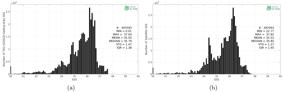
Figure 2: Histograms of SSS from TSG (GOSUD-Sailing-ship) (a) and SMOS SSS L3 v7 - 18 Days (CATDS-CECOS-LOCEAN) (b) considering all match-up pairs per bins of 0.1 over the Atlantic Ocean Pi-MEP region and for the full satellite product period.
