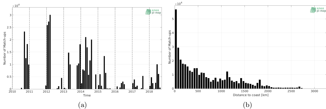
Figure 1: Number of match-ups between TSG (GOSUD-Sailing-ship) and SMOS SSS L3 v7 - 18 Days (CATDS-CECOS-LOCEAN) SSS as a function of time (a) and as function of the distance to coast (b) over the Atlantic Ocean Pi-MEP region and for the full satellite product period.
