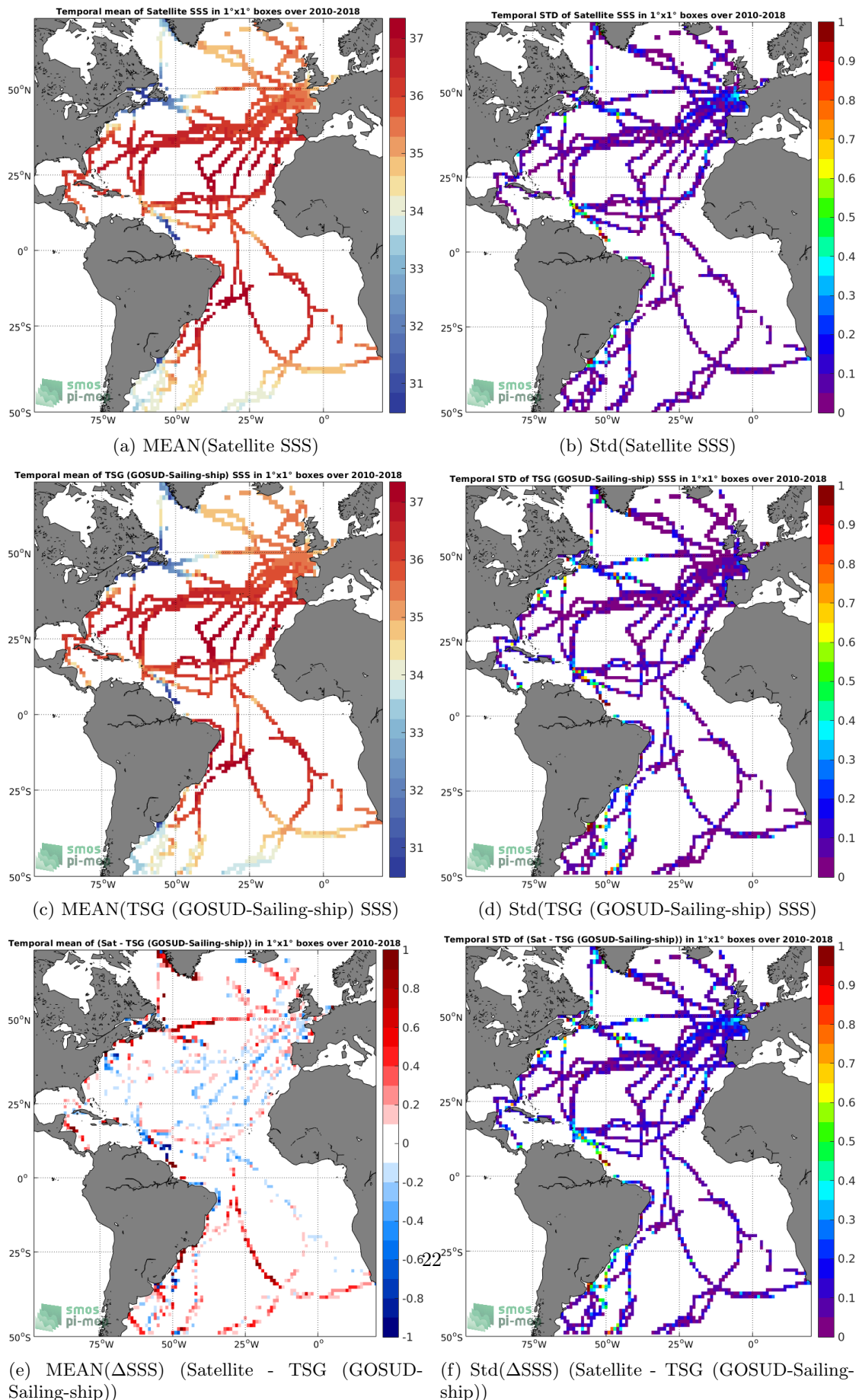
Figure 6: Temporal mean (left) and Std (right) of SSS from SMOS SSS L3 v7 - 18 Days (CATDS-CECOS-LOCEAN) (top), TSG (GOSUD-Sailing-ship) (middle), and of \Delta SSS (Satellite - TSG (GOSUD-Sailing-ship)). Only match-up pairs are used to generate these maps.
