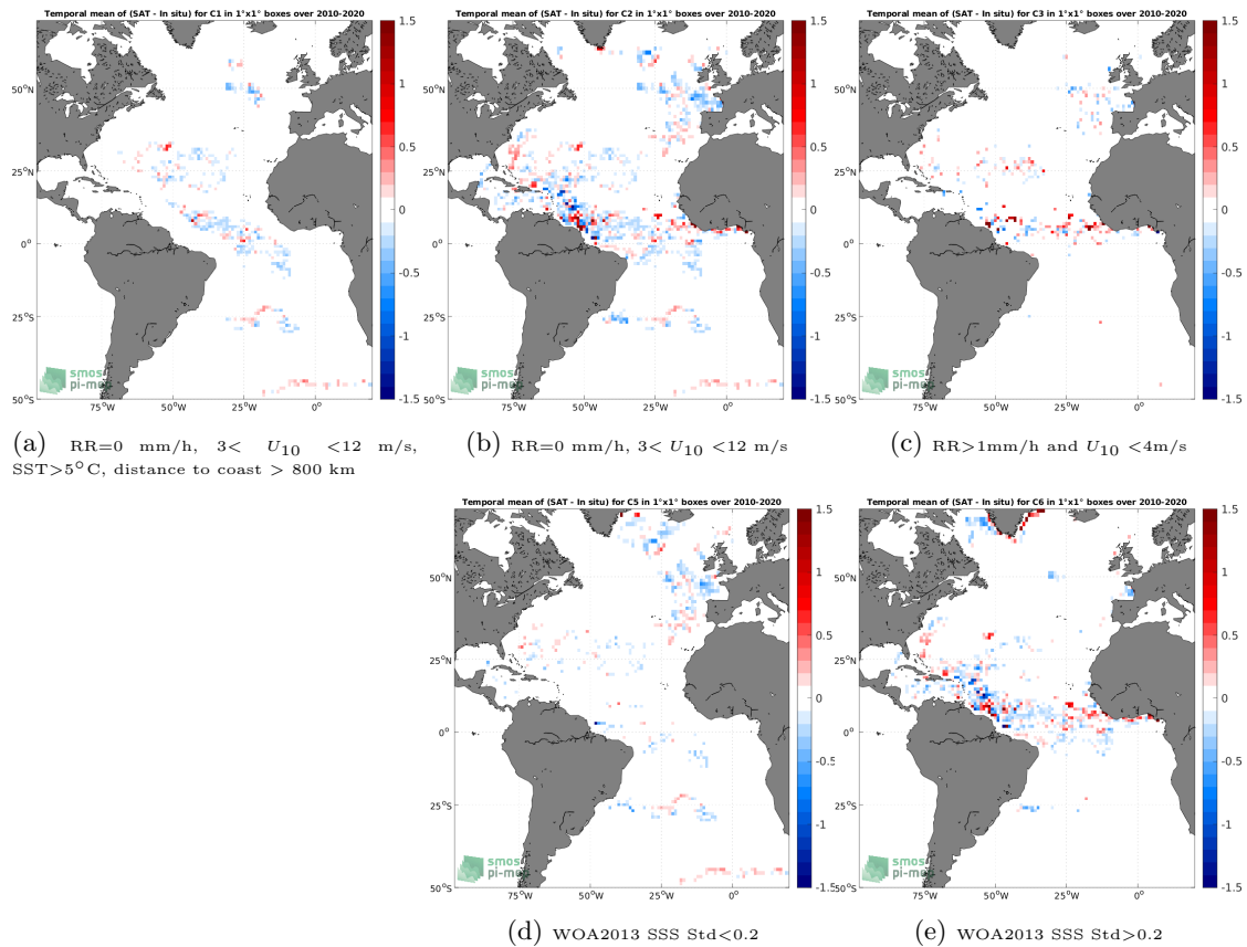
Figure 11: Temporal mean gridded over spatial boxes of size 1^\circ \times 1^\circ of \Delta SSS (SMOS SSS L3 v7 - 18 Days (CATDS-CECOS-LOCEAN) - Surface drifters) for 5 different subdatasets corresponding to:RR=0 mm/h, 3 < U_{10} < 12 m/s, SST >5^\circ\text{C} , distance to coast > 800 km (a), RR=0 mm/h, 3 < U_{10} < 12 m/s (b), RR >1 mm/h and U_{10} < 4 m/s (c), WOA2013 SSS Std <0.2 (d), WOA2013 SSS Std >0.2 (e).
