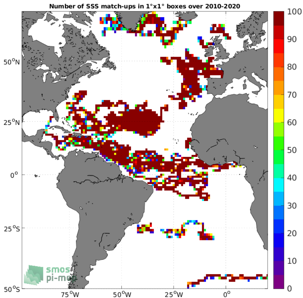
Figure 3: Number of SSS match-ups between Surface drifters SSS and the SMOS SSS L3 v7 - 18 Days (CATDS-CECOS-LOCEAN) SSS product for the Atlantic Ocean Pi-MEP region over 1^\circ \times 1^\circ boxes and for the full satellite product period.
