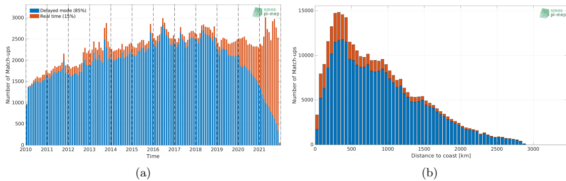
Figure 1: Number of match-ups between Argo and SMOS SSS L3 v7 - 18 Days (CATDS-CECOS-LOCEAN) SSS as a function of time (a) and as function of the distance to coast (b) over the Atlantic Ocean Pi-MEP region and for the full satellite product period.
