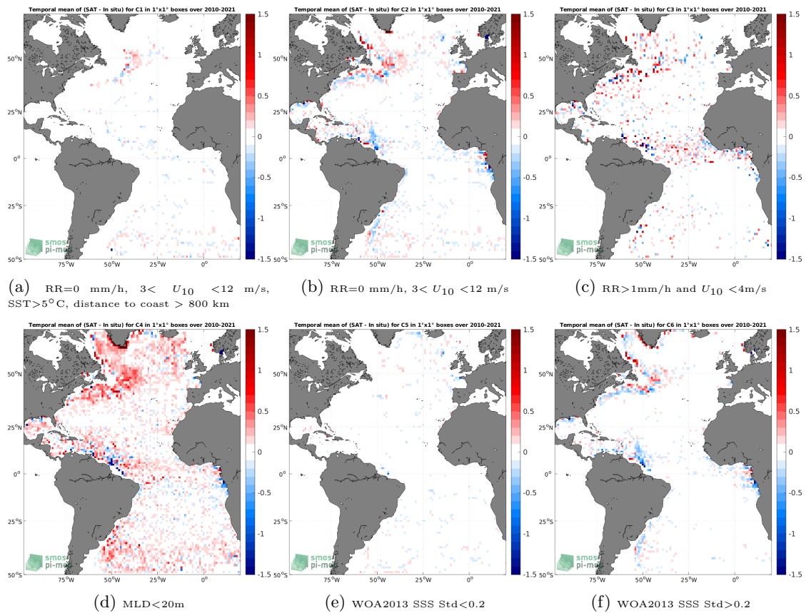
Figure 12: Temporal mean gridded over spatial boxes of size 1^\circ \times 1^\circ of \Delta SSS (SMOS SSS L3 v7 - 18 Days (CATDS-CECOS-LOCEAN) - Argo) for 6 different subdatasets corresponding to:RR=0 mm/h, 3 < U_{10} < 12 m/s, SST>5°C, distance to coast > 800 km (a), RR=0 mm/h, 3 < U_{10} < 12 m/s (b), RR>1mm/h and U_{10} < 4 m/s (c),MLD<20m (d),WOA2013 SSS Std<0.2 (e),WOA2013 SSS Std>0.2 (f).
