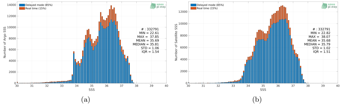
Figure 2: Histograms of SSS from Argo (a) and SMOS SSS L3 v7 - 18 Days (CATDS-CECOS-LOCEAN) (b) considering all match-up pairs per bins of 0.1 over the Atlantic Ocean Pi-MEP region and for the full satellite product period.
