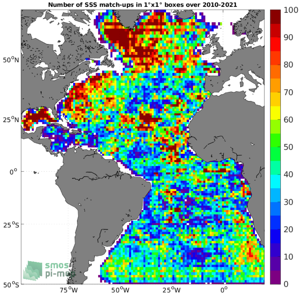
Figure 4: Number of SSS match-ups between Argo SSS and the SMOS SSS L3 v7 - 18 Days (CATDS-CECOS-LOCEAN) SSS product for the Atlantic Ocean Pi-MEP region over 1°x1° boxes and for the full satellite product period.
