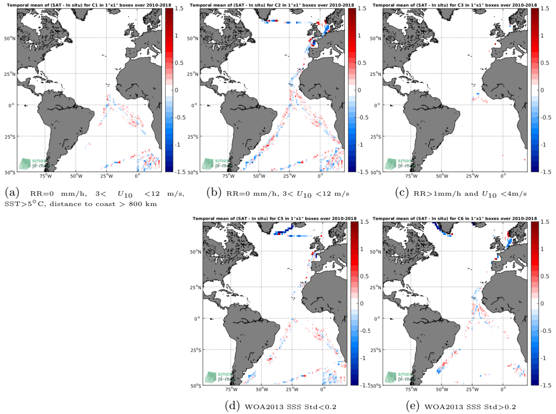
Figure 12: Temporal mean gridded over spatial boxes of size 1^\circ \times 1^\circ of \Delta SSS (SMOS-L3-CATDS-CECOS-LOCEAN-V4-9DAYS-25KM - TSG-POLARSTERN) for 5 different subdatasets corresponding to: RR=0 mm/h, 3 < U_{10} < 12 m/s, SST > 5^\circ C , distance to coast > 800 km (a), RR=0 mm/h, 3 < U_{10} < 12 m/s (b), RR > 1 mm/h and U_{10} < 4 m/s (c), WOA2013 SSS Std < 0.2 (d), WOA2013 SSS Std > 0.2 (e).
