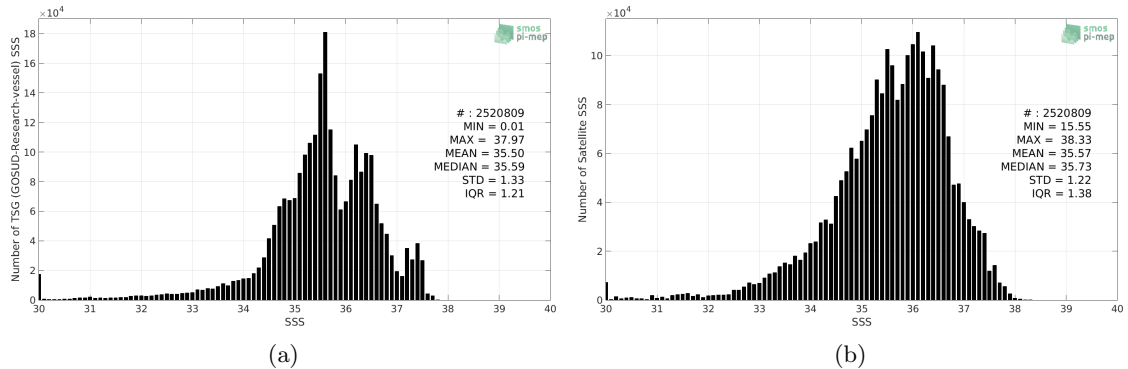
Figure 2: Histograms of SSS from TSG (GOSUD-Research-vessel) (a) and SMOS SSS L3 v4 - 9 Days (CATDS-CECOS-LOCEAN) (b) considering all match-up pairs per bins of 0.1 over the Atlantic Ocean Pi-MEP region and for the full satellite product period.
