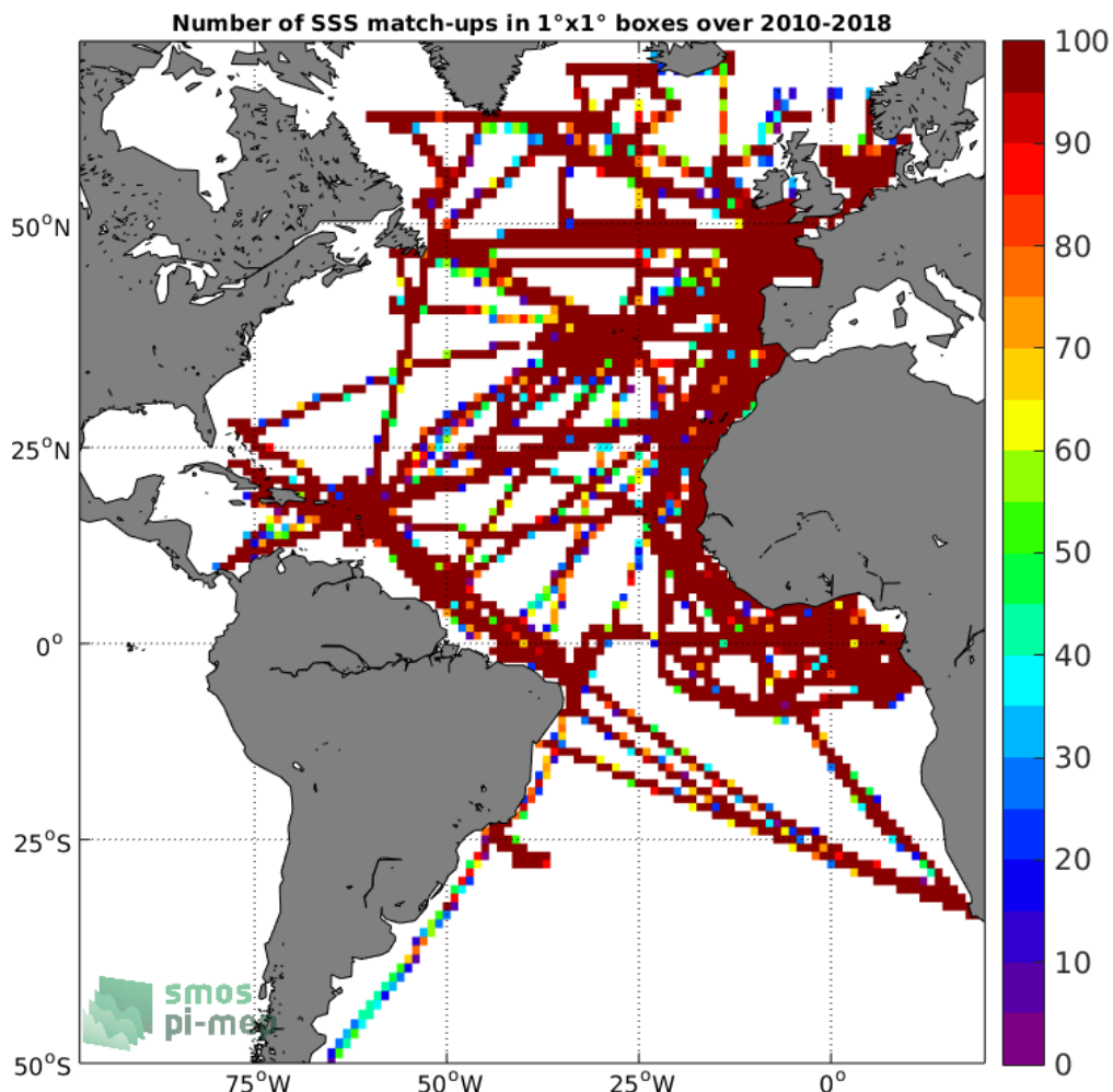
Figure 4: Number of SSS match-ups between TSG (GOSUD-Research-vessel) SSS and the SMOS SSS L3 v4 - 9 Days (CATDS-CECOS-LOCEAN) SSS product for the Atlantic Ocean Pi-MEP region over 1°x1° boxes and for the full satellite product period.
