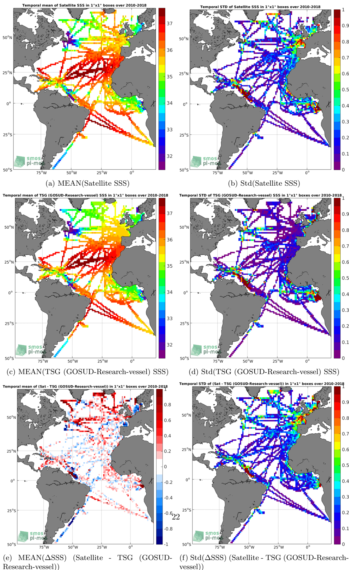
Figure 6: Temporal mean (left) and Std (right) of SSS from SMOS SSS L3 v4 - 9 Days (CATDS-CECOS-LOCEAN) (top), TSG (GOSUD-Research-vessel) (middle), and of \Delta SSS (Satellite - TSG (GOSUD-Research-vessel)). Only match-up pairs are used to generate these maps.
