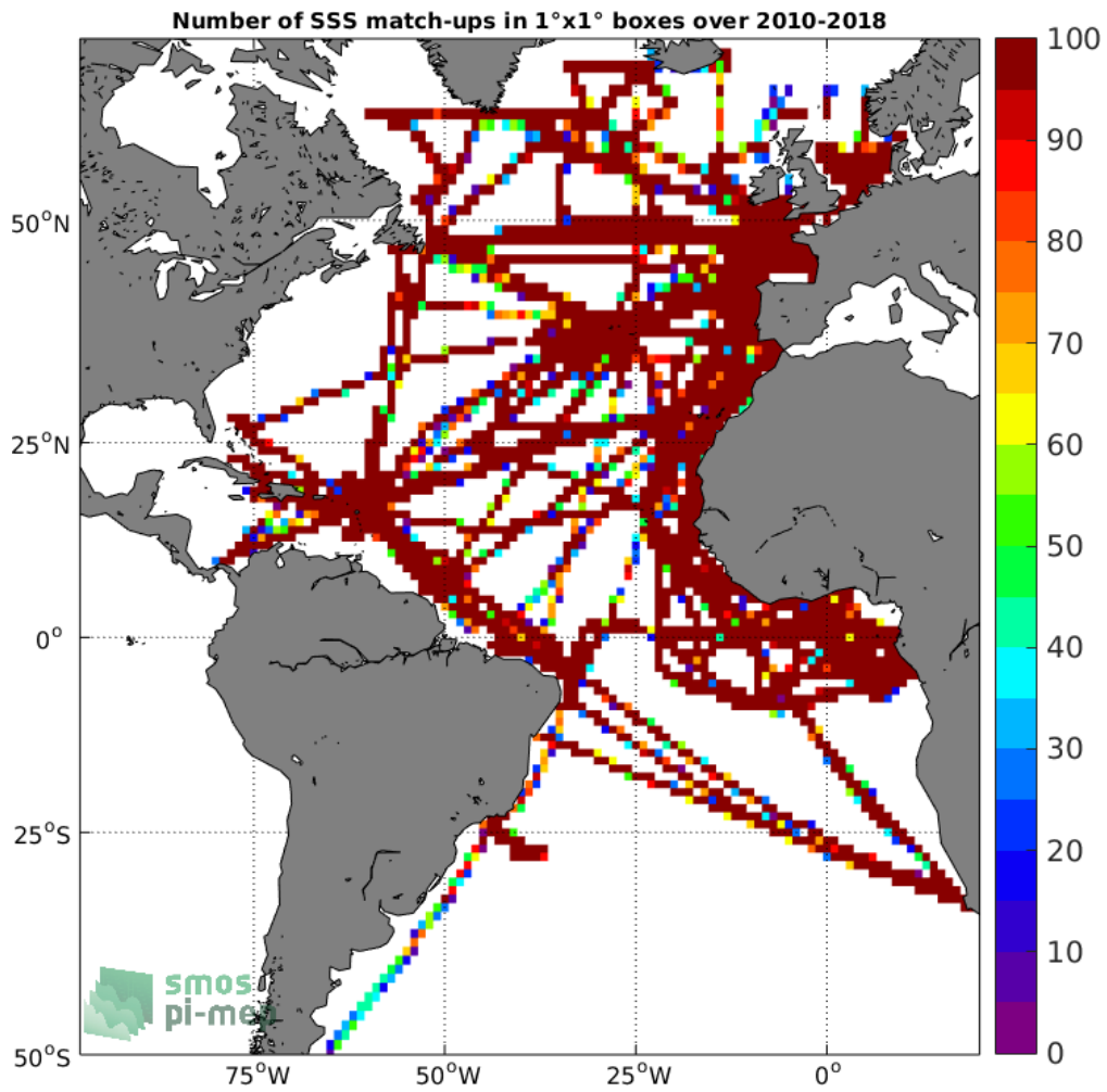
Figure 4: Number of SSS match-ups between TSG-GOSUD-Research-vessel SSS and the SMOS-L3-CATDS-CECOS-LOCEAN-V4-9DAYS-25KM SSS product for the Atlantic Ocean Pi-MEP region over 1°x1° boxes and for the full satellite product period.
