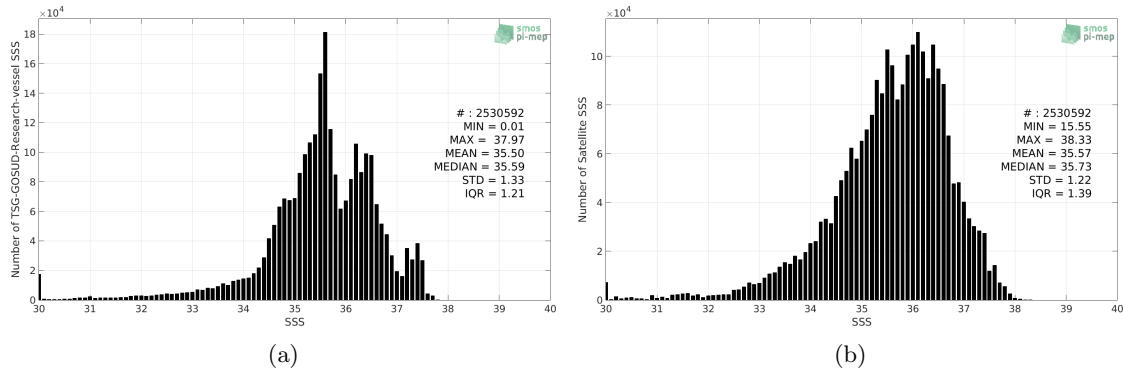
Figure 2: Histograms of SSS from TSG-GOSUD-Research-vessel (a) and SMOS-L3-CATDS-CECOS-LOCEAN-V4-9DAYS-25KM (b) considering all match-up pairs per bins of 0.1 over the Atlantic Ocean Pi-MEP region and for the full satellite product period.
