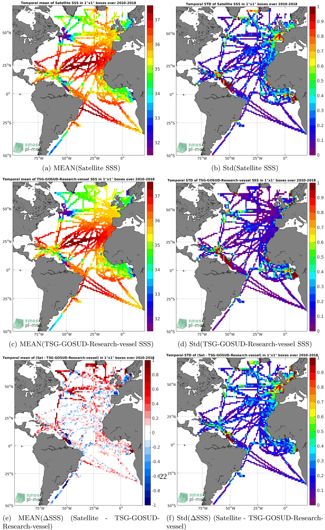
Figure 6: Temporal mean (left) and Std (right) of SSS from SMOS-L3-CATDS-CECOS-LOCEAN-V4-9DAYS-25KM (top), TSG-GOSUD-Research-vessel (middle), and of \Delta SSS (Satellite - TSG-GOSUD-Research-vessel). Only match-up pairs are used to generate these maps.
