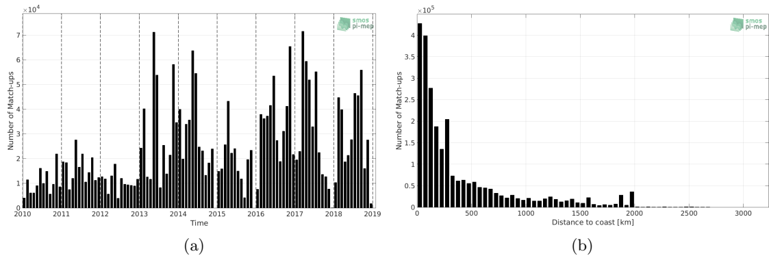
Figure 1: Number of match-ups between TSG-GOSUD-Research-vessel and SMOS-L3-CATDS-CECOS-LOCEAN-V4-9DAYS-25KM SSS as a function of time (a) and as function of the distance to coast (b) over the Atlantic Ocean Pi-MEP region and for the full satellite product period.
