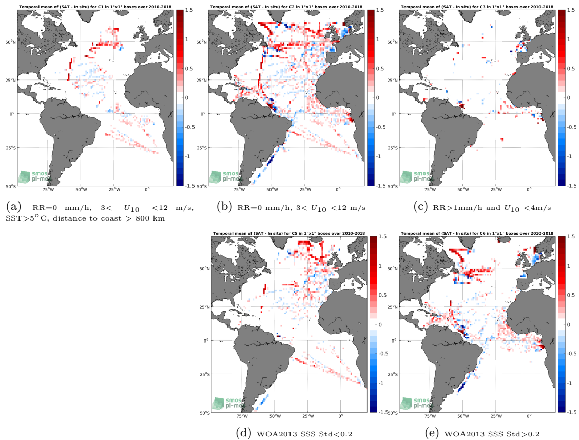
Figure 12: Temporal mean gridded over spatial boxes of size 1^\circ \times 1^\circ of \Delta\text{SSS} (SMOS-L3-CATDS-CECOS-LOCEAN-V4-9DAYS-25KM - TSG-GOSUD-Research-vessel) for 5 different subdatasets corresponding to:RR=0 mm/h, 3 < U_{10} < 12 m/s, SST>5°C, distance to coast > 800 km (a), RR=0 mm/h, 3 < U_{10} < 12 m/s (b), RR>1mm/h and U_{10} < 4 m/s (c), WOA2013 SSS Std<0.2 (d), WOA2013 SSS Std>0.2 (e).
