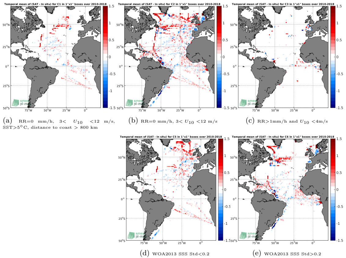
Figure 12: Temporal mean gridded over spatial boxes of size 1^\circ \times 1^\circ of \Delta SSS (SMOS-L3-CATDS-CECOS-LOCEAN-V4-9DAYS-25KM - TSG-GOSUD-Research-vessel) for 5 different subdatasets corresponding to:RR=0 mm/h, 3 < U_{10} < 12 m/s, SST>5°C, distance to coast > 800 km (a), RR=0 mm/h, 3 < U_{10} < 12 m/s (b), RR>1mm/h and U_{10} < 4 m/s (c), WOA2013 SSS Std<0.2 (d), WOA2013 SSS Std>0.2 (e).
