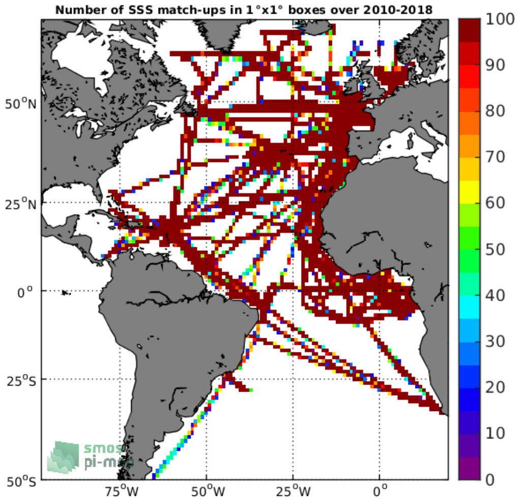
Figure 4: Number of SSS match-ups between TSG-GOSUD-Research-vessel SSS and the SMOS-L3-CATDS-CECOS-LOCEAN-V4-9DAYS-25KM SSS product for the Atlantic Ocean Pi-MEP region over 1°x1° boxes and for the full satellite product period.
