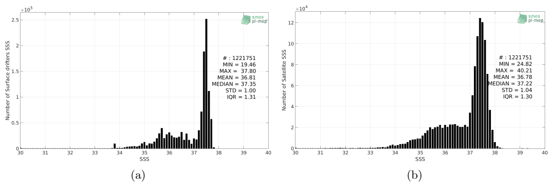
Figure 2: Histograms of SSS from Surface drifters (a) and SMOS SSS L3 v4 - 9 Days (CATDS-CECOS-LOCEAN) (b) considering all match-up pairs per bins of 0.1 over the Atlantic Ocean Pi-MEP region and for the full satellite product period.
