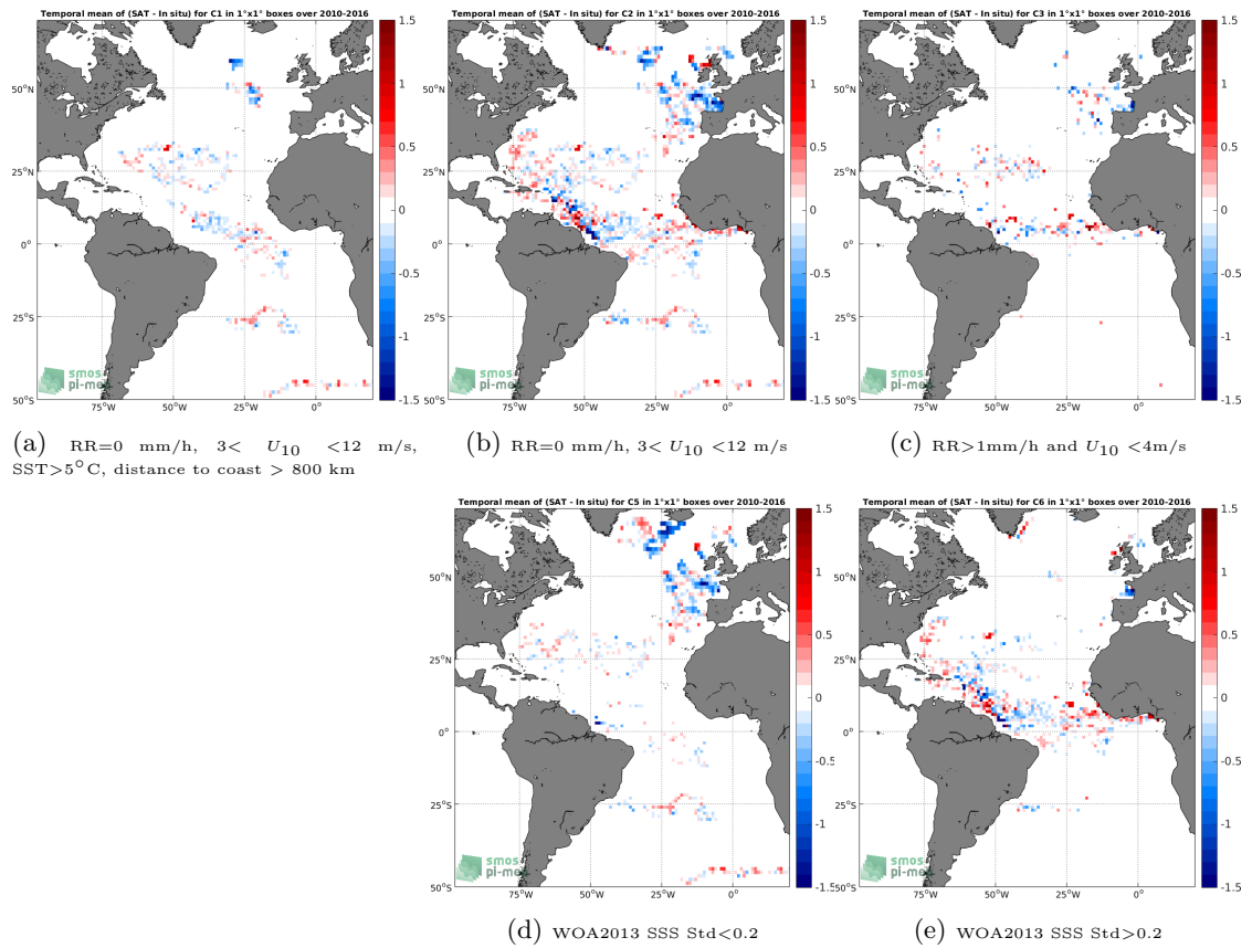
Figure 11: Temporal mean gridded over spatial boxes of size 1^\circ \times 1^\circ of \Delta SSS (SMOS SSS L3 v4 - 9 Days (CATDS-CECOS-LOCEAN) - Surface drifters) for 5 different subdatasets corresponding to:RR=0 mm/h, 3 < U_{10} < 12 m/s, SST >5^\circ\text{C} , distance to coast > 800 km (a), RR=0 mm/h, 3 < U_{10} < 12 m/s (b), RR >1 mm/h and U_{10} < 4 m/s (c), WOA2013 SSS Std <0.2 (d), WOA2013 SSS Std >0.2 (e).
