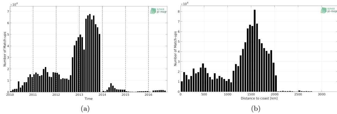
Figure 1: Number of match-ups between Surface drifters and SMOS SSS L3 v4 - 9 Days (CATDS-CECOS-LOCEAN) SSS as a function of time (a) and as function of the distance to coast (b) over the Atlantic Ocean Pi-MEP region and for the full satellite product period.
