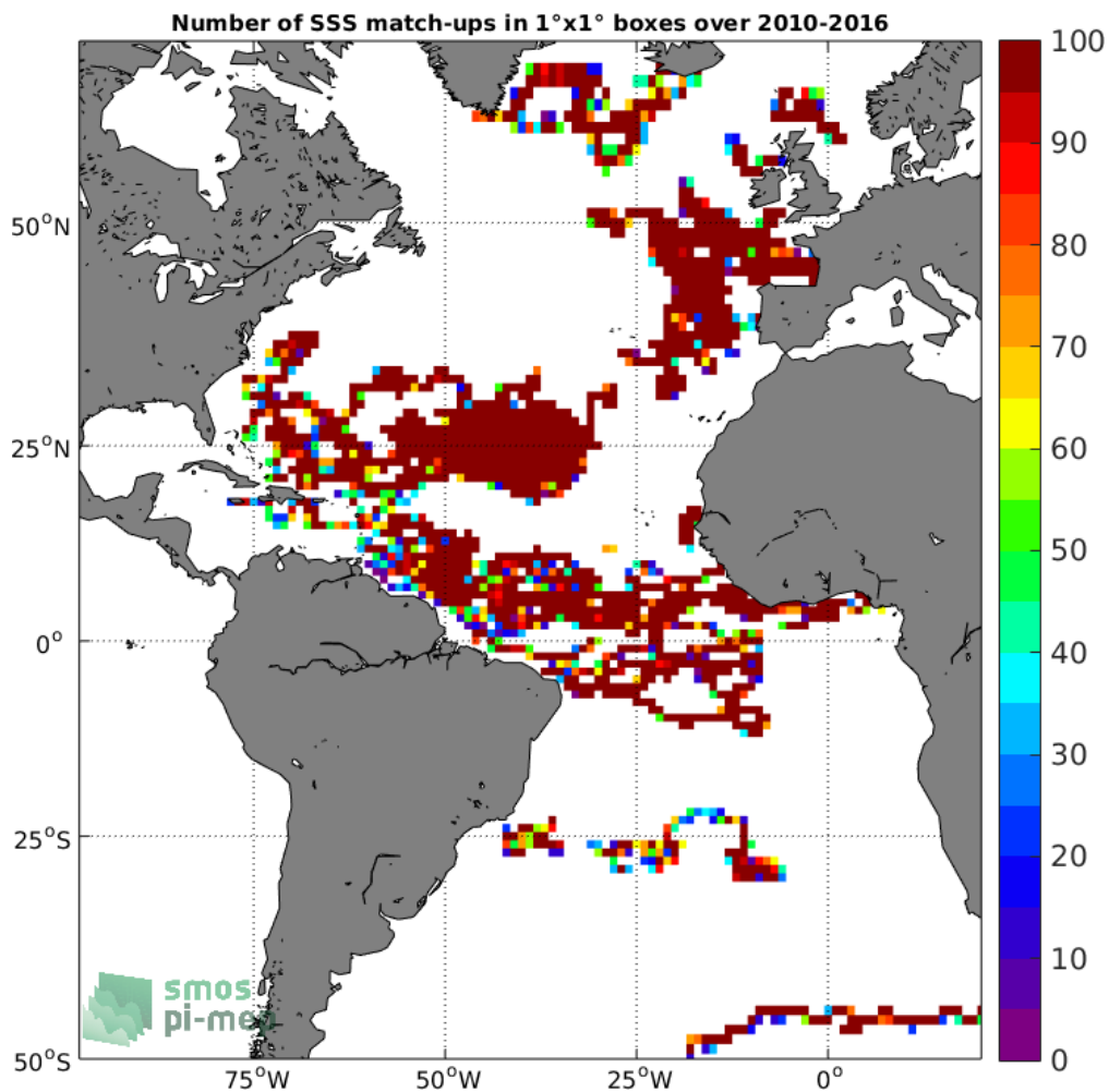
Figure 3: Number of SSS match-ups between Surface drifters SSS and the SMOS SSS L3 v4 - 9 Days (CATDS-CECOS-LOCEAN) SSS product for the Atlantic Ocean Pi-MEP region over 1°x1° boxes and for the full satellite product period.
