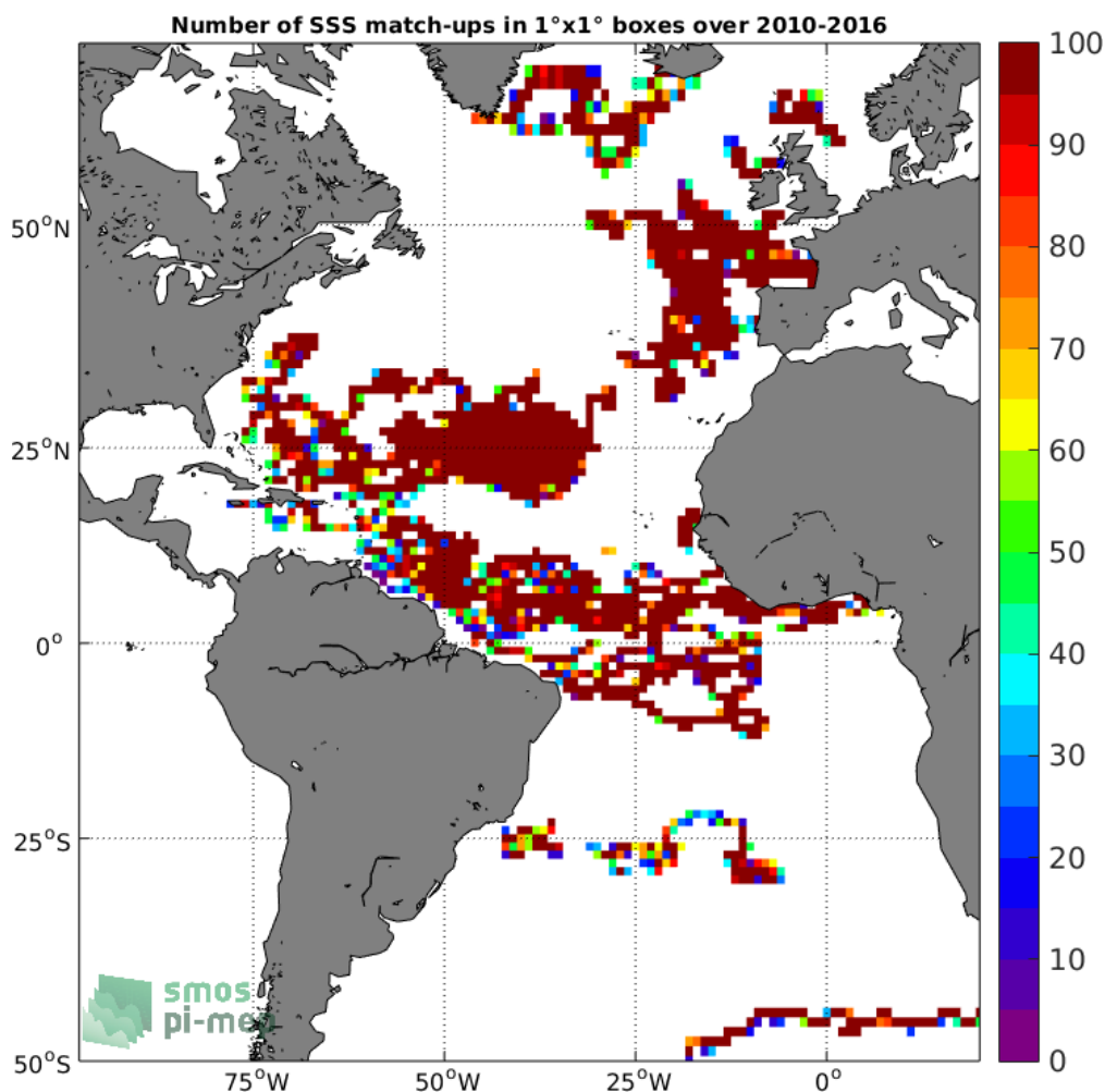
Figure 3: Number of SSS match-ups between Surface drifters SSS and the SMOS-L3-CATDS-CECOS-LOCEAN-V4-9DAYS-25KM SSS product for the Atlantic Ocean Pi-MEP region over 1°x1° boxes and for the full satellite product period.
