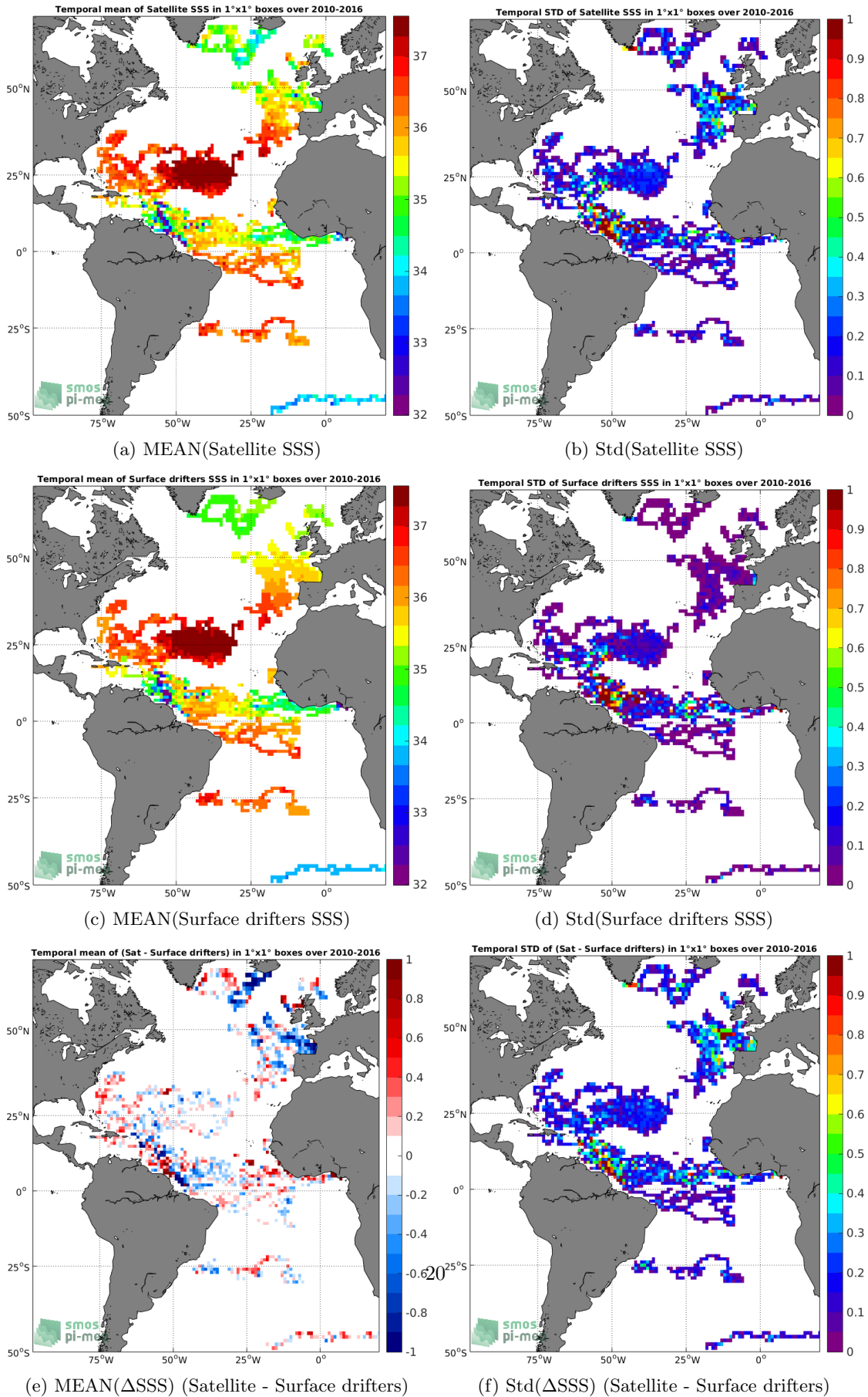
Figure 5: Temporal mean (left) and Std (right) of SSS from SMOS-L3-CATDS-CECOS-LOCEAN-V4-9DAYS-25KM (top), Surface drifters (middle), and of \Delta SSS (Satellite - Surface drifters). Only match-up pairs are used to generate these maps.
