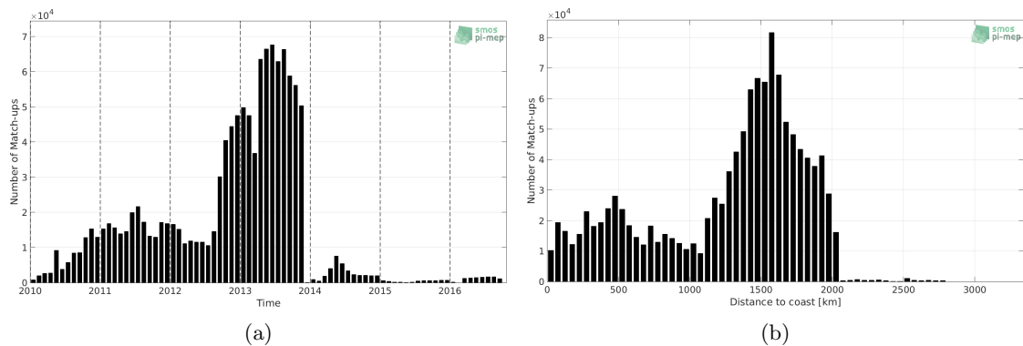
Figure 1: Number of match-ups between Surface drifters and SMOS-L3-CATDS-CECOS-LOCEAN-V4-9DAYS-25KM SSS as a function of time (a) and as function of the distance to coast (b) over the Atlantic Ocean Pi-MEP region and for the full satellite product period.
