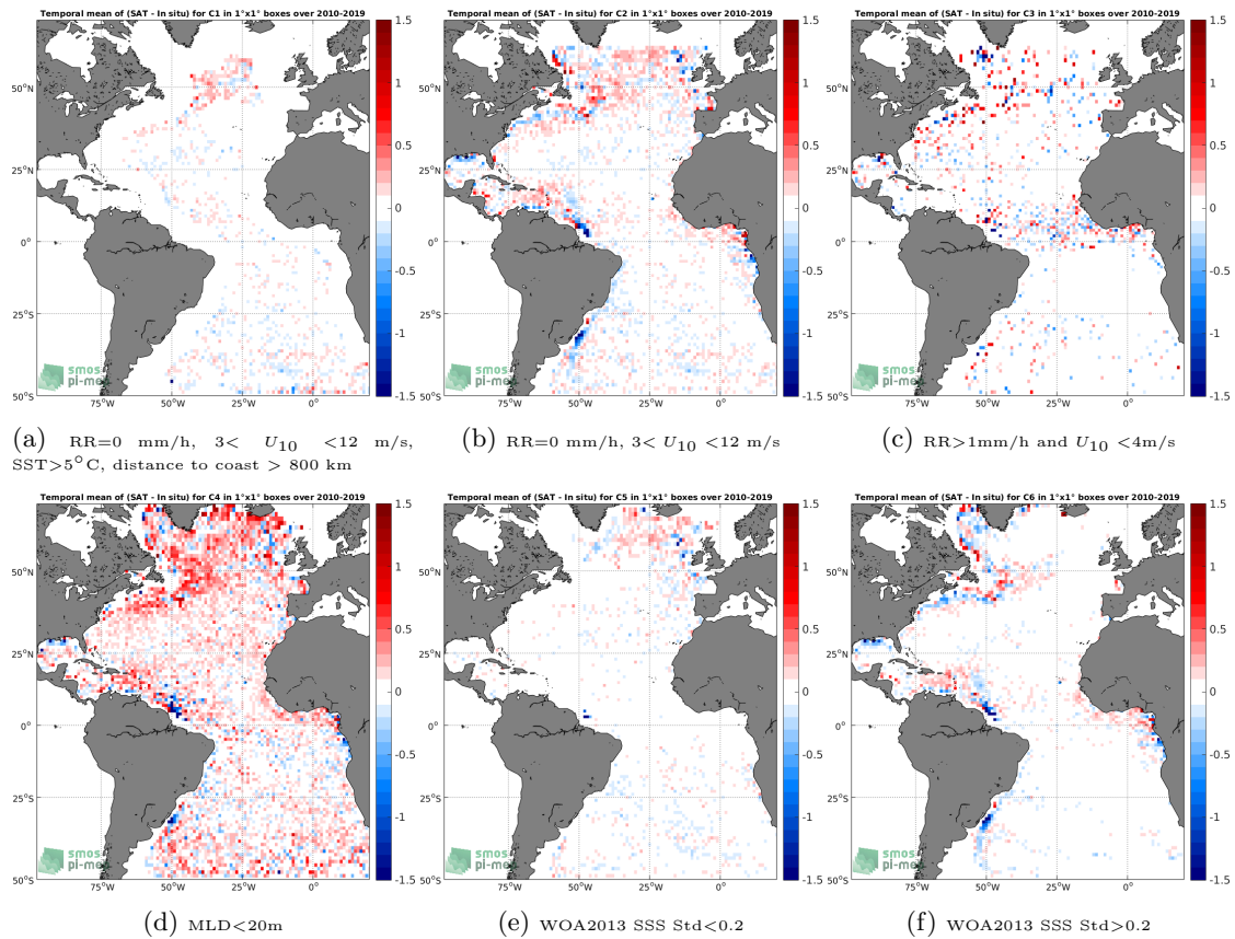
Figure 12: Temporal mean gridded over spatial boxes of size 1^\circ \times 1^\circ of \Delta SSS (SMOS SSS L3 v4 - 9 Days (CATDS-CECOS-LOCEAN) - Argo) for 6 different subdatasets corresponding to:RR=0 mm/h, 3 < U_{10} < 12 m/s, SST >5^\circ C, distance to coast > 800 km (a), RR=0 mm/h, 3 < U_{10} < 12 m/s (b), RR >1 mm/h and U_{10} < 4 m/s (c),MLD <20 m (d),WOA2013 SSS Std <0.2 (e),WOA2013 SSS Std >0.2 (f).
