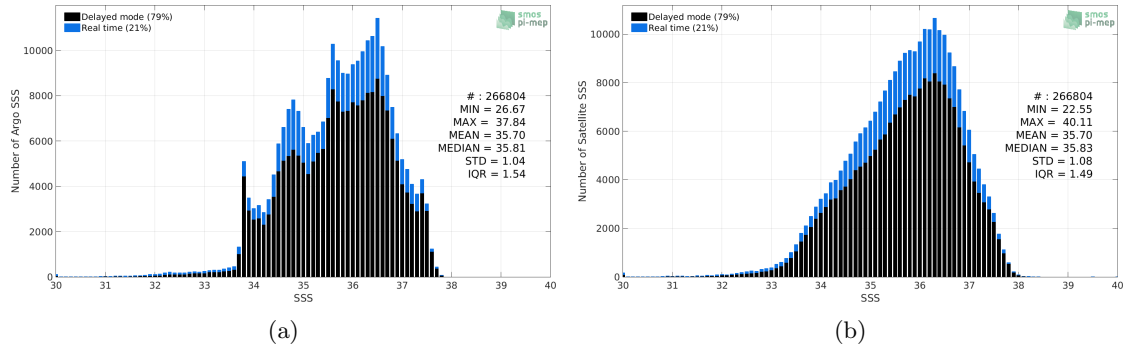
Figure 2: Histograms of SSS from Argo (a) and SMOS SSS L3 v4 - 9 Days (CATDS-CECOS-LOCEAN) (b) considering all match-up pairs per bins of 0.1 over the Atlantic Ocean Pi-MEP region and for the full satellite product period.
