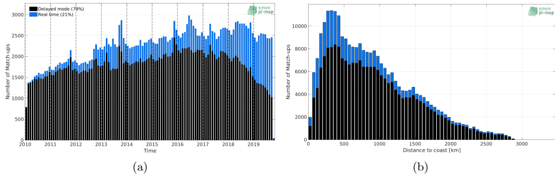
Figure 1: Number of match-ups between Argo and SMOS SSS L3 v4 - 9 Days (CATDS-CECOS-LOCEAN) SSS as a function of time (a) and as function of the distance to coast (b) over the Atlantic Ocean Pi-MEP region and for the full satellite product period.
