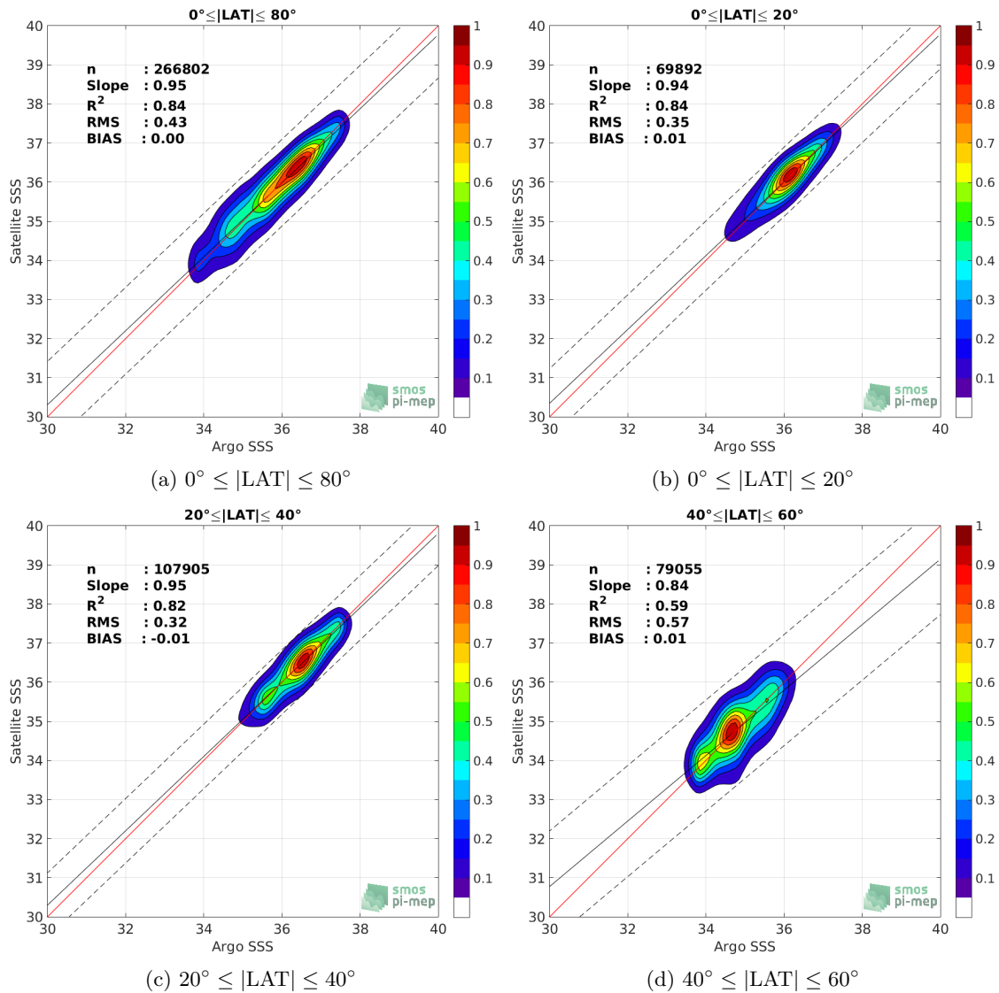
Figure 9: Contour maps of the concentration of SMOS SSS v4 - 9 Days (CATDS-CECOS-LOCEAN) SSS (y-axis) versus Argo SSS (x-axis) at match-up pairs for different latitude bands. For each plot, the red line shows x=y . The black thin and dashed lines indicate a linear fit through the data cloud and the \pm 95\% confidence levels, respectively. The number match-up pairs n , the slope and R^2 coefficient of the linear fit, the root mean square (RMS) and the mean bias between satellite and in situ data are indicated for each latitude band in each plots.
