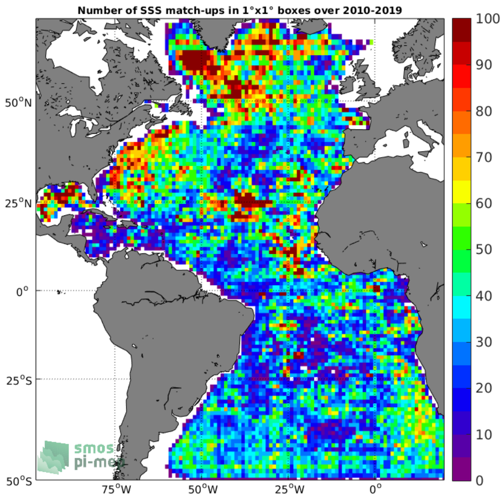
Figure 4: Number of SSS match-ups between Argo SSS and the SMOS SSS L3 v4 - 9 Days (CATDS-CECOS-LOCEAN) SSS product for the Atlantic Ocean Pi-MEP region over 1°x1° boxes and for the full satellite product period.
