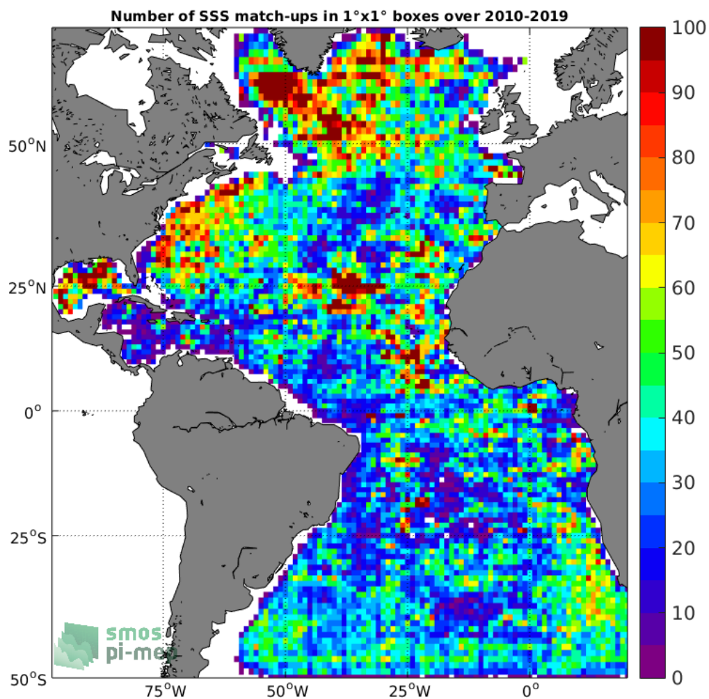
Figure 4: Number of SSS match-ups between Argo SSS and the SMOS-L3-CATDS-CECOS-LOCEAN-V4-9DAYS-25KM SSS product for the Atlantic Ocean Pi-MEP region over 1°x1° boxes and for the full satellite product period.
