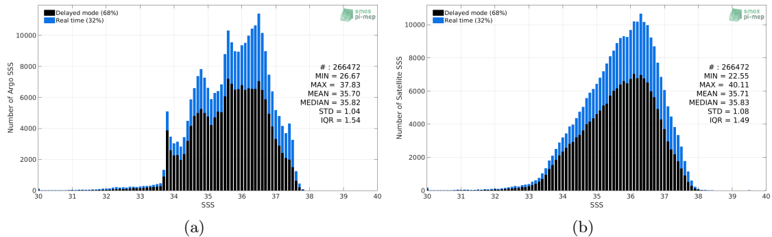
Figure 2: Histograms of SSS from Argo (a) and SMOS-L3-CATDS-CECOS-LOCEAN-V4-9DAYS-25KM (b) considering all match-up pairs per bins of 0.1 over the Atlantic Ocean Pi-MEP region and for the full satellite product period.
