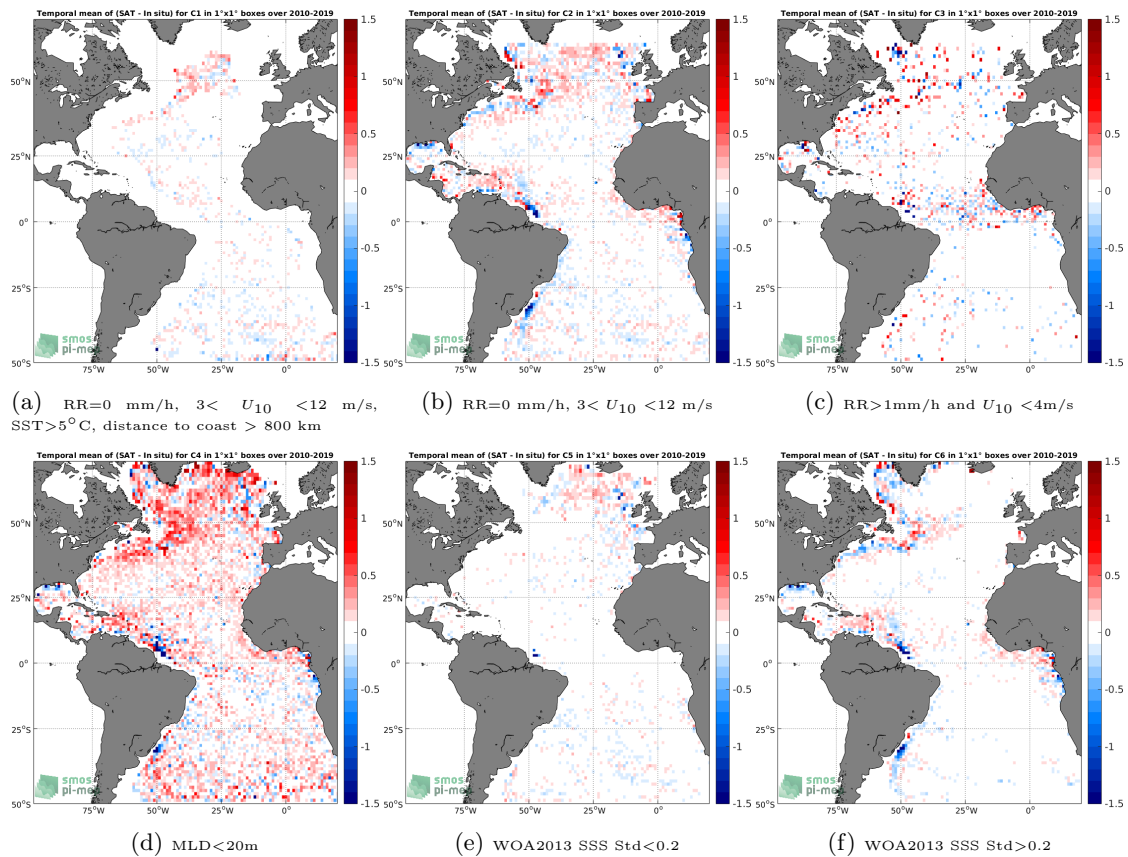
Figure 12: Temporal mean gridded over spatial boxes of size 1^\circ \times 1^\circ of \Delta SSS (SMOS-L3-CATDS-CECOS-LOCEAN-V4-9DAYS-25KM - Argo) for 6 different subdatasets corresponding to:RR=0 mm/h, 3 < U_{10} < 12 m/s, SST >5^\circ C, distance to coast > 800 km (a), RR=0 mm/h, 3 < U_{10} < 12 m/s (b), RR >1 mm/h and U_{10} < 4 m/s (c),MLD <20 m (d),WOA2013 SSS Std <0.2 (e),WOA2013 SSS Std >0.2 (f).
