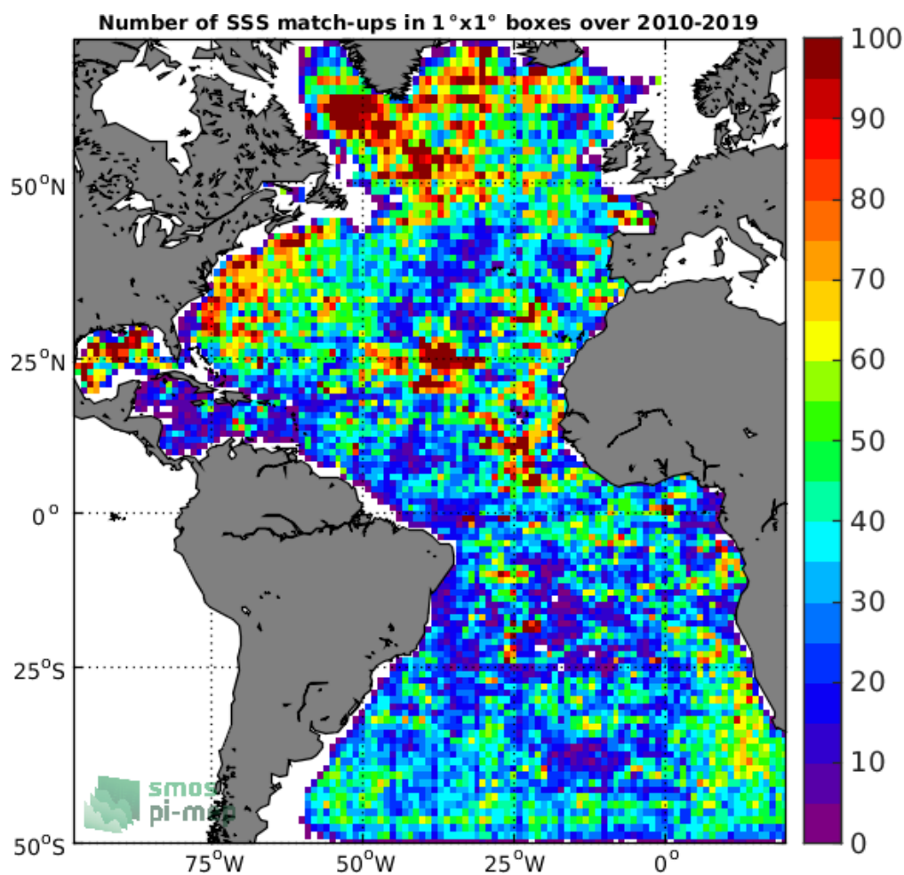
Figure 4: Number of SSS match-ups between Argo SSS and the SMOS-L3-CATDS-CECOS-LOCEAN-V4-9DAYS-25KM SSS product for the Atlantic Ocean Pi-MEP region over 1°x1° boxes and for the full satellite product period.
