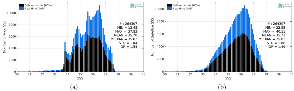
Figure 2: Histograms of SSS from Argo (a) and SMOS-L3-CATDS-CECOS-LOCEAN-V4-9DAYS-25KM (b) considering all match-up pairs per bins of 0.1 over the Atlantic Ocean Pi-MEP region and for the full satellite product period.
