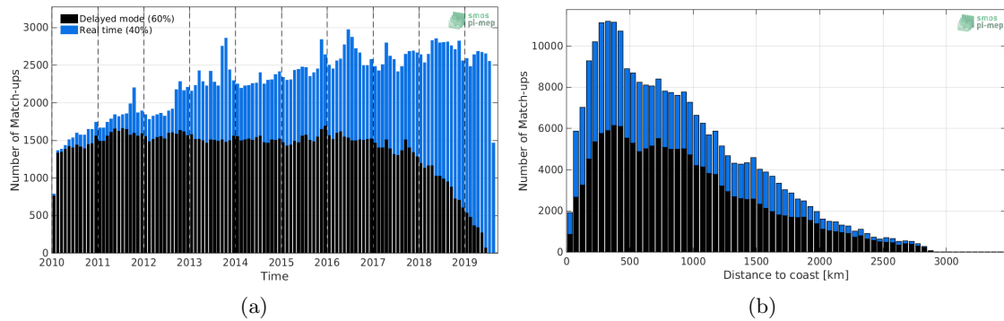
Figure 1: Number of match-ups between Argo and SMOS-L3-CATDS-CECOS-LOCEAN-V4-9DAYS-25KM SSS as a function of time (a) and as function of the distance to coast (b) over the Atlantic Ocean Pi-MEP region and for the full satellite product period.
