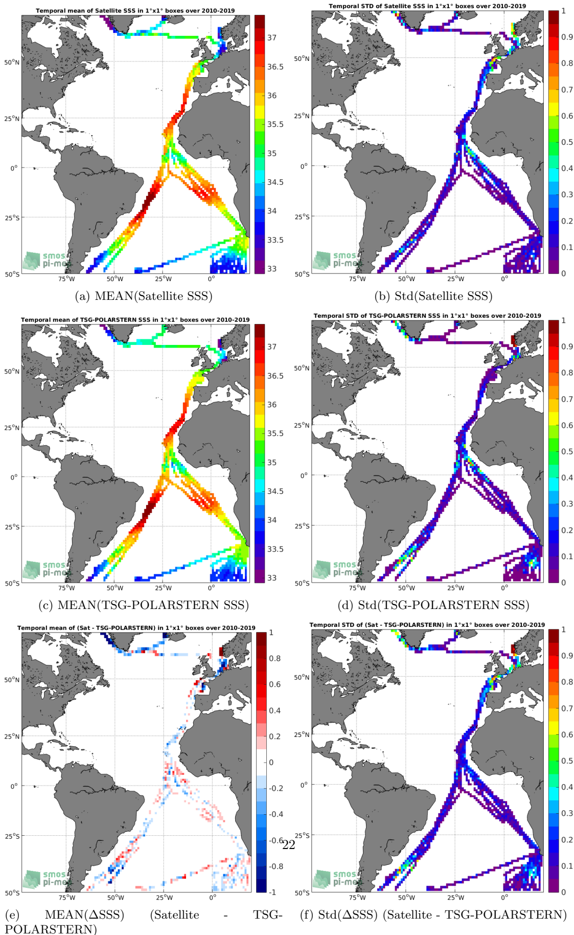
Figure 6: Temporal mean (left) and Std (right) of SSS from SMOS-L3-CATDS-CECOS-LOCEAN-V4-18DAYS-25KM (top), TSG-POLARSTERN (middle), and of \Delta SSS (Satellite - TSG-POLARSTERN). Only match-up pairs are used to generate these maps.
