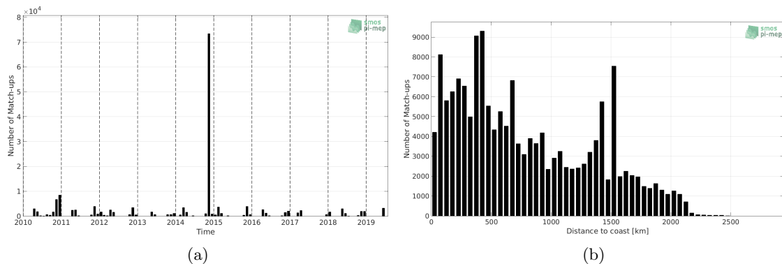
Figure 1: Number of match-ups between TSG-POLARSTERN and SMOS-L3-CATDS-CECOS-LOCEAN-V4-18DAYS-25KM SSS as a function of time (a) and as function of the distance to coast (b) over the Atlantic Ocean Pi-MEP region and for the full satellite product period.
