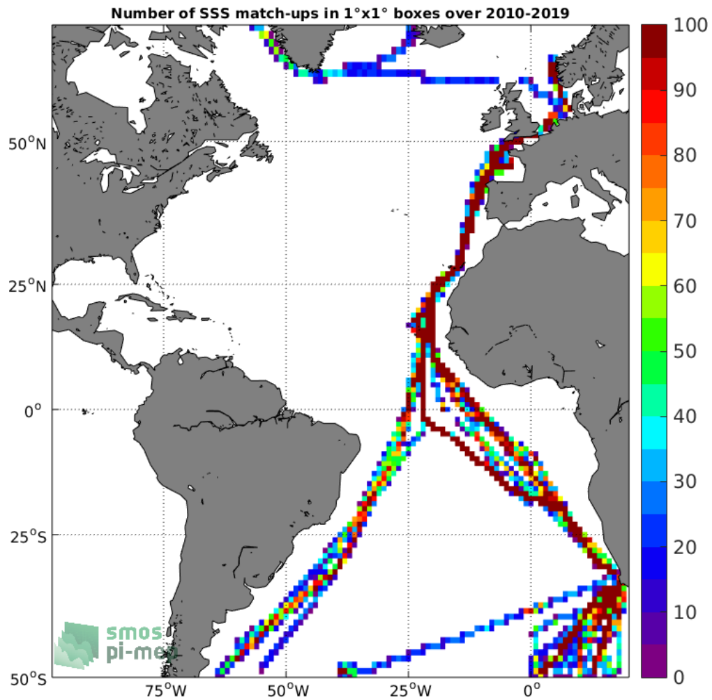
Figure 4: Number of SSS match-ups between TSG-POLARSTERN SSS and the SMOS-L3-CATDS-CECOS-LOCEAN-V4-18DAYS-25KM SSS product for the Atlantic Ocean Pi-MEP region over 1°x1° boxes and for the full satellite product period.
