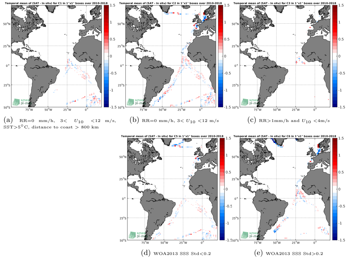
Figure 12: Temporal mean gridded over spatial boxes of size 1^\circ \times 1^\circ of \Delta SSS (SMOS-L3-CATDS-CECOS-LOCEAN-V4-18DAYS-25KM - TSG-POLARSTERN) for 5 different subdatasets corresponding to: RR=0 mm/h, 3 < U_{10} < 12 m/s, SST > 5^\circ C , distance to coast > 800 km (a), RR=0 mm/h, 3 < U_{10} < 12 m/s (b), RR > 1 mm/h and U_{10} < 4 m/s (c), WOA2013 SSS Std < 0.2 (d), WOA2013 SSS Std > 0.2 (e).
