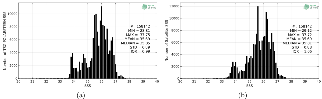
Figure 2: Histograms of SSS from TSG-POLARSTERN (a) and SMOS-L3-CATDS-CECOS-LOCEAN-V4-18DAYS-25KM (b) considering all match-up pairs per bins of 0.1 over the Atlantic Ocean Pi-MEP region and for the full satellite product period.
