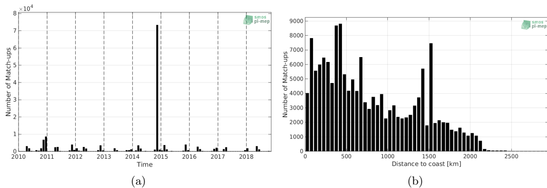
Figure 1: Number of match-ups between TSG-POLARSTERN and SMOS-L3-CATDS-CECOS-LOCEAN-V4-18DAYS-25KM SSS as a function of time (a) and as function of the distance to coast (b) over the Atlantic Ocean Pi-MEP region and for the full satellite product period.
