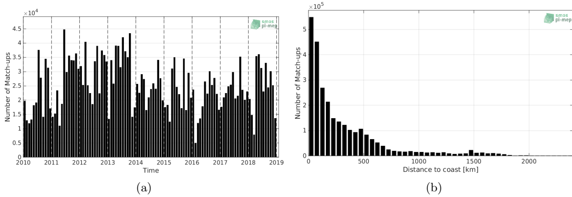
Figure 1: Number of match-ups between TSG-LEGOS-DM and SMOS-L3-CATDS-CECOS-LOCEAN-V4-18DAYS-25KM SSS as a function of time (a) and as function of the distance to coast (b) over the Atlantic Ocean Pi-MEP region and for the full satellite product period.
