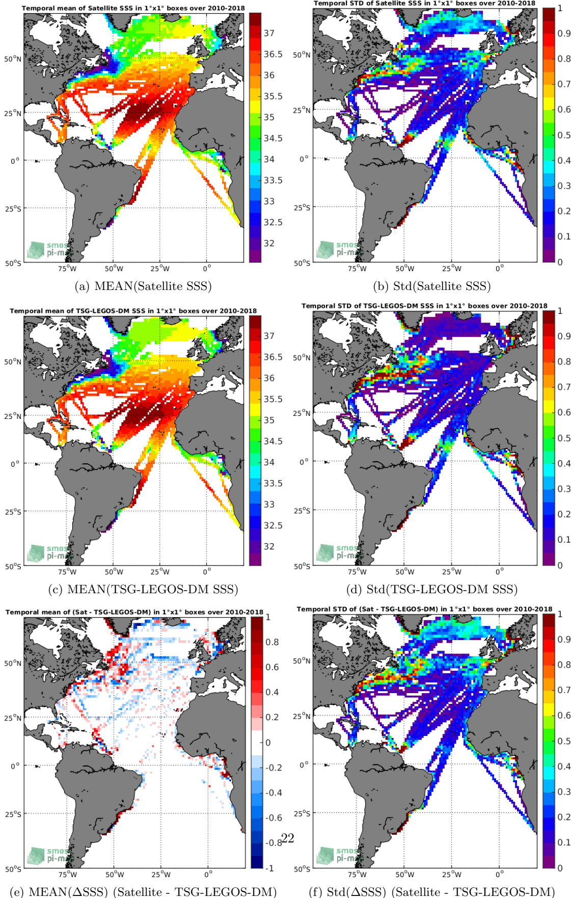
Figure 6: Temporal mean (left) and Std (right) of SSS from SMOS-L3-CATDS-CECOS-LOCEAN-V4-18DAYS-25KM (top), TSG-LEGOS-DM (middle), and of ΔSSS (Satellite - TSG-LEGOS-DM). Only match-up pairs are used to generate these maps.
