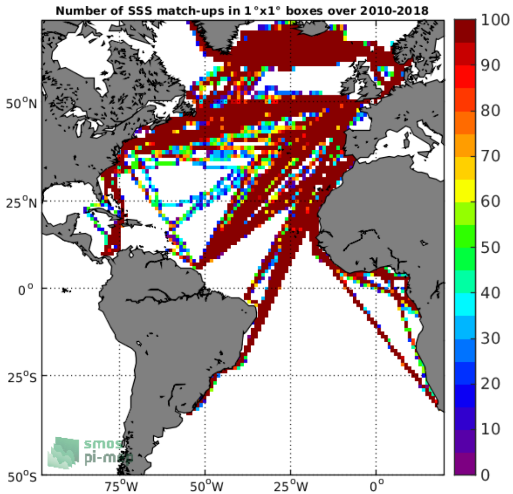
Figure 4: Number of SSS match-ups between TSG-LEGOS-DM SSS and the SMOS-L3-CATDS-CECOS-LOCEAN-V4-18DAYS-25KM SSS product for the Atlantic Ocean Pi-MEP region over 1^\circ \times 1^\circ boxes and for the full satellite product period.
