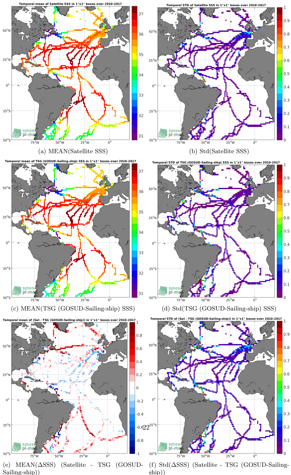
Figure 6: Temporal mean (left) and Std (right) of SSS from SMOS SSS L3 v4 - 18 Days (CATDS-CECOS-LOCEAN) (top), TSG (GOSUD-Sailing-ship) (middle), and of \Delta SSS (Satellite - TSG (GOSUD-Sailing-ship)). Only match-up pairs are used to generate these maps.
