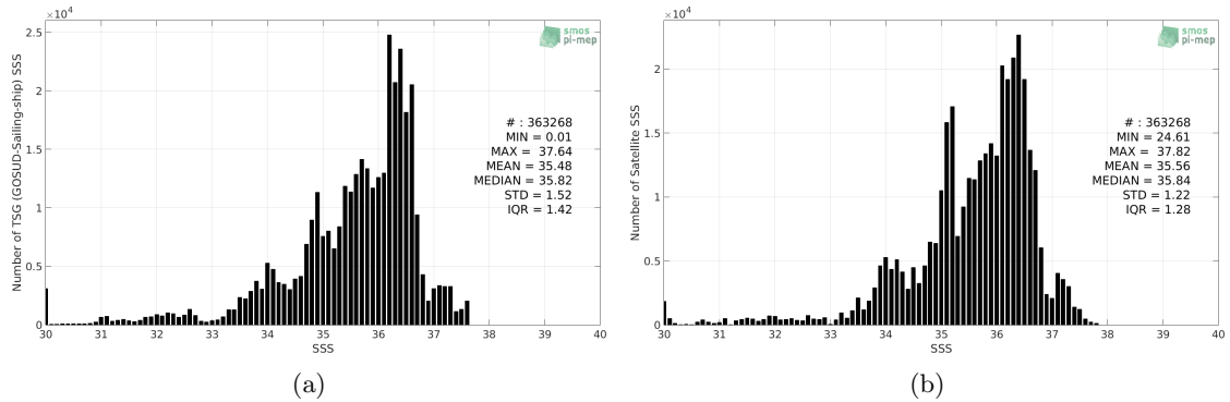
Figure 2: Histograms of SSS from TSG (GOSUD-Sailing-ship) (a) and SMOS SSS L3 v4 - 18 Days (CATDS-CECOS-LOCEAN) (b) considering all match-up pairs per bins of 0.1 over the Atlantic Ocean Pi-MEP region and for the full satellite product period.
