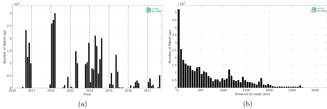
Figure 1: Number of match-ups between TSG (GOSUD-Sailing-ship) and SMOS SSS L3 v4 - 18 Days (CATDS-CECOS-LOCEAN) SSS as a function of time (a) and as function of the distance to coast (b) over the Atlantic Ocean Pi-MEP region and for the full satellite product period.
