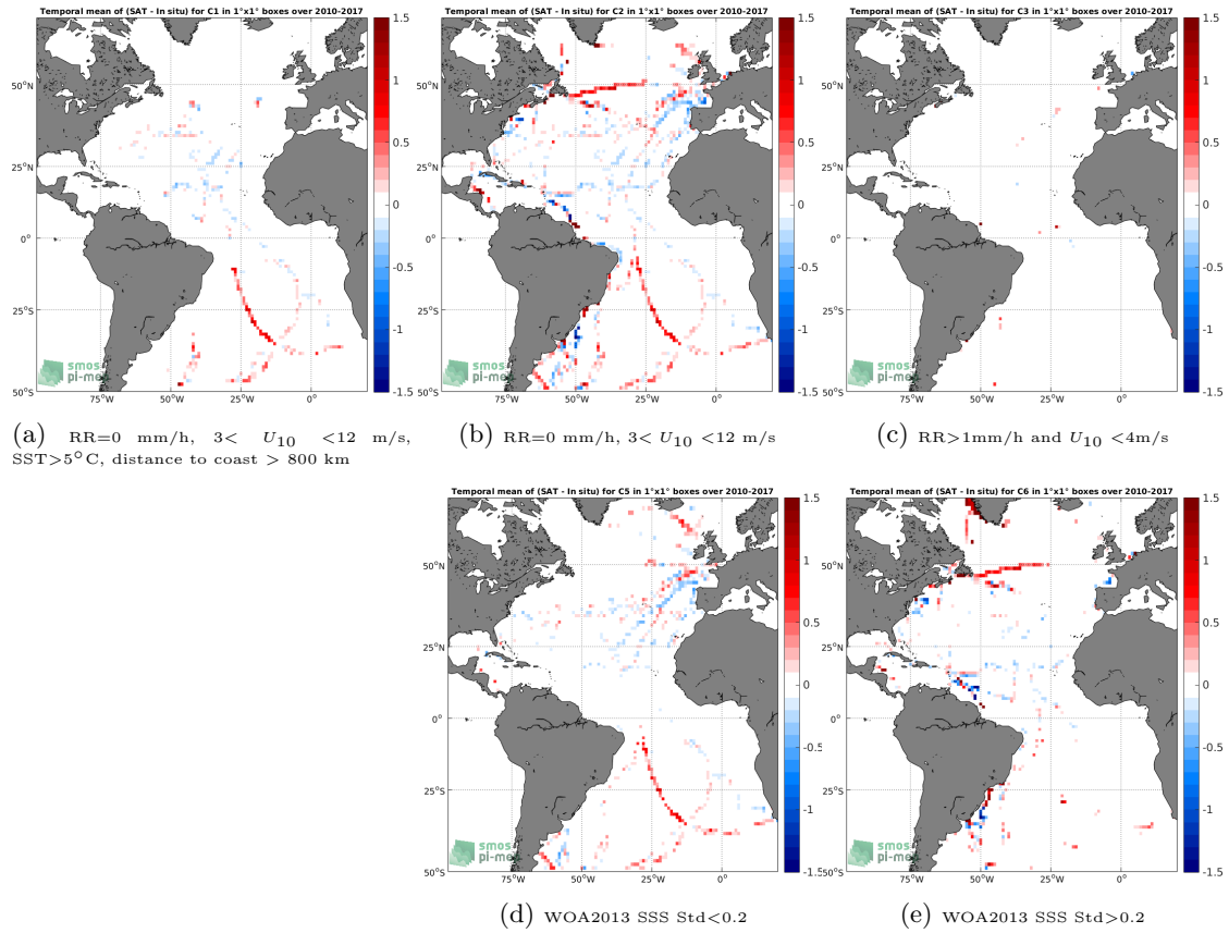
Figure 12: Temporal mean gridded over spatial boxes of size 1^\circ \times 1^\circ of \Delta\text{SSS} (SMOS SSS L3 v4 - 18 Days (CATDS-CECOS-LOCEAN) - TSG (GOSUD-Sailing-ship)) for 5 different subdatasets corresponding to:RR=0 mm/h, 3 < U_{10} < 12 m/s, SST>5°C, distance to coast > 800 km (a), RR=0 mm/h, 3 < U_{10} < 12 m/s (b), RR>1mm/h and U_{10} < 4 m/s (c), WOA2013 SSS Std<0.2 (d), WOA2013 SSS Std>0.2 (e).
