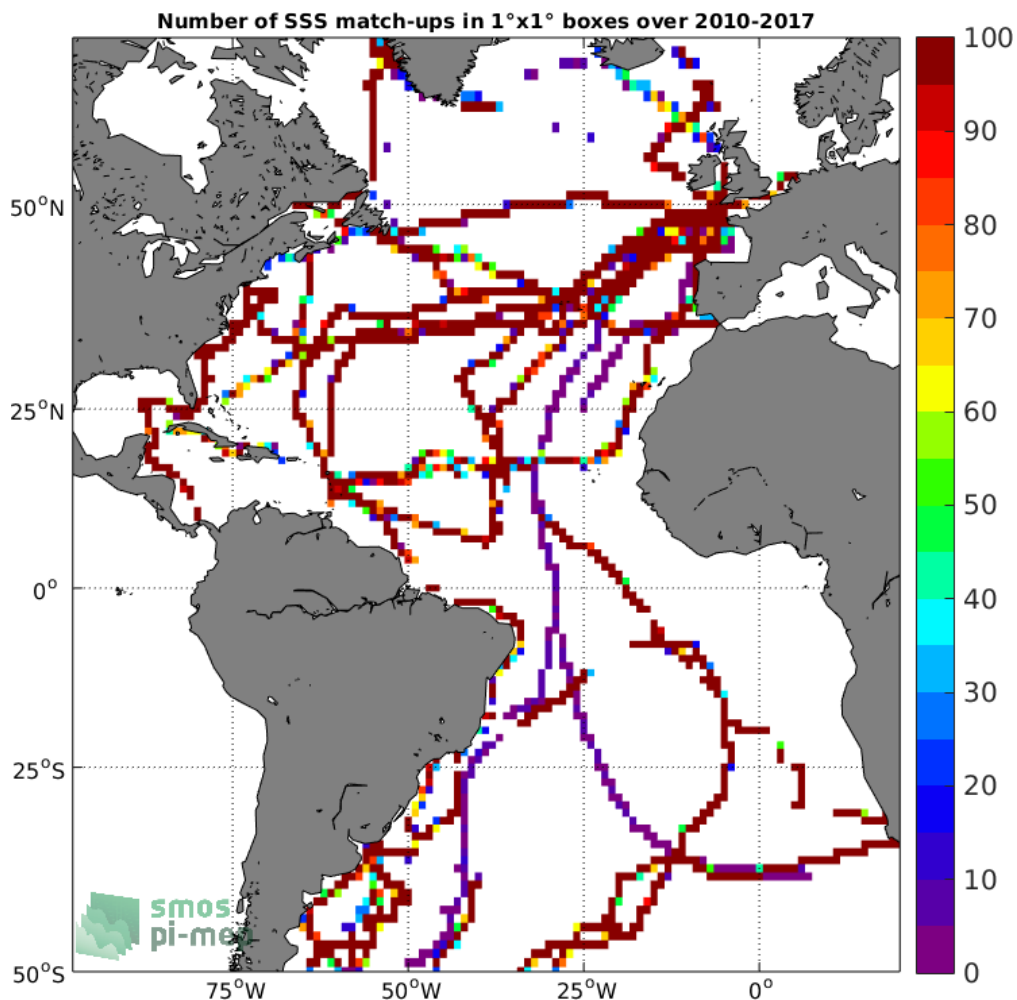
Figure 4: Number of SSS match-ups between TSG (GOSUD-Sailing-ship) SSS and the SMOS SSS L3 v4 - 18 Days (CATDS-CECOS-LOCEAN) SSS product for the Atlantic Ocean Pi-MEP region over 1°x1° boxes and for the full satellite product period.
