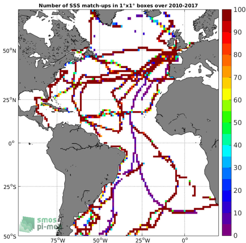
Figure 4: Number of SSS match-ups between TSG-GOSUD-Sailing-ship SSS and the SMOS-L3-CATDS-CECOS-LOCEAN-V4-18DAYS-25KM SSS product for the Atlantic Ocean Pi-MEP region over 1°x1° boxes and for the full satellite product period.
