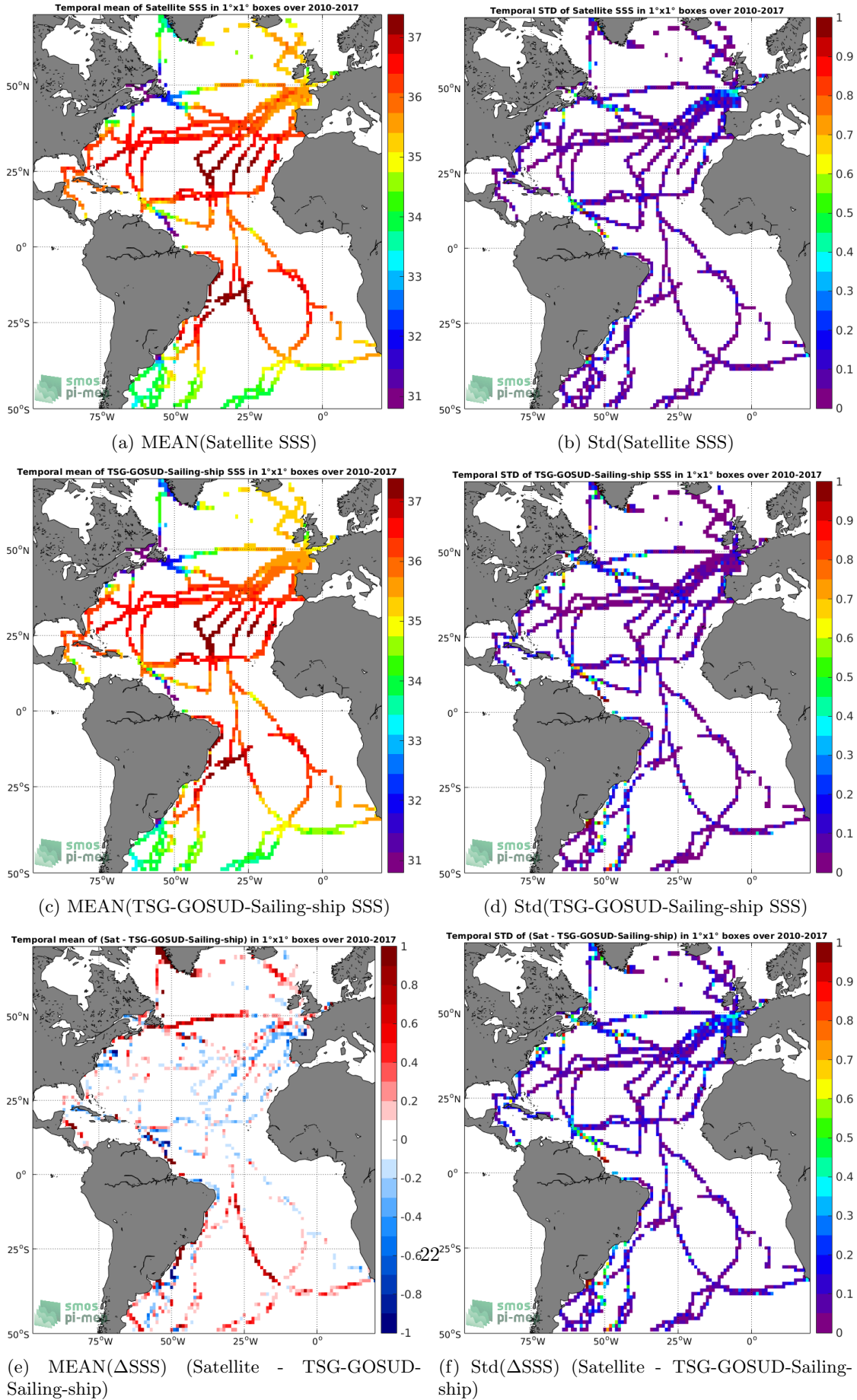
Figure 6: Temporal mean (left) and Std (right) of SSS from SMOS-L3-CATDS-CECOS-LOCEAN-V4-18DAYS-25KM (top), TSG-GOSUD-Sailing-ship (middle), and of ΔSSS (Satellite - TSG-GOSUD-Sailing-ship). Only match-up pairs are used to generate these maps.
