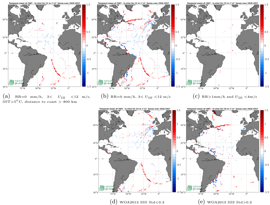
Figure 12: Temporal mean gridded over spatial boxes of size 1^\circ \times 1^\circ of \Delta\text{SSS} (SMOS-L3-CATDS-CECOS-LOCEAN-V4-18DAYS-25KM - TSG-GOSUD-Sailing-ship) for 5 different subdatasets corresponding to:RR=0 mm/h, 3 < U_{10} < 12 m/s, SST>5°C, distance to coast > 800 km (a), RR=0 mm/h, 3 < U_{10} < 12 m/s (b), RR>1mm/h and U_{10} < 4 m/s (c), WOA2013 SSS Std<0.2 (d), WOA2013 SSS Std>0.2 (e).
