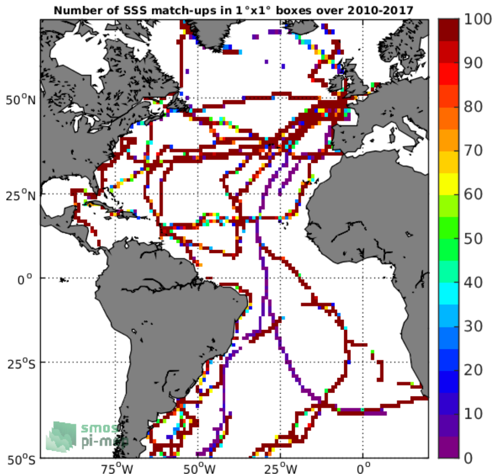
Figure 4: Number of SSS match-ups between TSG-GOSUD-Sailing-ship SSS and the SMOS-L3-CATDS-CECOS-LOCEAN-V4-18DAYS-25KM SSS product for the Atlantic Ocean Pi-MEP region over 1°x1° boxes and for the full satellite product period.
