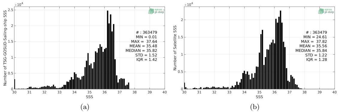
Figure 2: Histograms of SSS from TSG-GOSUD-Sailing-ship (a) and SMOS-L3-CATDS-CECOS-LOCEAN-V4-18DAYS-25KM (b) considering all match-up pairs per bins of 0.1 over the Atlantic Ocean Pi-MEP region and for the full satellite product period.
