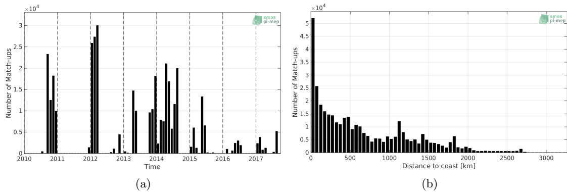
Figure 1: Number of match-ups between TSG-GOSUD-Sailing-ship and SMOS-L3-CATDS-CECOS-LOCEAN-V4-18DAYS-25KM SSS as a function of time (a) and as function of the distance to coast (b) over the Atlantic Ocean Pi-MEP region and for the full satellite product period.
