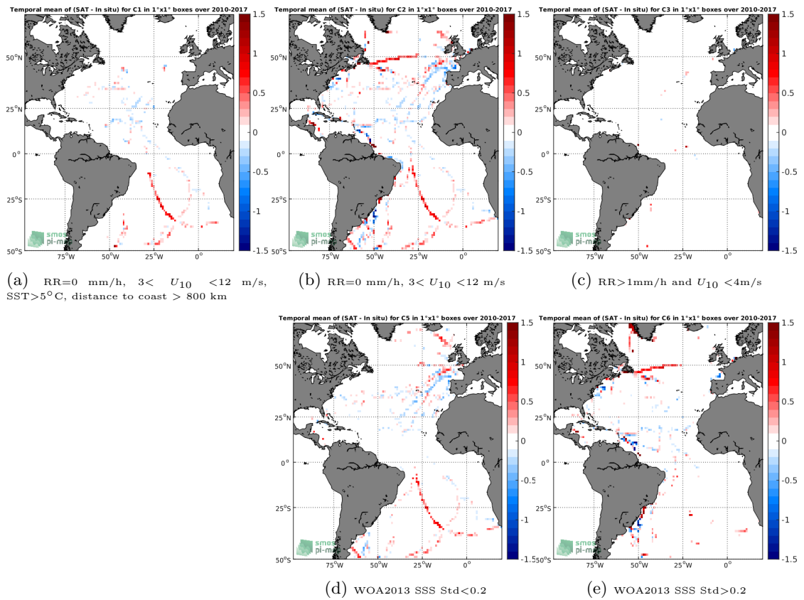
Figure 12: Temporal mean gridded over spatial boxes of size 1^\circ \times 1^\circ of \Delta SSS (SMOS-L3-CATDS-CECOS-LOCEAN-V4-18DAYS-25KM - TSG-GOSUD-Sailing-ship) for 5 different subdatasets corresponding to:RR=0 mm/h, 3 < U_{10} < 12 m/s, SST>5°C, distance to coast > 800 km (a), RR=0 mm/h, 3 < U_{10} < 12 m/s (b), RR>1mm/h and U_{10} < 4 m/s (c), WOA2013 SSS Std<0.2 (d), WOA2013 SSS Std>0.2 (e).
