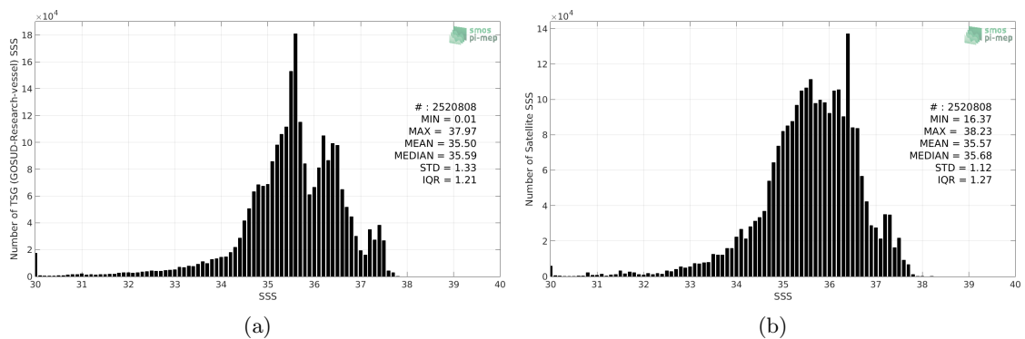
Figure 2: Histograms of SSS from TSG (GOSUD-Research-vessel) (a) and SMOS SSS L3 v4 - 18 Days (CATDS-CECOS-LOCEAN) (b) considering all match-up pairs per bins of 0.1 over the Atlantic Ocean Pi-MEP region and for the full satellite product period.
