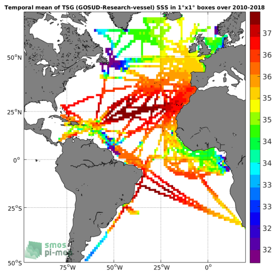
(c) MEAN(TSG (GOSUD-Research-vessel) SSS)
