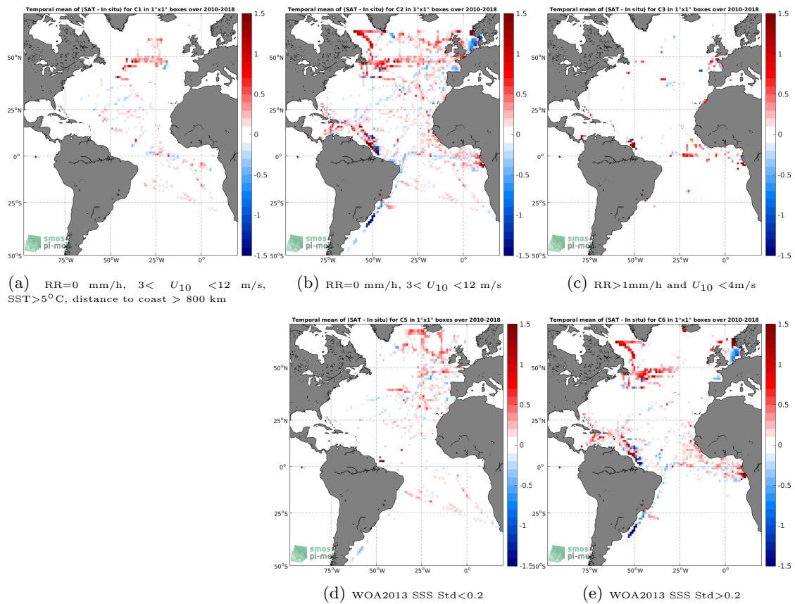
Figure 12: Temporal mean gridded over spatial boxes of size 1^\circ \times 1^\circ of \Delta\text{SSS} (SMOS SSS L3 v4 - 18 Days (CATDS-CECOS-LOCEAN) - TSG (GOSUD-Research-vessel)) for 5 different subdatasets corresponding to:RR=0 mm/h, 3 < U_{10} < 12 m/s, SST>5°C, distance to coast > 800 km (a), RR=0 mm/h, 3 < U_{10} < 12 m/s (b), RR>1mm/h and U_{10} < 4 m/s (c), WOA2013 SSS Std<0.2 (d), WOA2013 SSS Std>0.2 (e).
