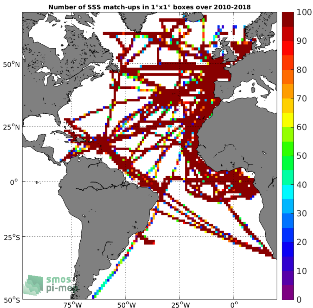
Figure 4: Number of SSS match-ups between TSG (GOSUD-Research-vessel) SSS and the SMOS SSS L3 v4 - 18 Days (CATDS-CECOS-LOCEAN) SSS product for the Atlantic Ocean Pi-MEP region over 1°x1° boxes and for the full satellite product period.
