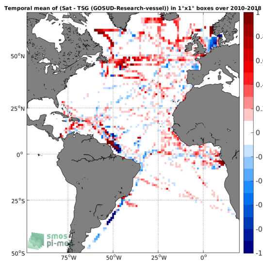
(e) MEAN( \Delta SSS) (Satellite - TSG (GOSUD-Research-vessel))
