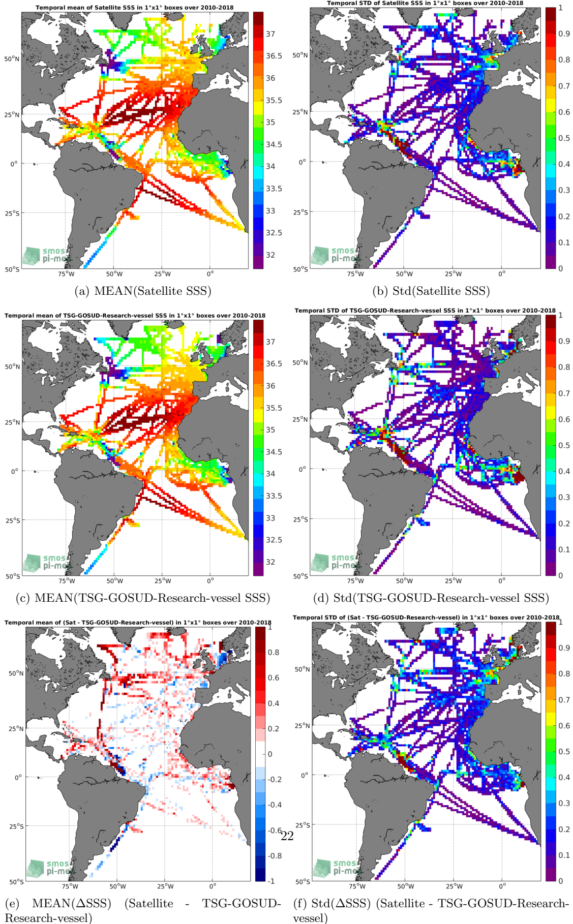
Figure 6: Temporal mean (left) and Std (right) of SSS from SMOS-L3-CATDS-CECOS-LOCEAN-V4-18DAYS-25KM (top), TSG-GOSUD-Research-vessel (middle), and of \Delta SSS (Satellite - TSG-GOSUD-Research-vessel). Only match-up pairs are used to generate these maps.
