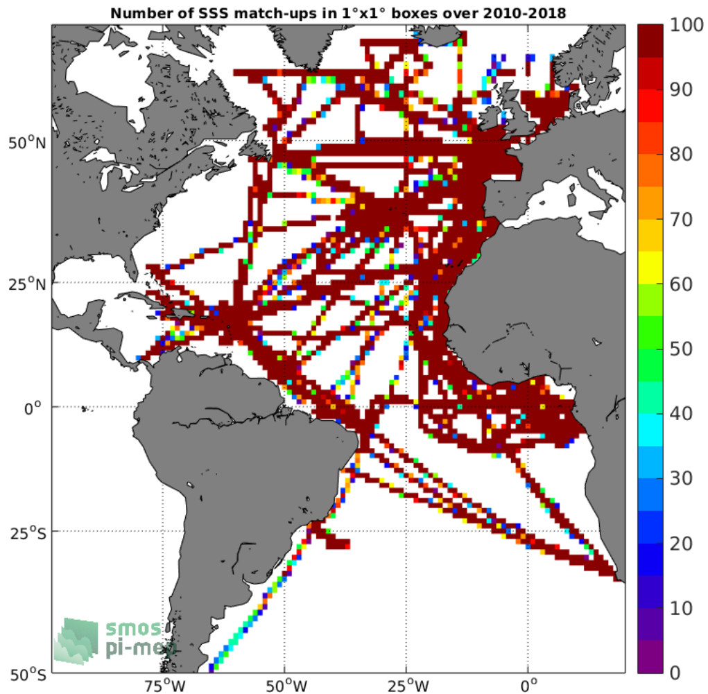
Figure 4: Number of SSS match-ups between TSG-GOSUD-Research-vessel SSS and the SMOS-L3-CATDS-CECOS-LOCEAN-V4-18DAYS-25KM SSS product for the Atlantic Ocean Pi-MEP region over 1°x1° boxes and for the full satellite product period.
