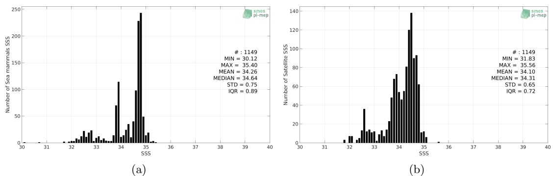
Figure 2: Histograms of SSS from Sea mammals (a) and SMOS SSS L3 v4 - 18 Days (CATDS-CECOS-LOCEAN) (b) considering all match-up pairs per bins of 0.1 over the Atlantic Ocean Pi-MEP region and for the full satellite product period.
