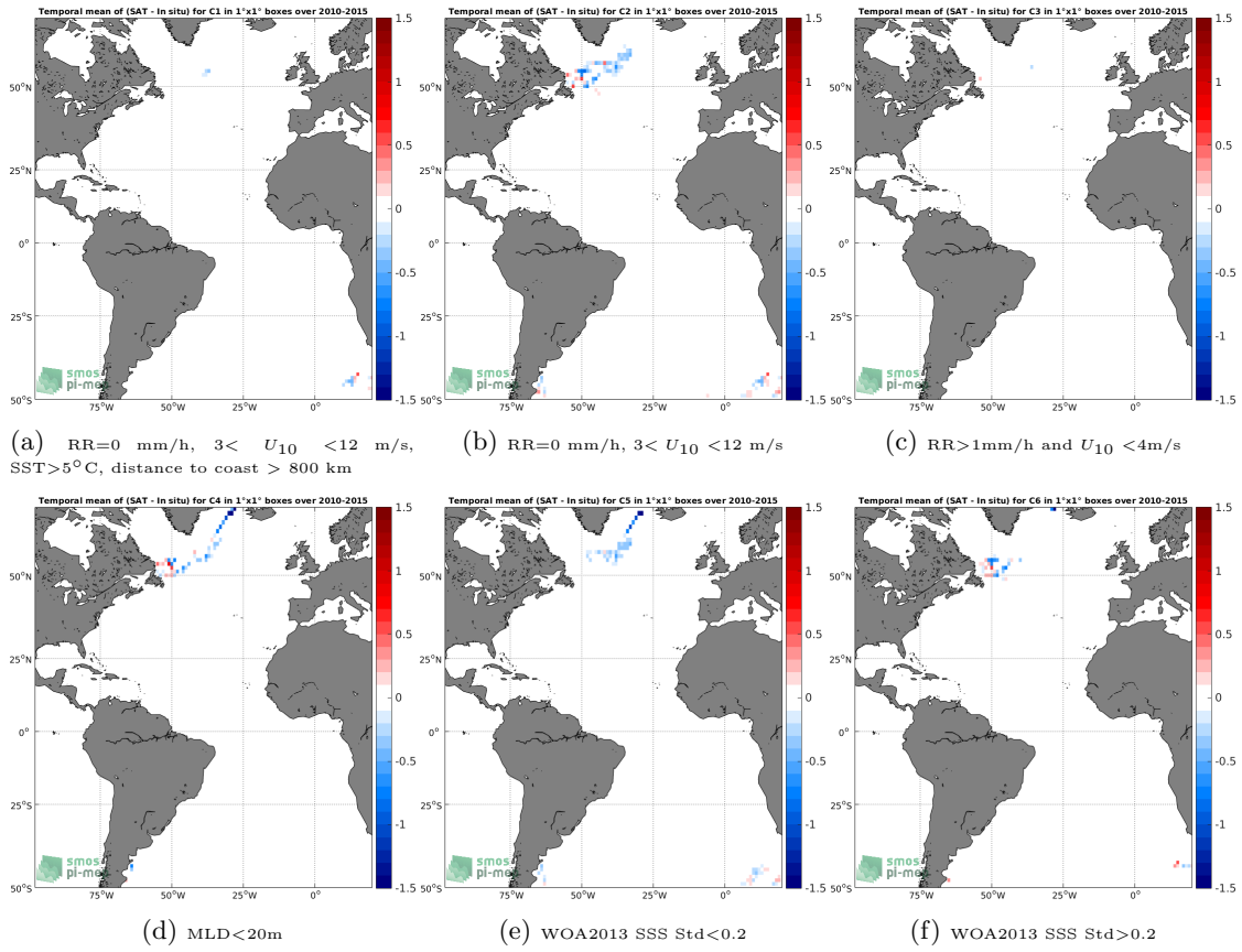
Figure 12: Temporal mean gridded over spatial boxes of size 1^\circ \times 1^\circ of \Delta SSS (SMOS SSS L3 v4 - 18 Days (CATDS-CECOS-LOCEAN) - Sea mammals) for 6 different subdatasets corresponding to:RR=0 mm/h, 3 < U_{10} < 12 m/s, SST>5°C, distance to coast > 800 km (a), RR=0 mm/h, 3 < U_{10} < 12 m/s (b), RR>1mm/h and U_{10} < 4 m/s (c),MLD<20m (d),WOA2013 SSS Std<0.2 (e),WOA2013 SSS Std>0.2 (f).
