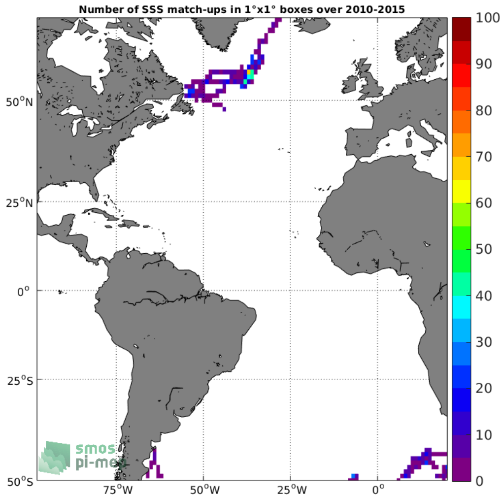
Figure 4: Number of SSS match-ups between Sea mammals SSS and the SMOS SSS L3 v4 - 18 Days (CATDS-CECOS-LOCEAN) SSS product for the Atlantic Ocean Pi-MEP region over 1°x1° boxes and for the full satellite product period.
