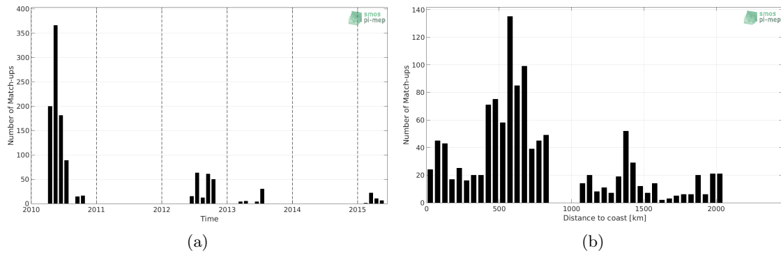
Figure 1: Number of match-ups between Sea mammals and SMOS SSS L3 v4 - 18 Days (CATDS-CECOS-LOCEAN) SSS as a function of time (a) and as function of the distance to coast (b) over the Atlantic Ocean Pi-MEP region and for the full satellite product period.
