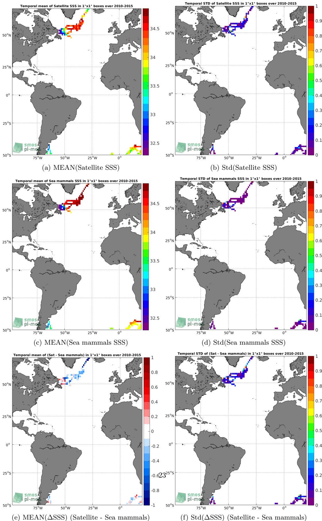
Figure 6: Temporal mean (left) and Std (right) of SSS from SMOS SSS L3 v4 - 18 Days (CATDS-CECOS-LOCEAN) (top), Sea mammals (middle), and of \Delta SSS (Satellite - Sea mammals). Only match-up pairs are used to generate these maps.
