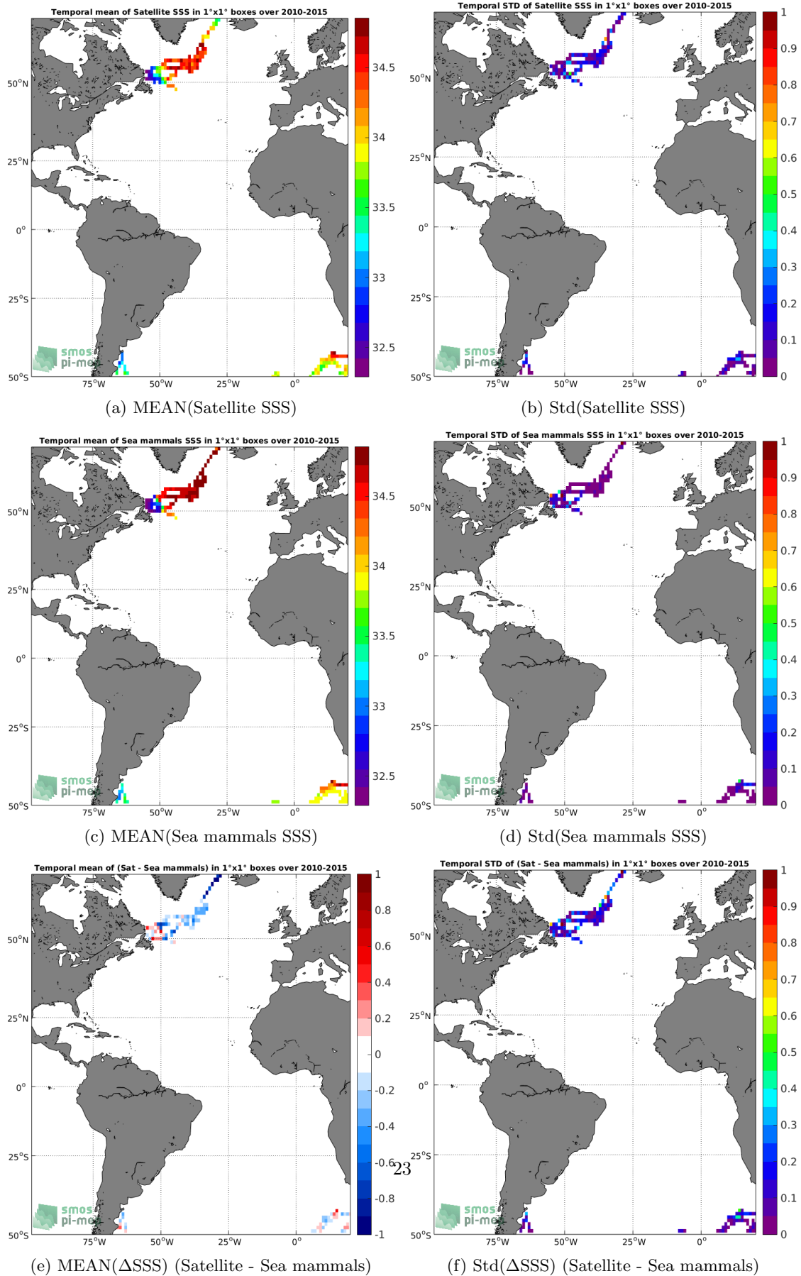
Figure 6: Temporal mean (left) and Std (right) of SSS from SMOS-L3-CATDS-CECOS-LOCEAN-V4-18DAYS-25KM (top), Sea mammals (middle), and of \Delta SSS (Satellite - Sea mammals). Only match-up pairs are used to generate these maps.
