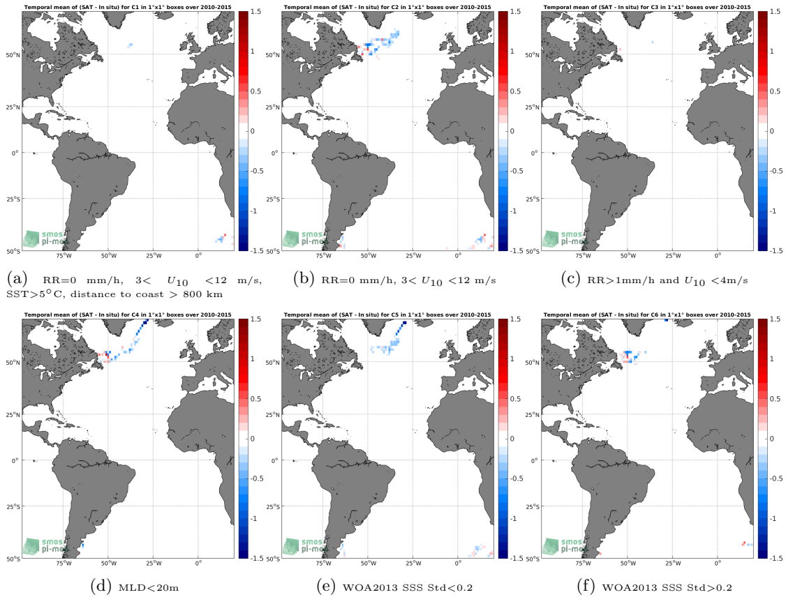
Figure 12: Temporal mean gridded over spatial boxes of size 1^\circ \times 1^\circ of \Delta SSS (SMOS-L3-CATDS-CECOS-LOCEAN-V4-18DAYS-25KM - Sea mammals) for 6 different subdatasets corresponding to: RR=0 mm/h, 3 < U_{10} < 12 m/s, SST>5°C, distance to coast > 800 km (a), RR=0 mm/h, 3 < U_{10} < 12 m/s (b), RR>1mm/h and U_{10} < 4 m/s (c),MLD<20m (d),WOA2013 SSS Std<0.2 (e),WOA2013 SSS Std>0.2 (f).
