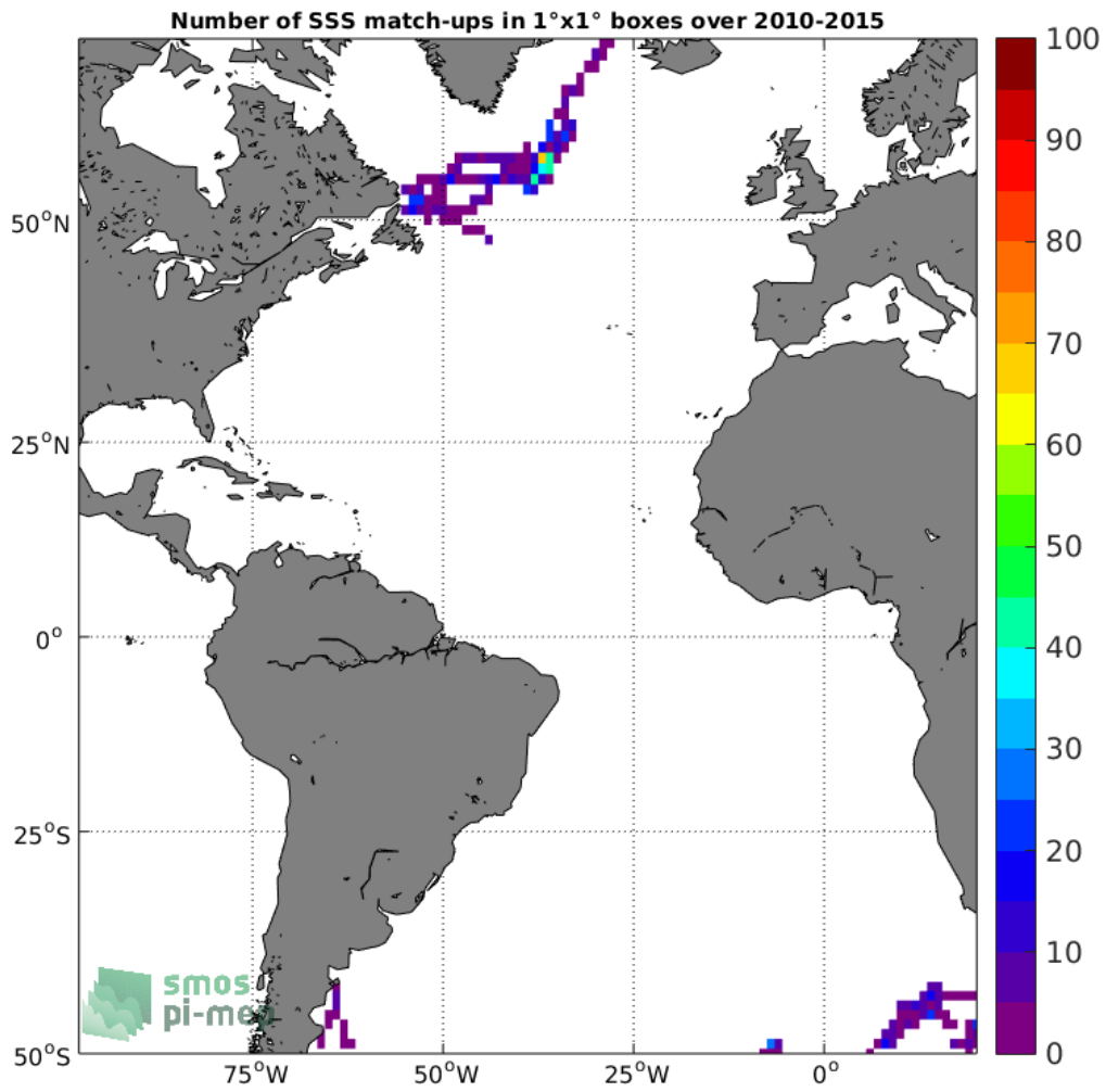
Figure 4: Number of SSS match-ups between Sea mammals SSS and the SMOS-L3-CATDS-CECOS-LOCEAN-V4-18DAYS-25KM SSS product for the Atlantic Ocean Pi-MEP region over 1°x1° boxes and for the full satellite product period.
