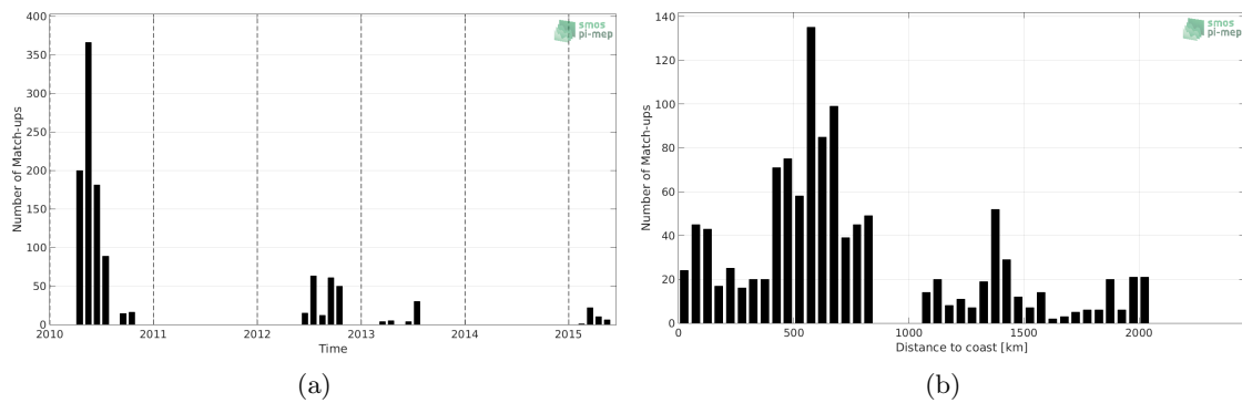
Figure 1: Number of match-ups between Sea mammals and SMOS-L3-CATDS-CECOS-LOCEAN-V4-18DAYS-25KM SSS as a function of time (a) and as function of the distance to coast (b) over the Atlantic Ocean Pi-MEP region and for the full satellite product period.
