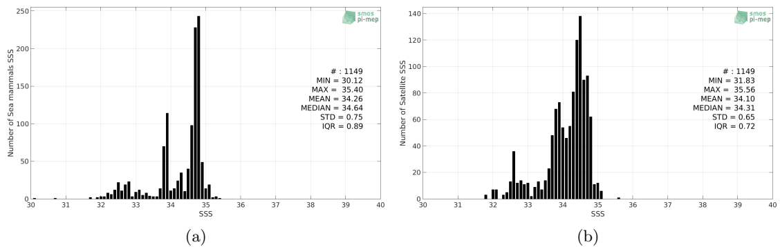
Figure 2: Histograms of SSS from Sea mammals (a) and SMOS-L3-CATDS-CECOS-LOCEAN-V4-18DAYS-25KM (b) considering all match-up pairs per bins of 0.1 over the Atlantic Ocean Pi-MEP region and for the full satellite product period.
