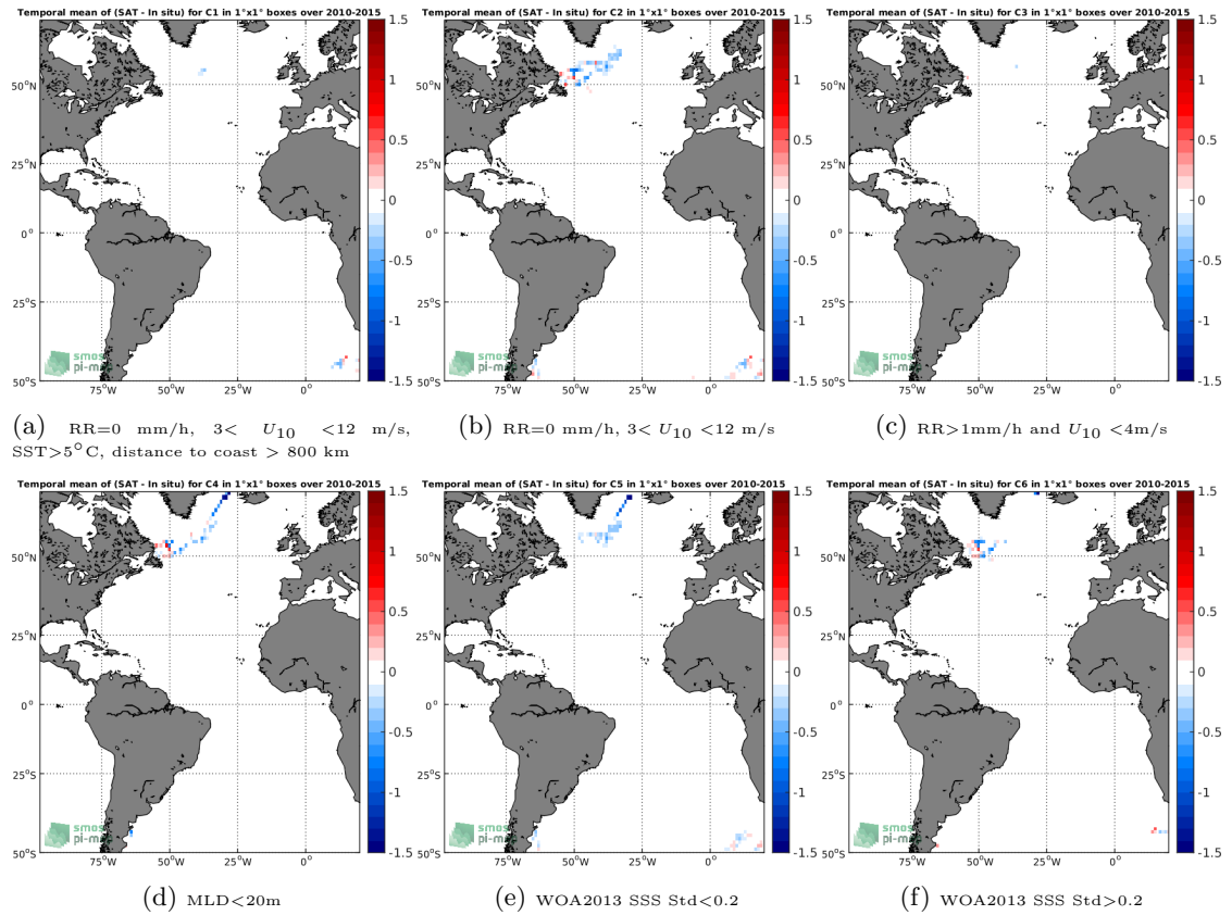
Figure 12: Temporal mean gridded over spatial boxes of size 1^\circ \times 1^\circ of \Delta SSS (SMOS-L3-CATDS-CECOS-LOCEAN-V4-18DAYS-25KM - Sea mammals) for 6 different subdatasets corresponding to:RR=0 mm/h, 3 < U_{10} < 12 m/s, SST > 5^\circ\text{C} , distance to coast > 800 km (a), RR=0 mm/h, 3 < U_{10} < 12 m/s (b), RR > 1 mm/h and U_{10} < 4 m/s (c),MLD < 20 m (d),WOA2013 SSS Std < 0.2 (e),WOA2013 SSS Std > 0.2 (f).
