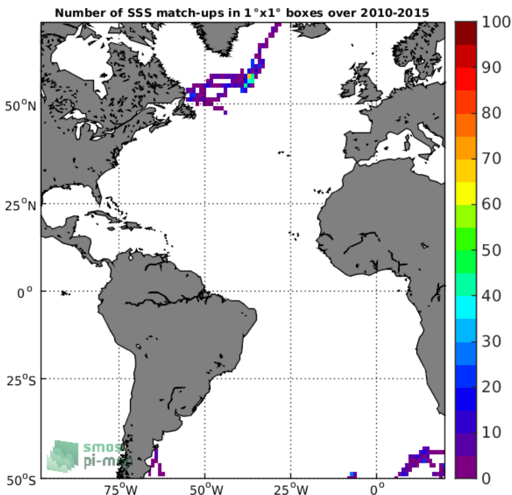
Figure 4: Number of SSS match-ups between Sea mammals SSS and the SMOS-L3-CATDS-CECOS-LOCEAN-V4-18DAYS-25KM SSS product for the Atlantic Ocean Pi-MEP region over 1°x1° boxes and for the full satellite product period.
