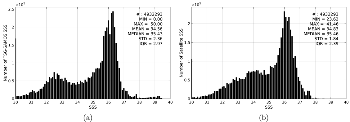
Figure 2: Histograms of SSS from TSG-SAMOS (a) and SMOS-L3-CATDS-CECOS-LOCEAN-V2-18DAYS-25KM (b) considering all match-up pairs per bins of 0.1 over the Atlantic Ocean Pi-MEP region and for the full satellite product period.
