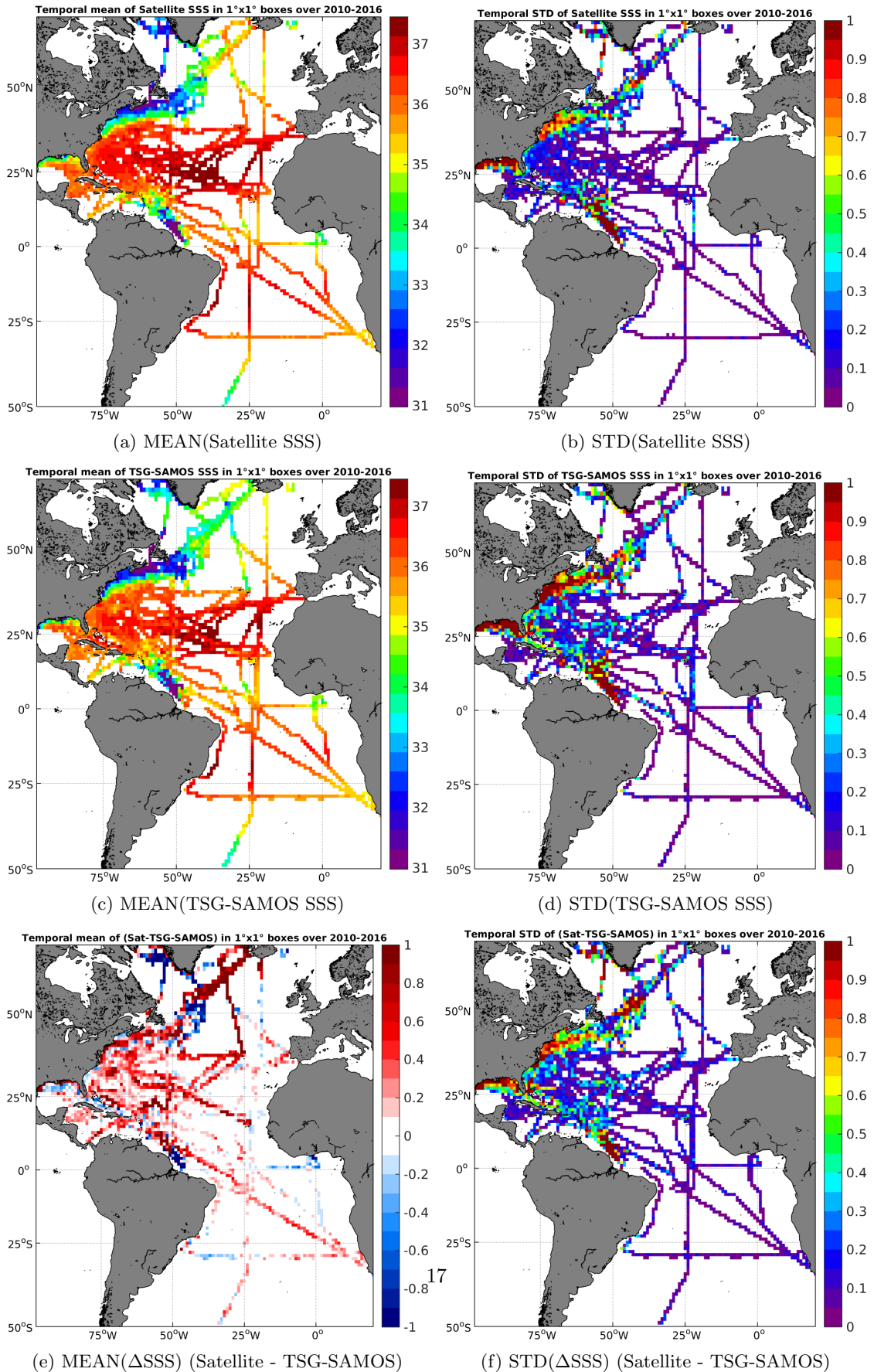
Figure 6: Temporal mean (left) and STD (right) of SSS from SMOS-L3-CATDS-CECOS-LOCEAN-V2-18DAYS-25KM (top), TSG-SAMOS (middle), and of \Delta SSS (Satellite - TSG-SAMOS). Only match-up pairs are used to generate these maps.
