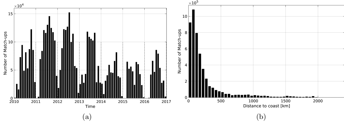
Figure 1: Number of match-ups between TSG-SAMOS and SMOS-L3-CATDS-CECOS-LOCEAN-V2-18DAYS-25KM SSS as a function of time (a) and as function of the distance to coast (b) over the Atlantic Ocean Pi-MEP region and for the full satellite product period.
