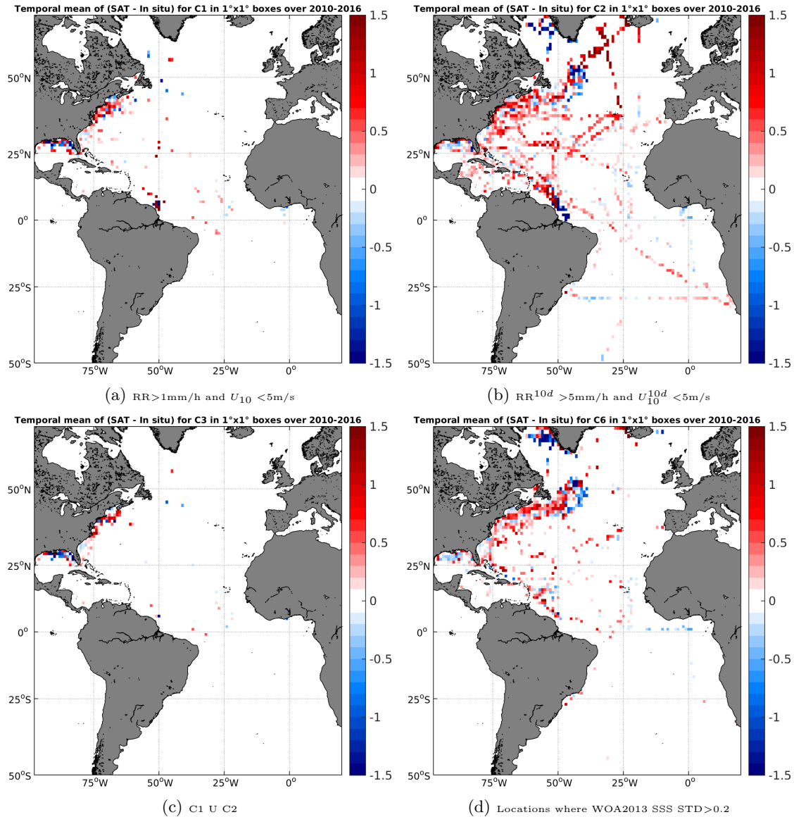
Figure 12: Temporal mean gridded over spatial boxes of size 1^\circ \times 1^\circ of \Delta SSS (SMOS-L3-CATDS-CECOS-LOCEAN-V2-18DAYS-25KM - TSG-SAMOS) for 4 different subdatasets corresponding to:RR >1 mm/h and U_{10} < 5 m/s (a), RR 10d > 5 mm/h and U_{10}^{10d} < 5 m/s (b), C1 U C2 (c),Locations where WOA2013 SSS STD >0.2 (d).
