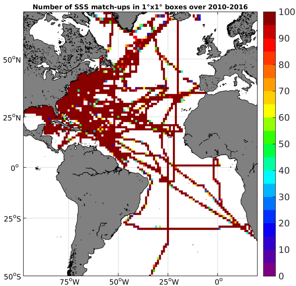
Figure 4: Number of SSS match-ups between TSG-SAMOS SSS and the SMOS-L3-CATDS-CECOS-LOCEAN-V2-18DAYS-25KM SSS product for the Atlantic Ocean Pi-MEP region over 1°x1° boxes and for the full satellite product period.
