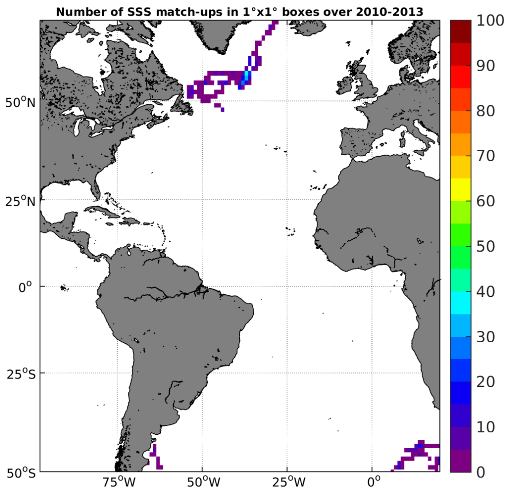
Figure 4: Number of SSS match-ups between Sea mammals SSS and the SMOS-L3-CATDS-CECOS-LOCEAN-V2-18DAYS-25KM SSS product for the Atlantic Ocean Pi-MEP region over 1°x1° boxes and for the full satellite product period.
