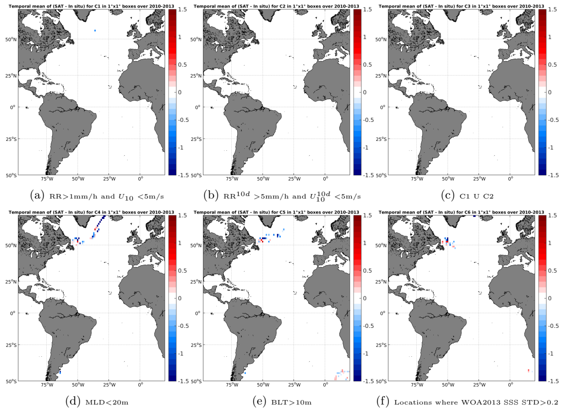
Figure 12: Temporal mean gridded over spatial boxes of size 1^\circ \times 1^\circ of \Delta SSS (SMOS-L3-CATDS-CECOS-LOCEAN-V2-18DAYS-25KM - Sea mammals) for 6 different subdatasets corresponding to:RR >1 mm/h and U_{10} < 5 m/s (a), RR 10d > 5 mm/h and U_{10}^{10d} < 5 m/s (b), C1 U C2 (c),MLD <20 m (d),BLT >10 m (e),Locations where WOA2013 SSS STD >0.2 (f).
