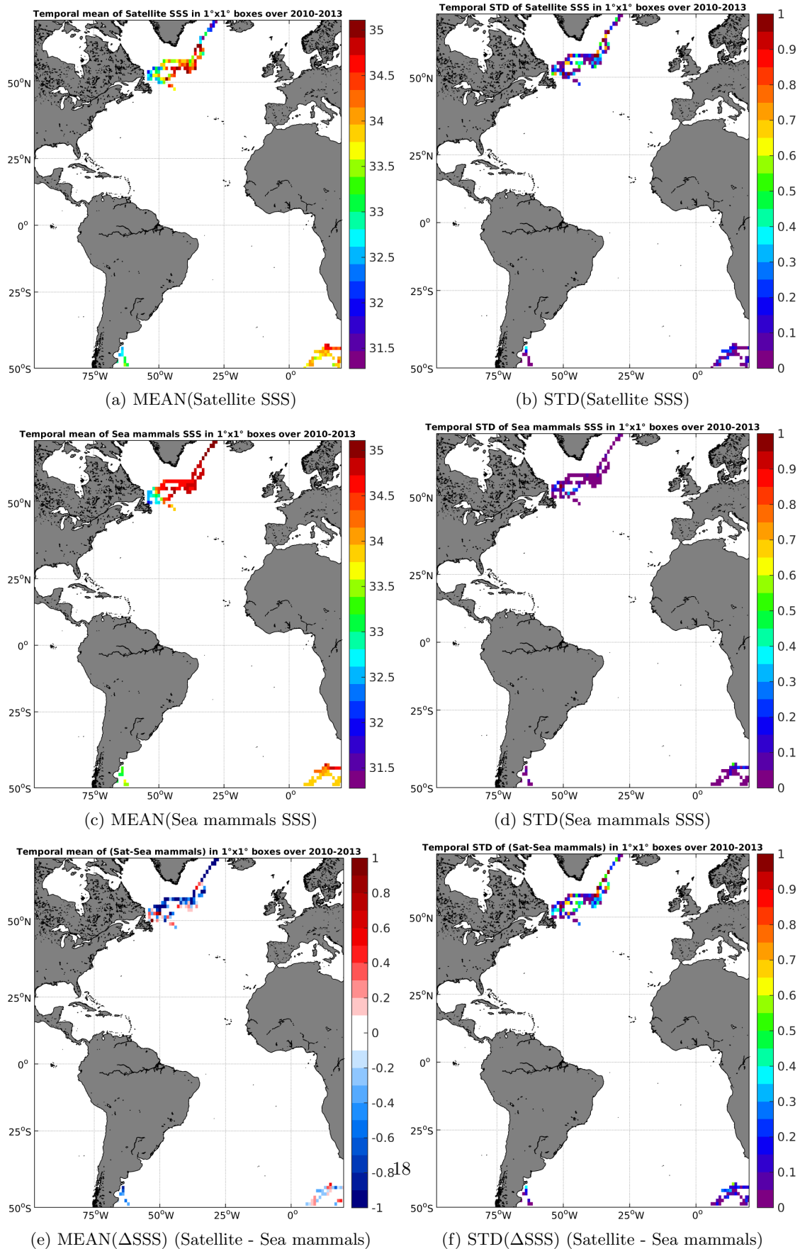
Figure 6: Temporal mean (left) and STD (right) of SSS from SMOS-L3-CATDS-CECOS-LOCEAN-V2-18DAYS-25KM (top), Sea mammals (middle), and of \Delta SSS (Satellite - Sea mammals). Only match-up pairs are used to generate these maps.
