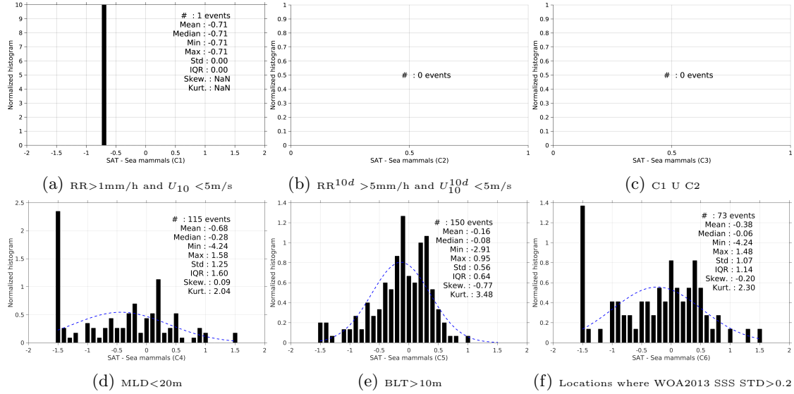
Figure 13: Normalized histogram of \Delta SSS (SMOS-L3-CATDS-CECOS-LOCEAN-V2-18DAYS-25KM - Sea mammals) for 6 different subdatasets corresponding to: RR>1mm/h and U_{10} < 5\text{m/s} (a), RR 10d >5mm/h and U_{10}^{10d} < 5\text{m/s} (b), C1 U C2 (c),MLD<20m (d),BLT>10m (e),Locations where WOA2013 SSS STD>0.2 (f).
