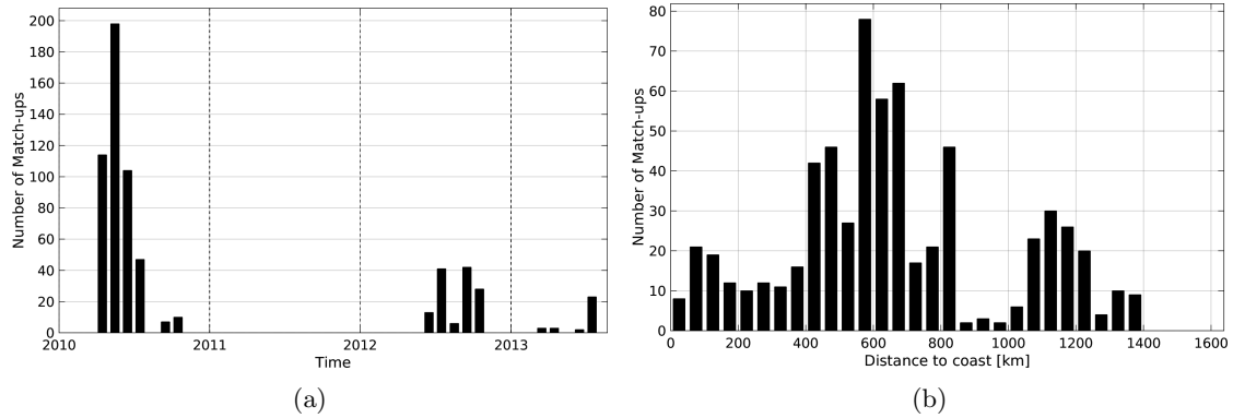
Figure 1: Number of match-ups between Sea mammals and SMOS-L3-CATDS-CECOS-LOCEAN-V2-18DAYS-25KM SSS as a function of time (a) and as function of the distance to coast (b) over the Atlantic Ocean Pi-MEP region and for the full satellite product period.
