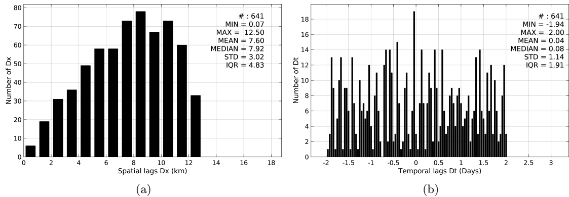
Figure 5: Histograms of the spatial (a) and temporal (b) lags between the time of the Sea mammals measurements and the date of the corresponding SMOS-L3-CATDS-CECOS-LOCEAN-V2-18DAYS-25KM SSS product.
