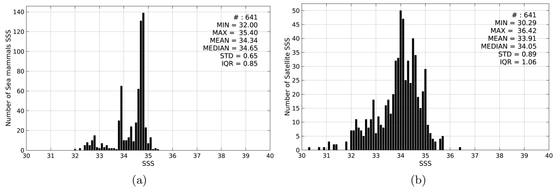
Figure 2: Histograms of SSS from Sea mammals (a) and SMOS-L3-CATDS-CECOS-LOCEAN-V2-18DAYS-25KM (b) considering all match-up pairs per bins of 0.1 over the Atlantic Ocean Pi-MEP region and for the full satellite product period.
