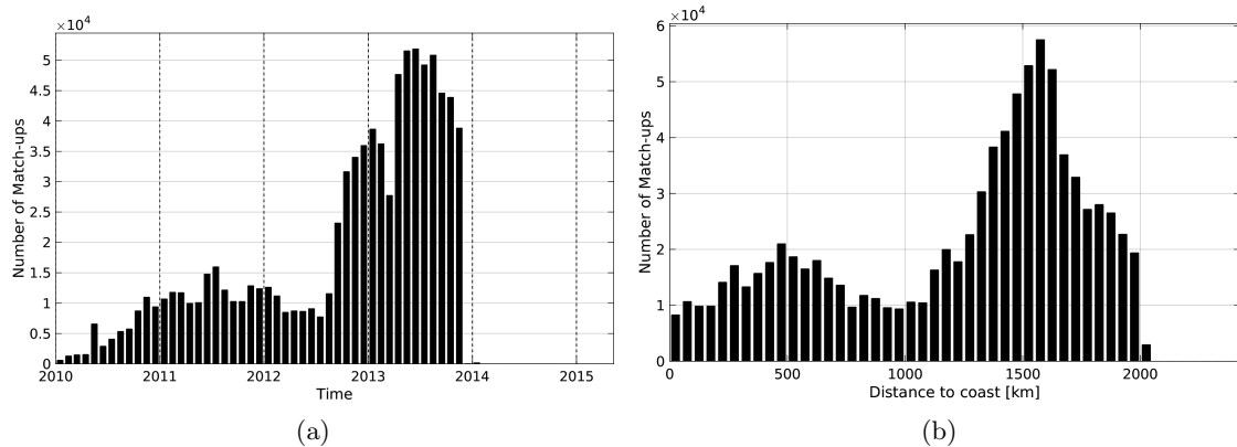
Figure 1: Number of match-ups between Surface drifters and SMOS-L3-CATDS-CECOS-LOCEAN-V2-18DAYS-25KM SSS as a function of time (a) and as function of the distance to coast (b) over the Atlantic Ocean Pi-MEP region and for the full satellite product period.
