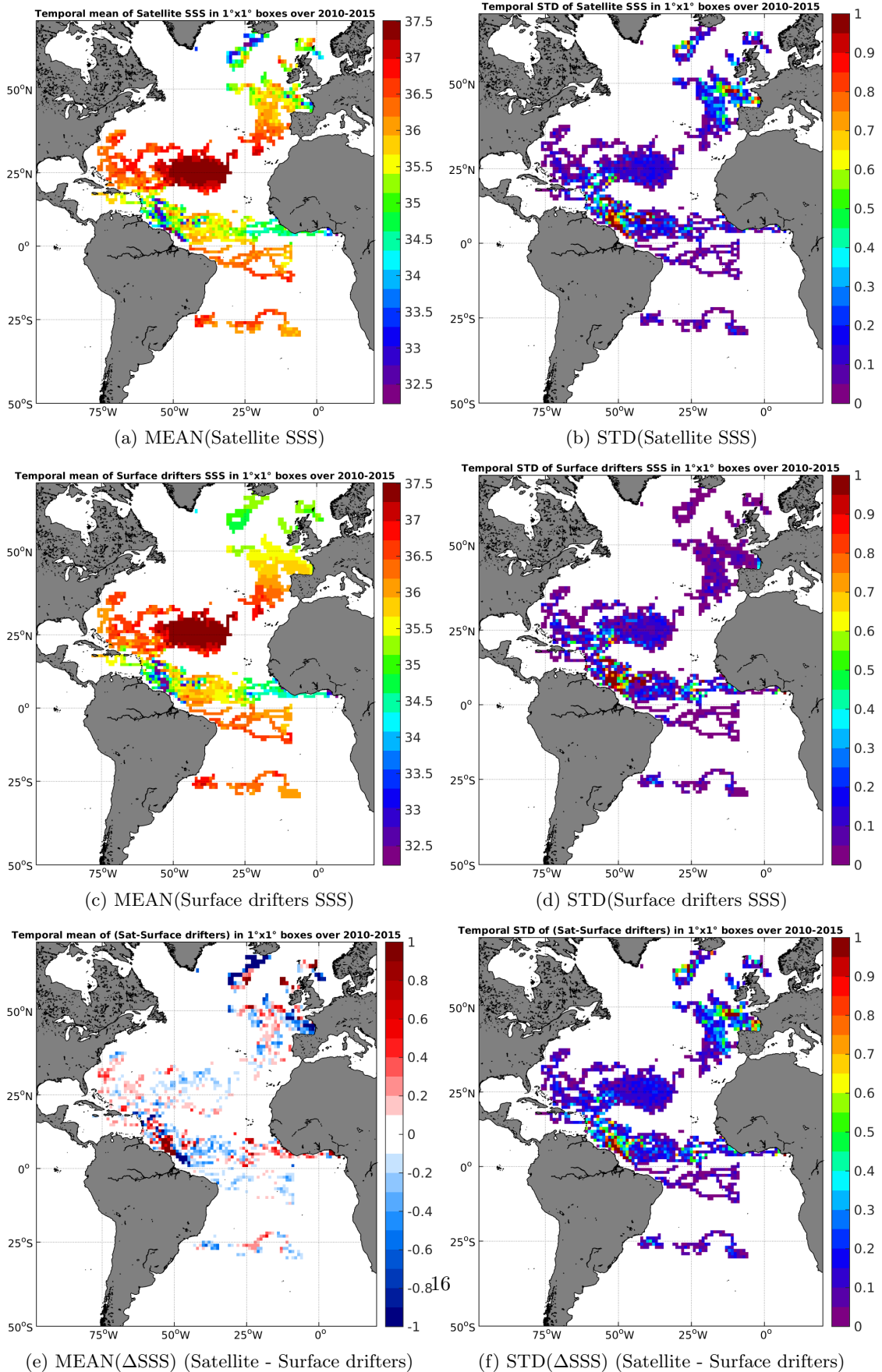
Figure 5: Temporal mean (left) and STD (right) of SSS from SMOS-L3-CATDS-CECOS-LOCEAN-V2-18DAYS-25KM (top), Surface drifters (middle), and of \Delta SSS (Satellite - Surface drifters). Only match-up pairs are used to generate these maps.
