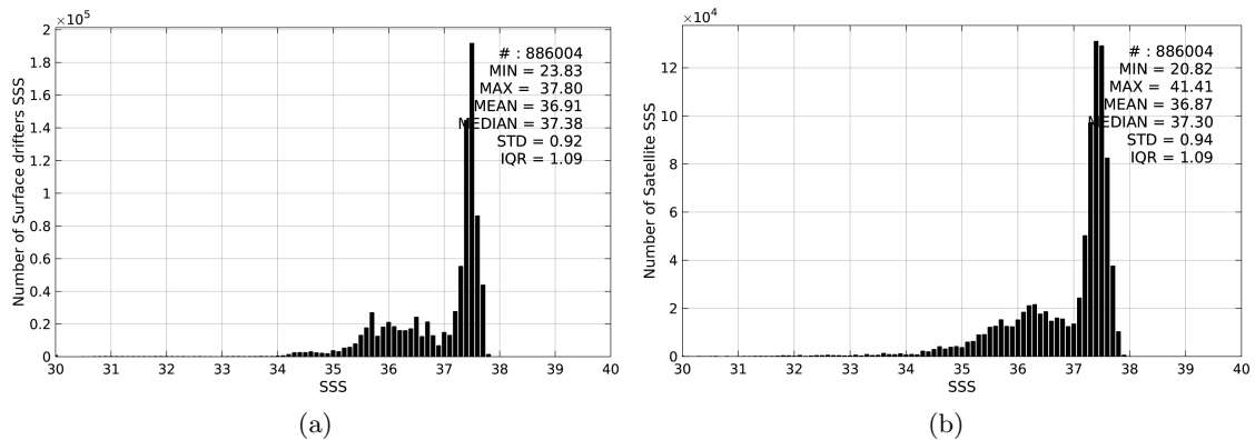
Figure 2: Histograms of SSS from Surface drifters (a) and SMOS-L3-CATDS-CECOS-LOCEAN-V2-18DAYS-25KM (b) considering all match-up pairs per bins of 0.1 over the Atlantic Ocean Pi-MEP region and for the full satellite product period.
