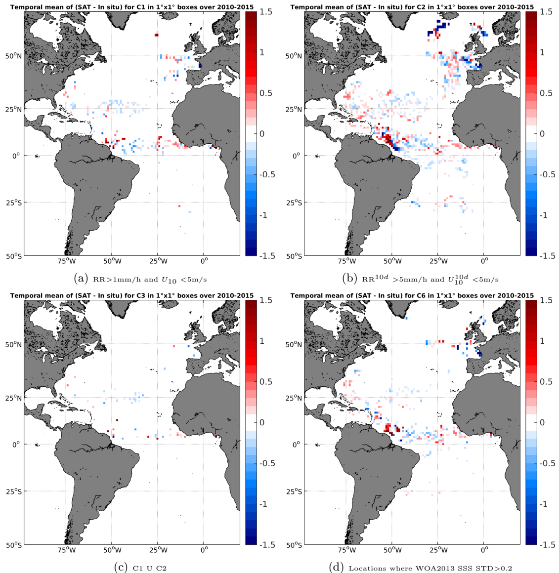
Figure 11: Temporal mean gridded over spatial boxes of size 1^\circ \times 1^\circ of \Delta SSS (SMOS-L3-CATDS-CECOS-LOCEAN-V2-18DAYS-25KM - Surface drifters) for 4 different subdatasets corresponding to:RR > 1 mm/h and U_{10} < 5 m/s (a), RR^{10d} > 5 mm/h and U_{10}^{10d} < 5 m/s (b), C1 U C2 (c),Locations where WOA2013 SSS STD > 0.2 (d).
