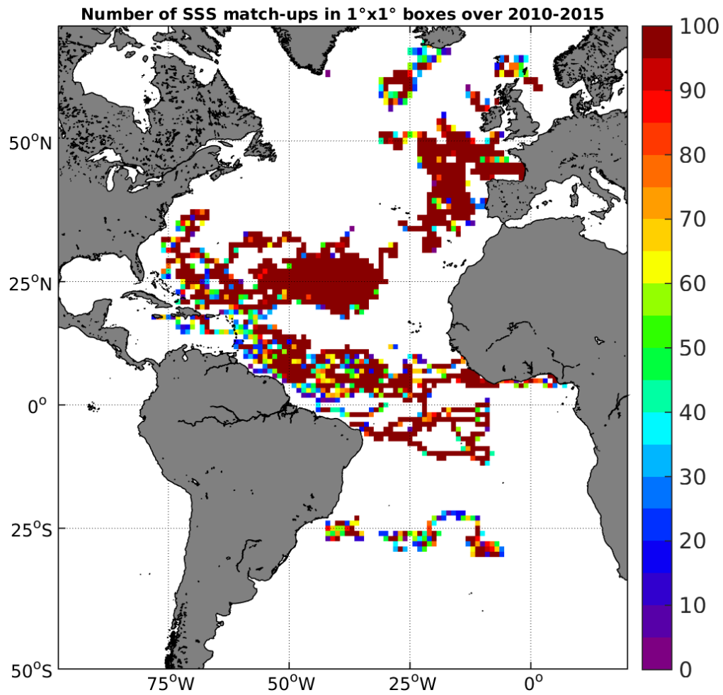
Figure 3: Number of SSS match-ups between Surface drifters SSS and the SMOS-L3-CATDS-CECOS-LOCEAN-V2-18DAYS-25KM SSS product for the Atlantic Ocean Pi-MEP region over 1°x1° boxes and for the full satellite product period.
